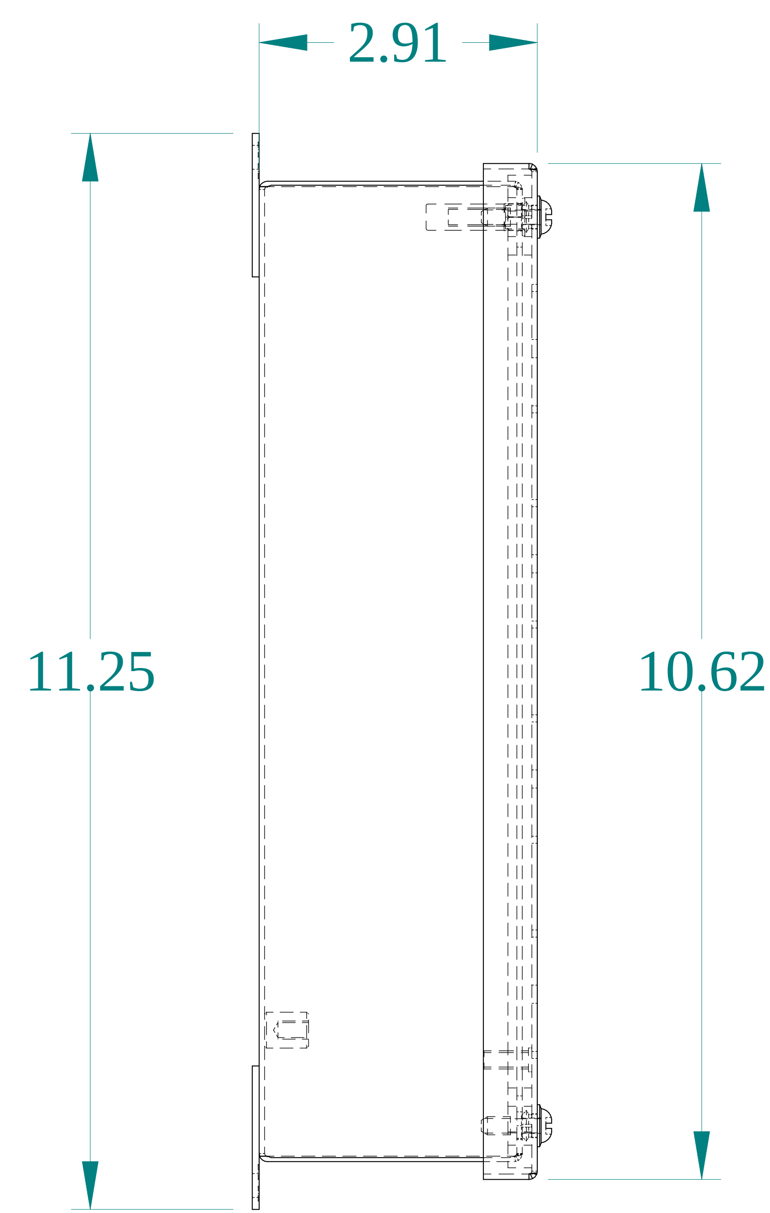
SIDE VIEW
