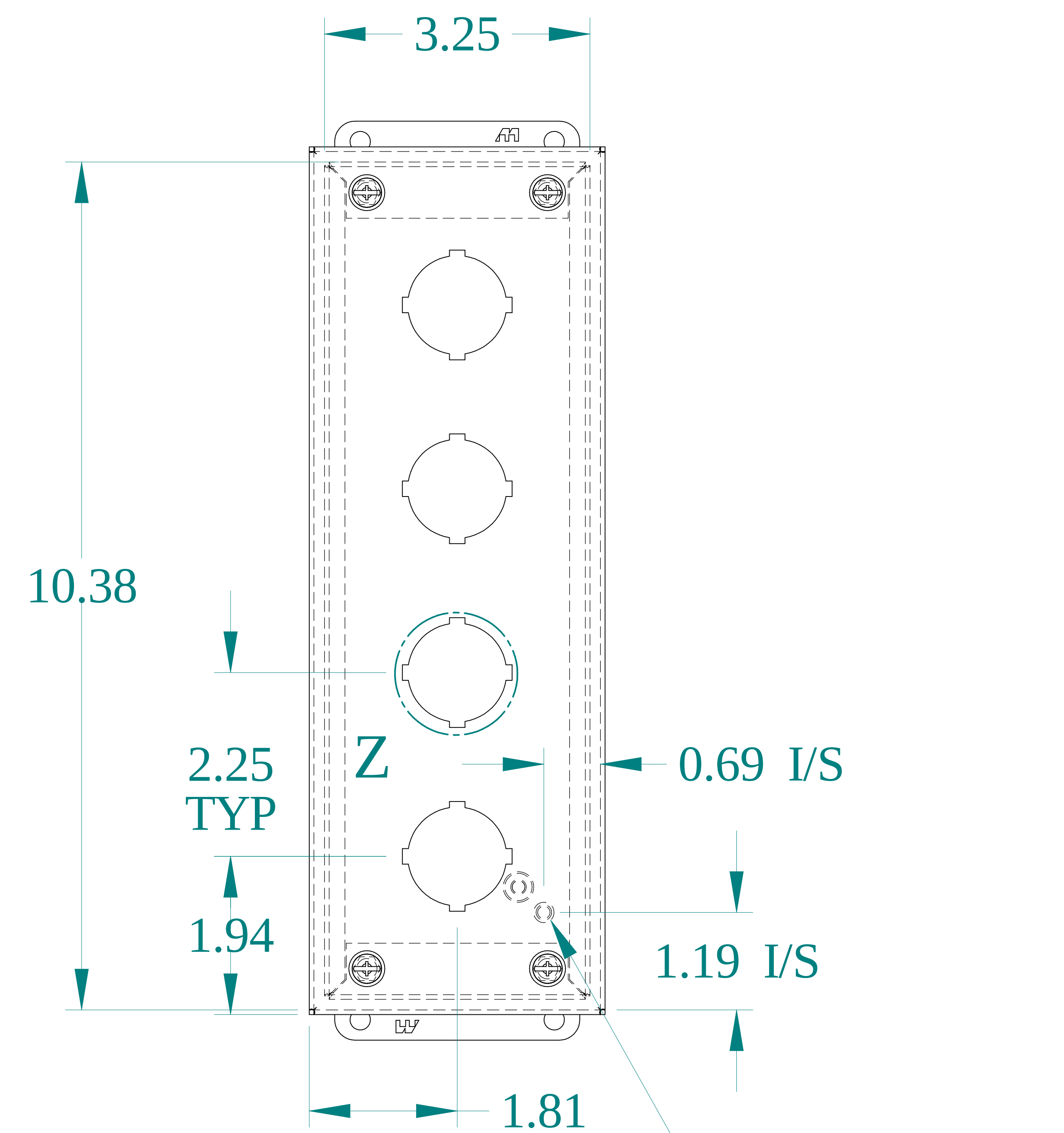
FRONT VIEW
