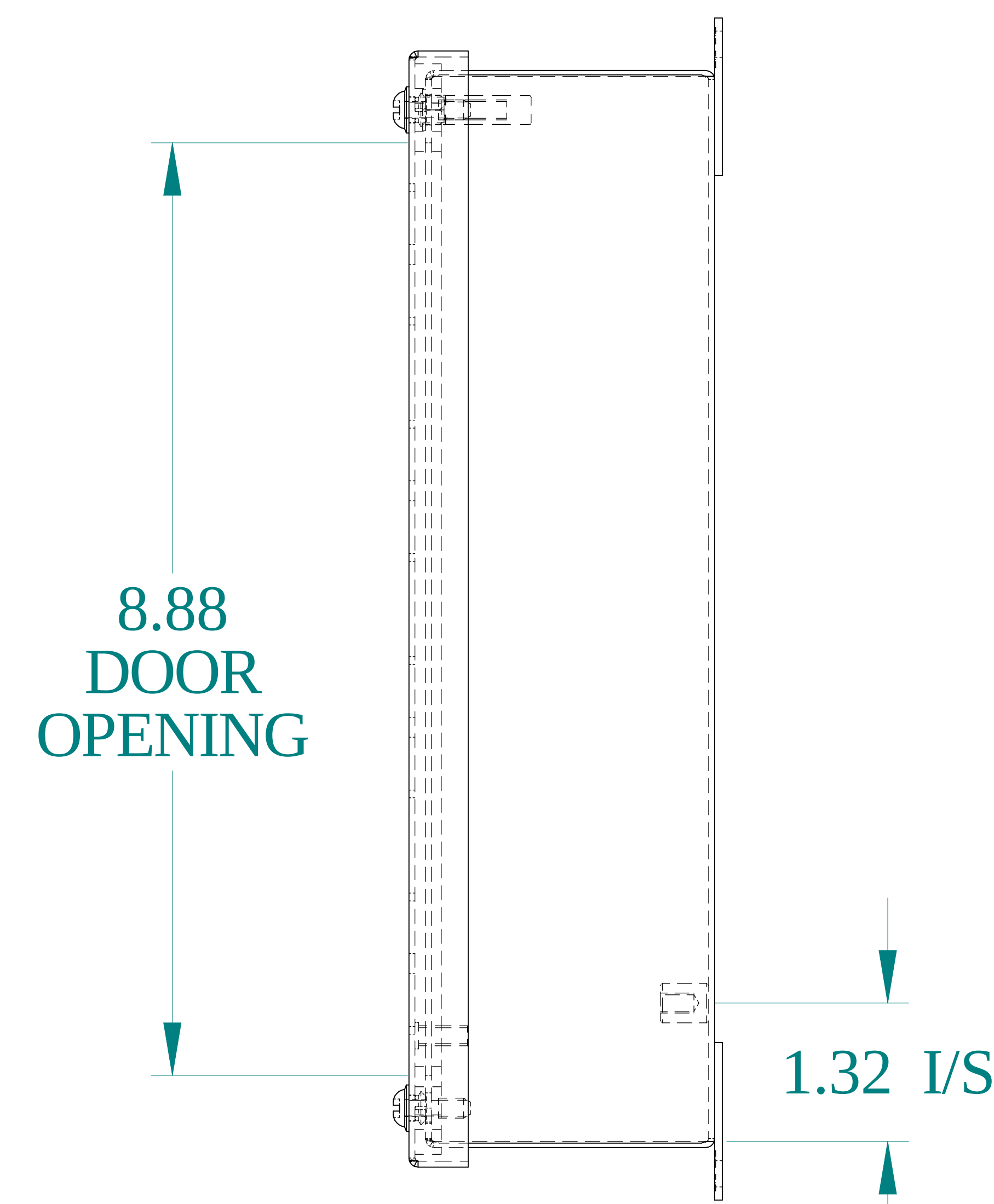
SIDE VIEW
