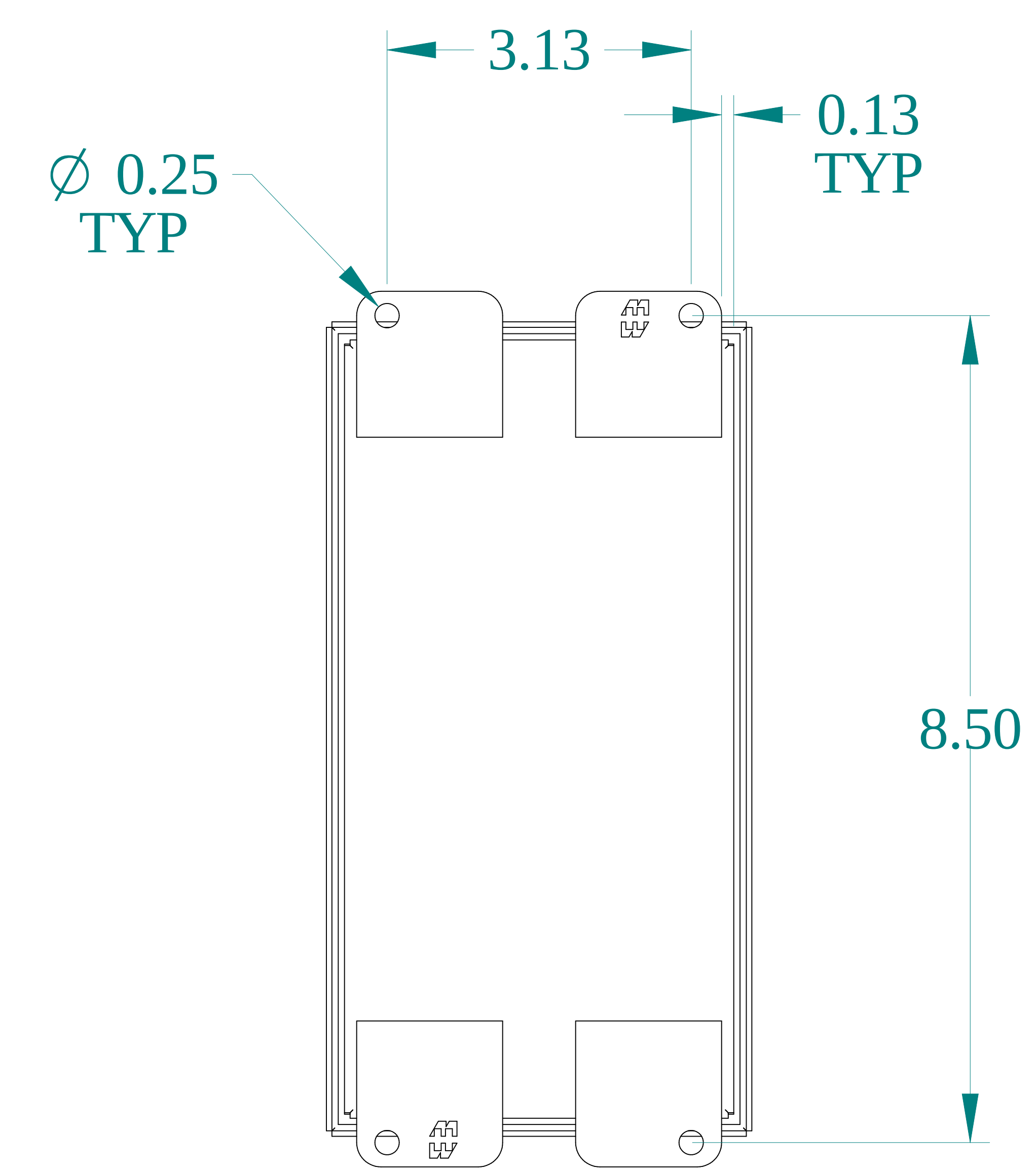
BACK VIEW
