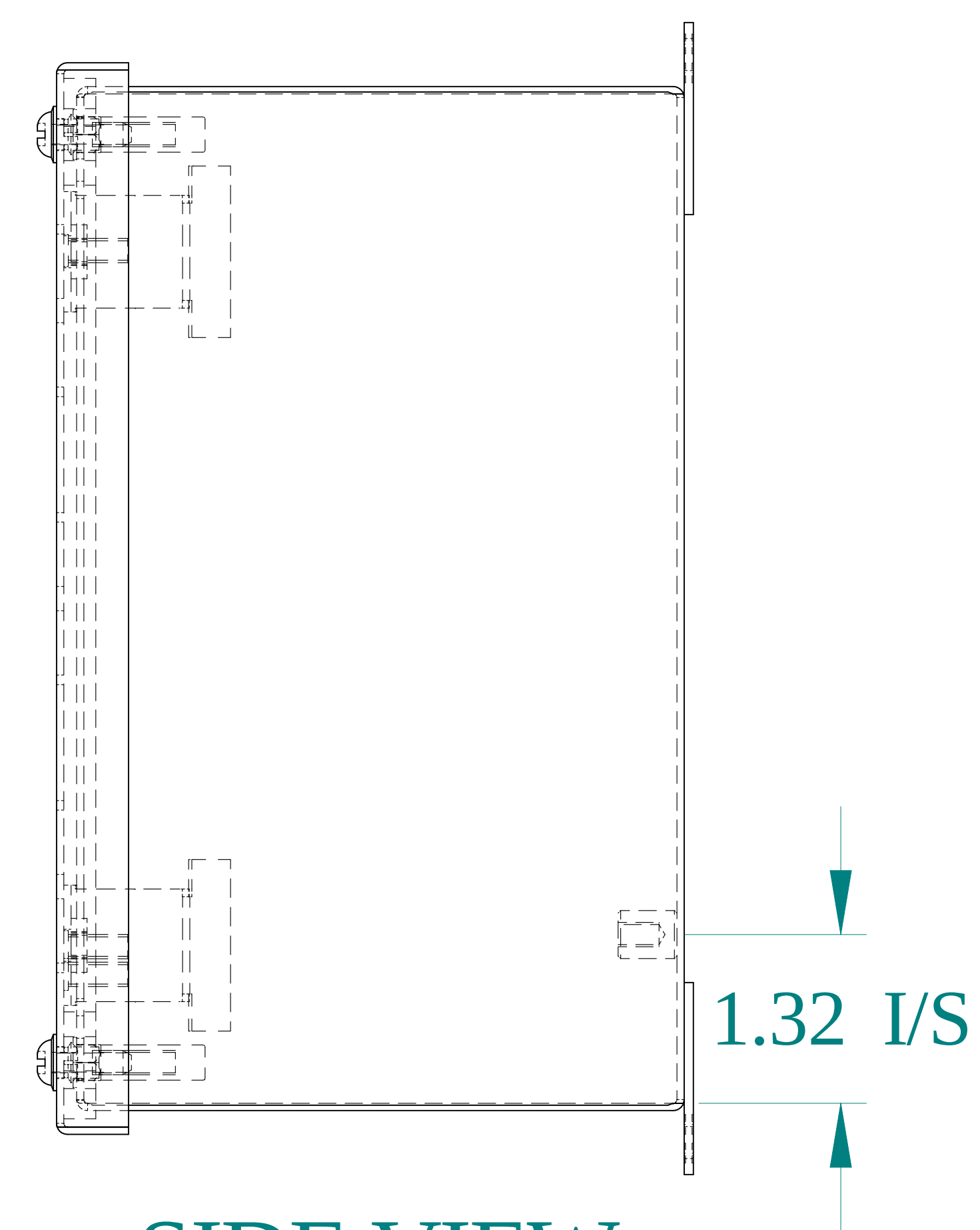
SIDE VIEW
