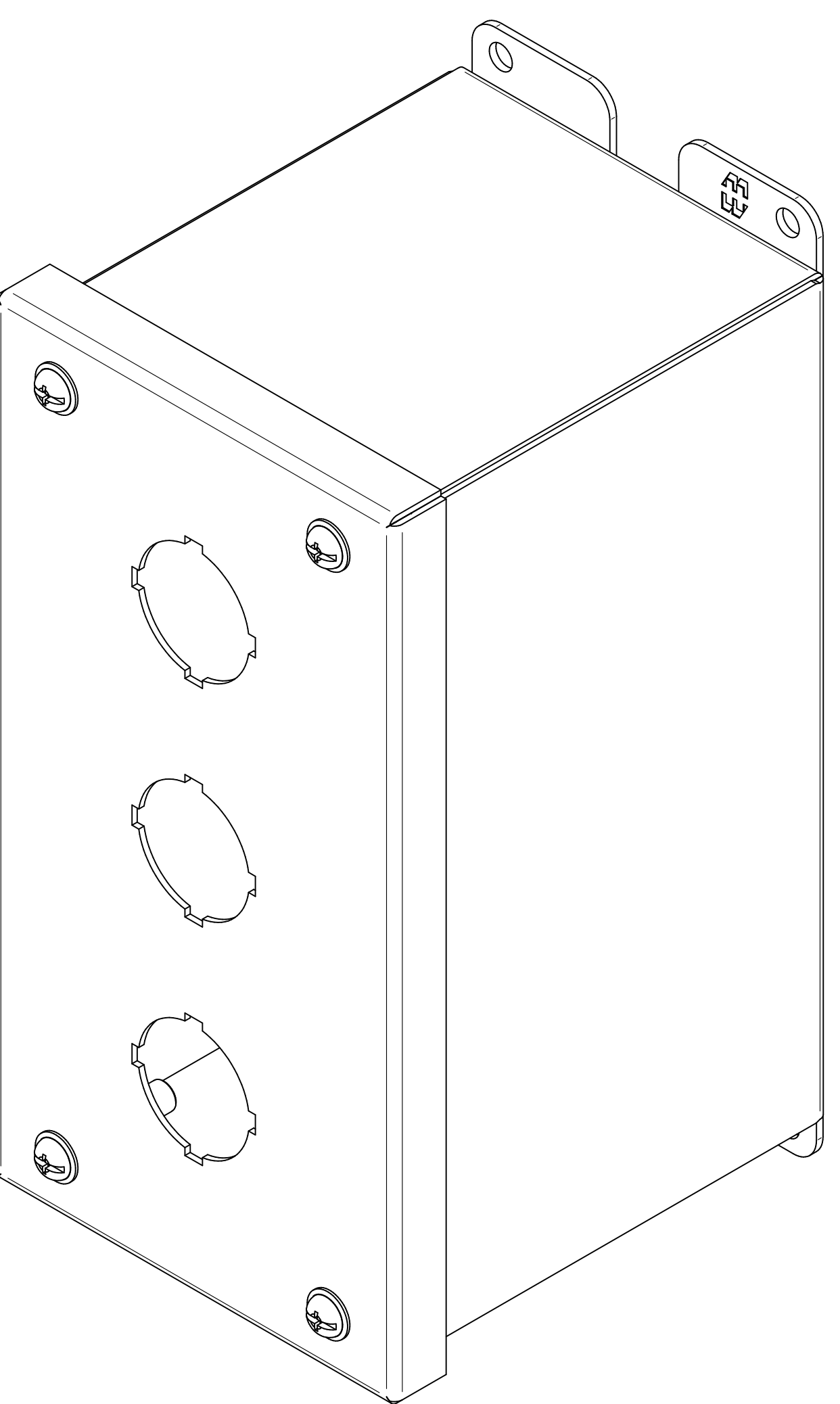
ISOMETRIC VIEWS
