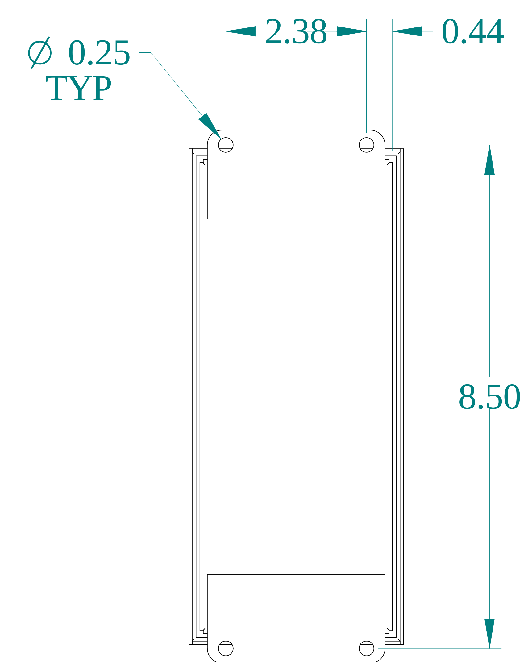
BACK VIEW
