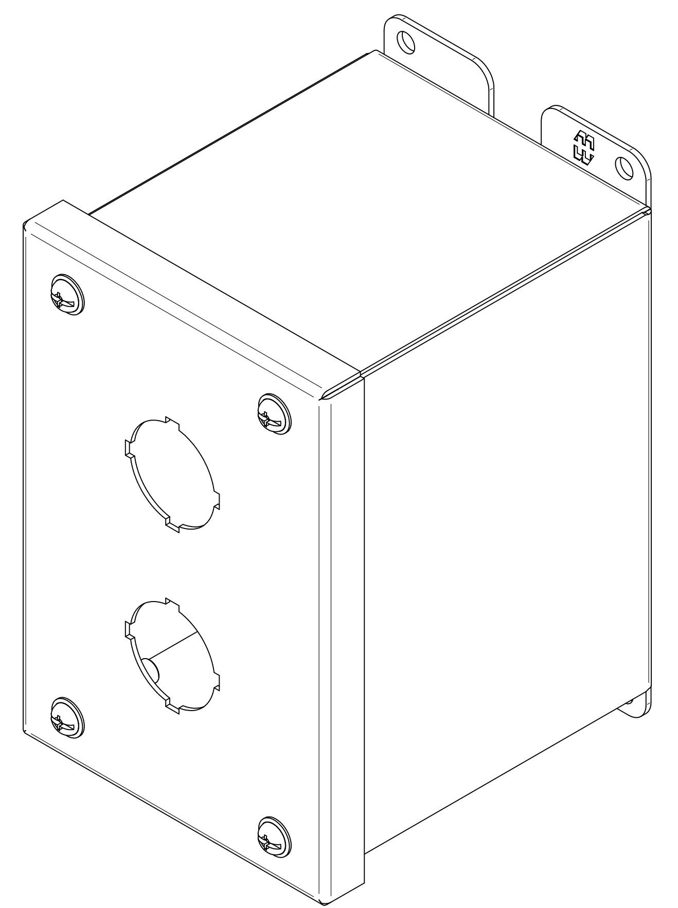
ISOMETRIC VIEWS
