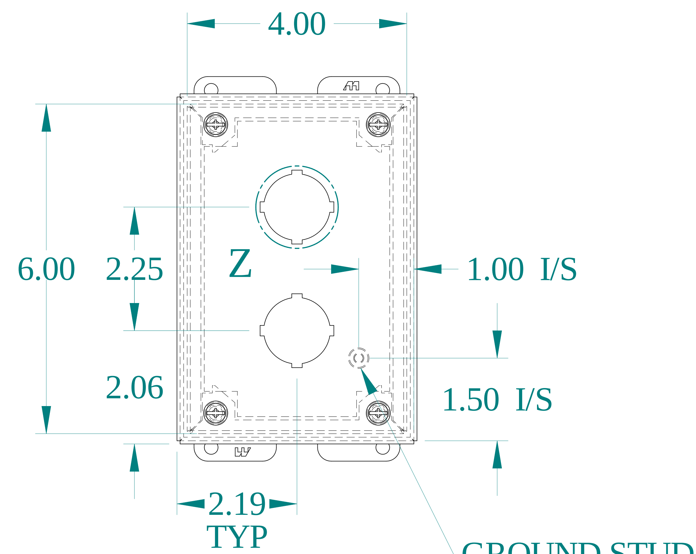
FRONT VIEW
