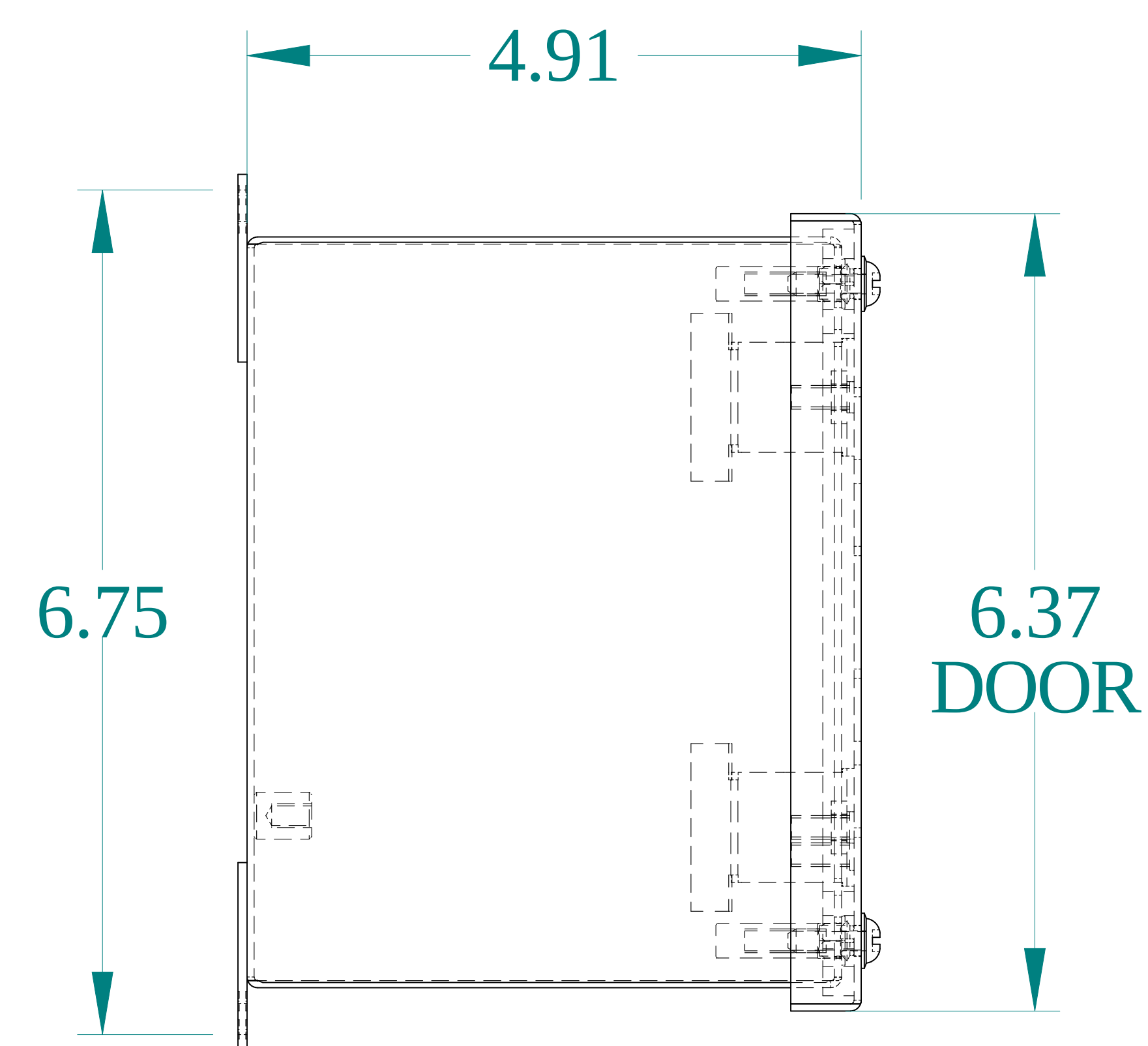
SIDE VIEW
