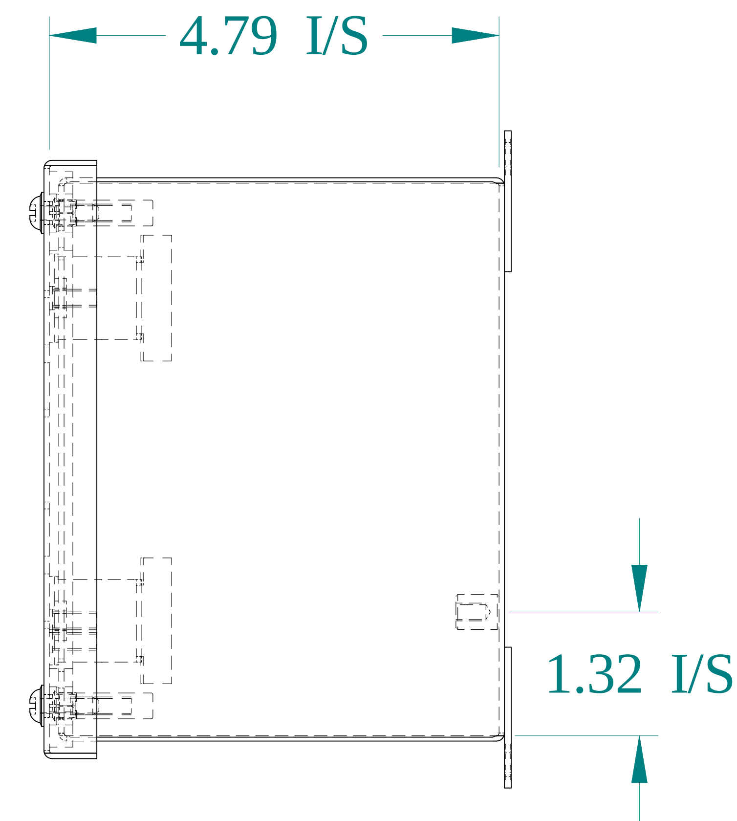
SIDE VIEW
