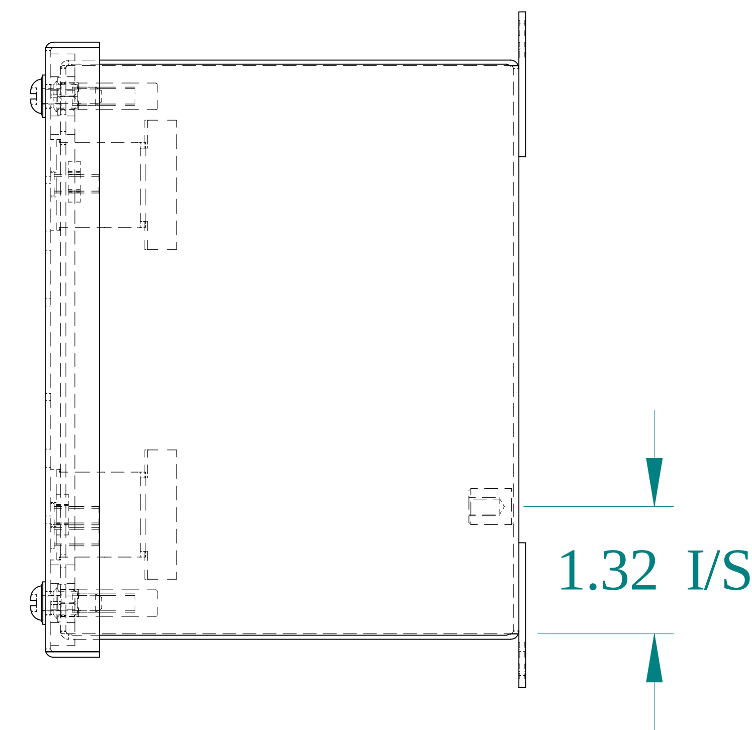
SIDE VIEW
