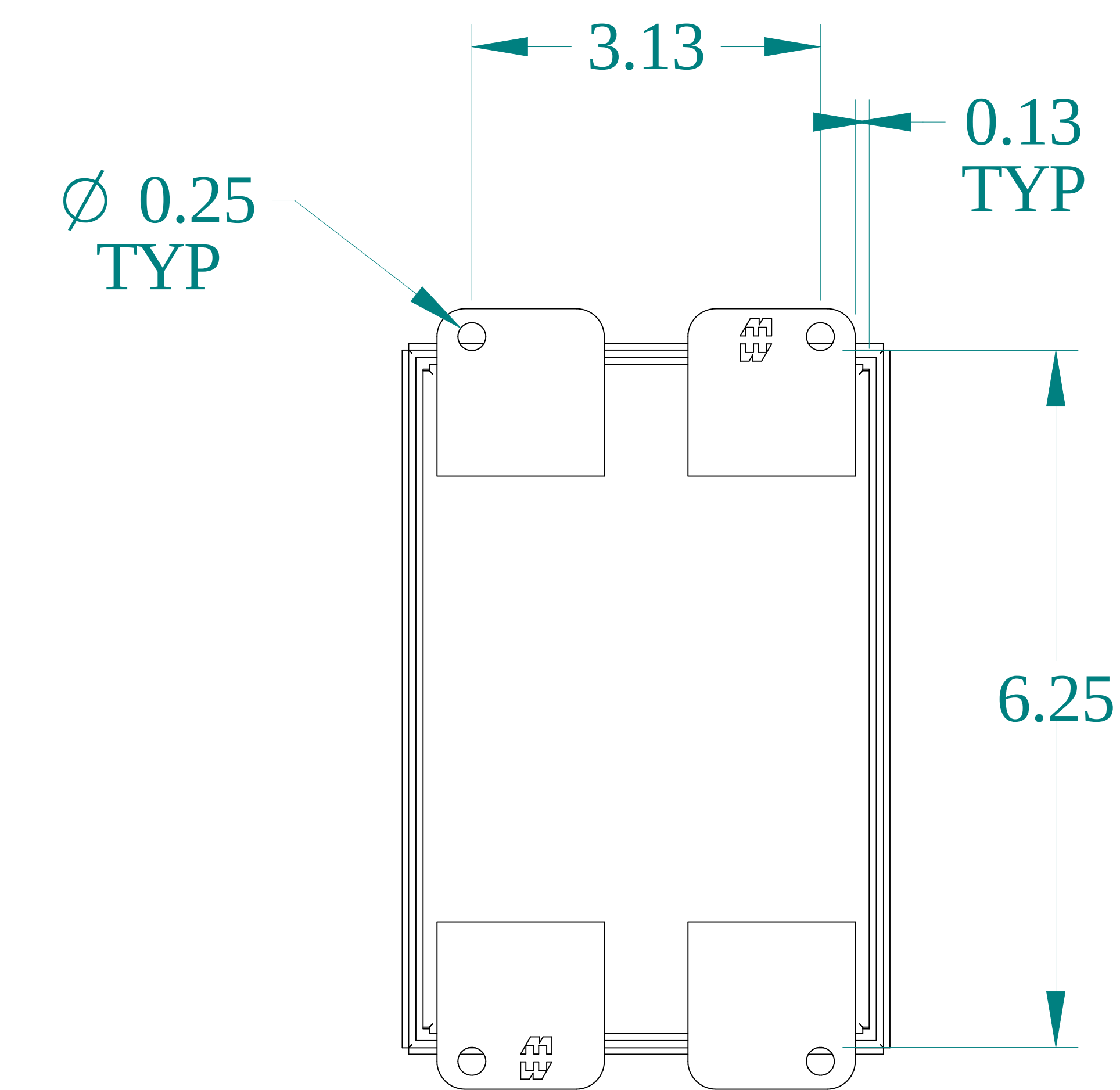
BACK VIEW
