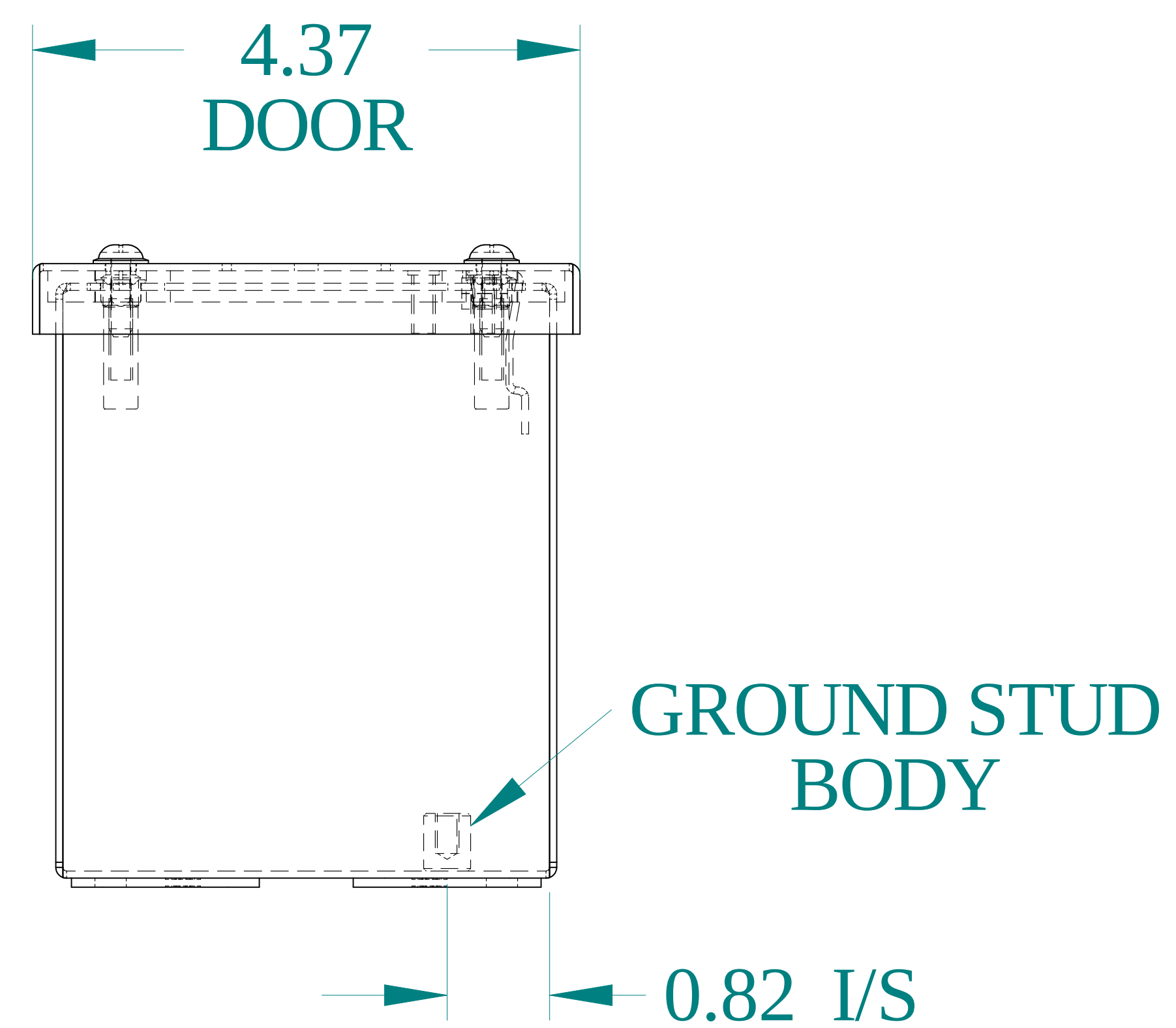
BOTTOM VIEW
