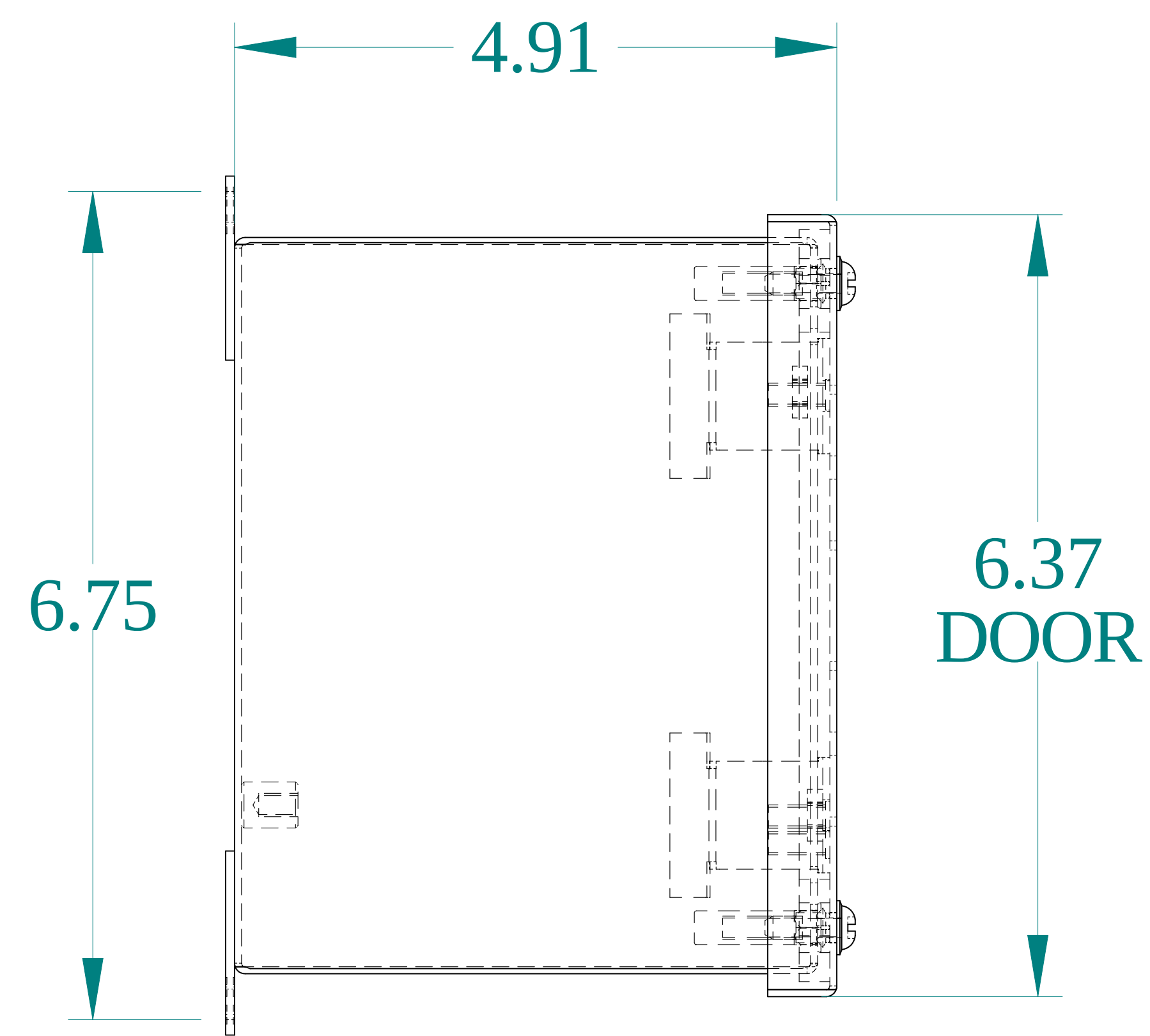
SIDE VIEW
