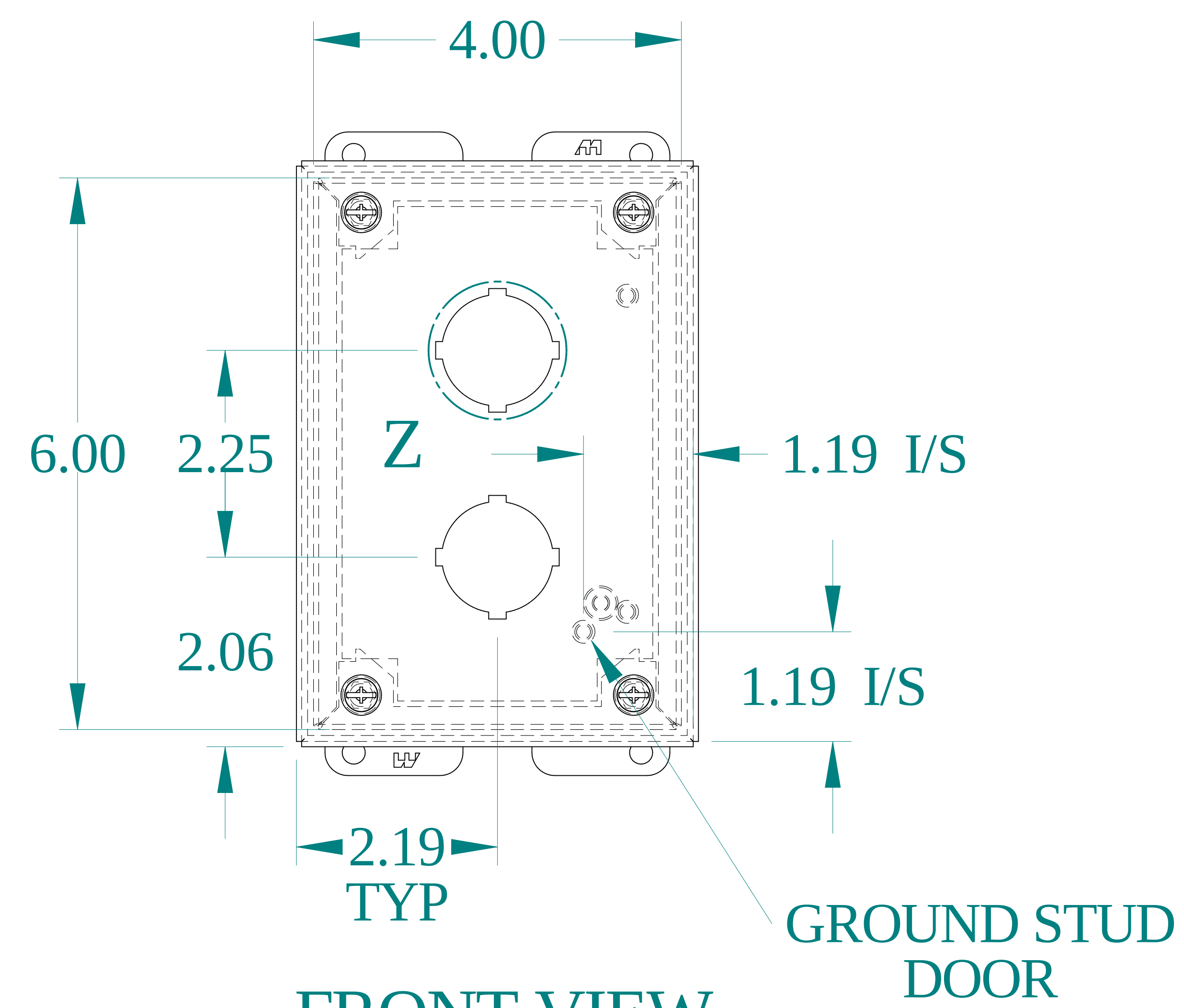
FRONT VIEW
