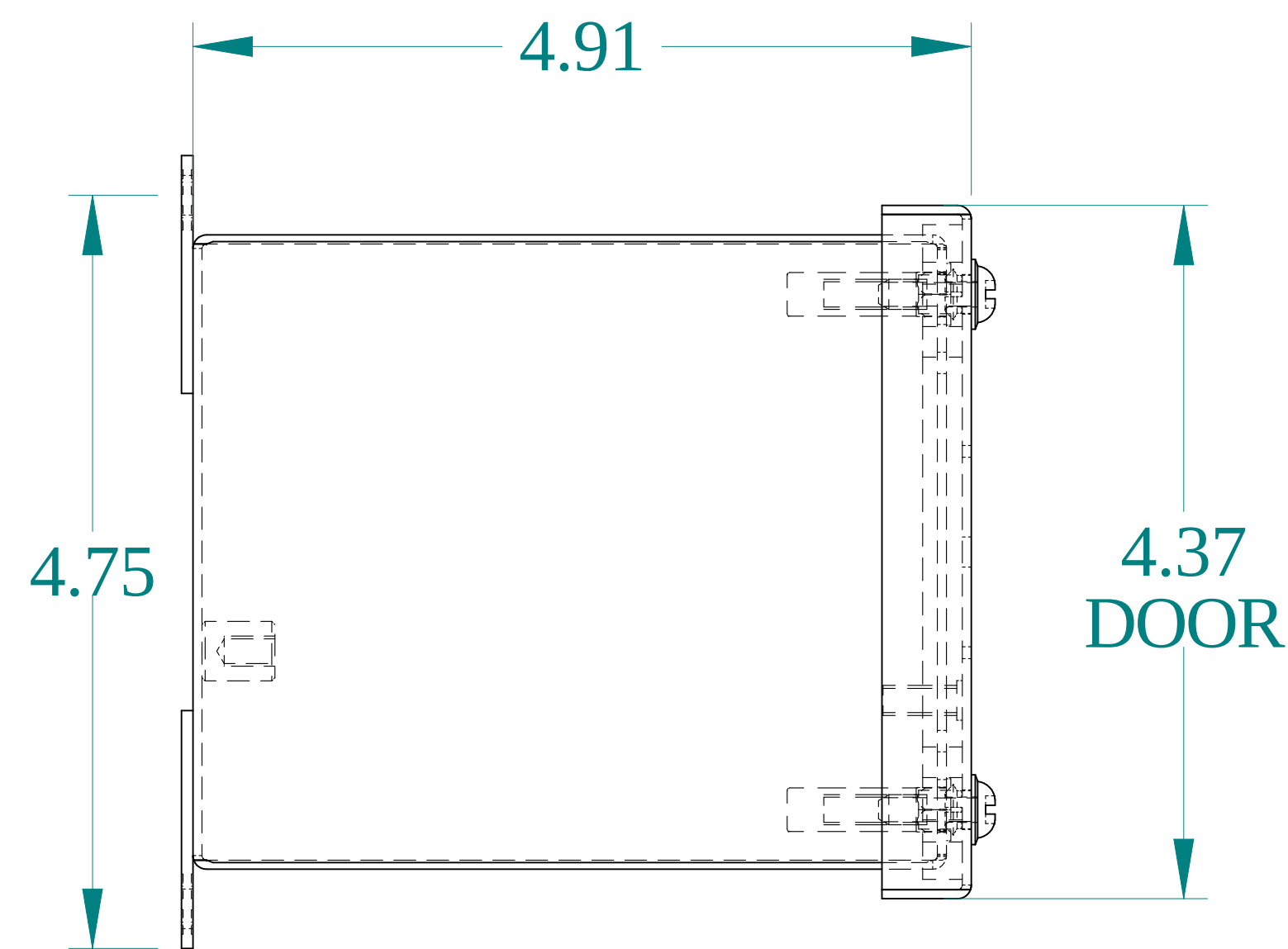
SIDE VIEW
