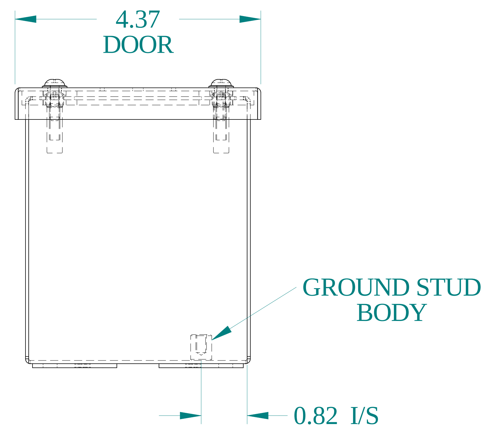
BOTTOM VIEW
