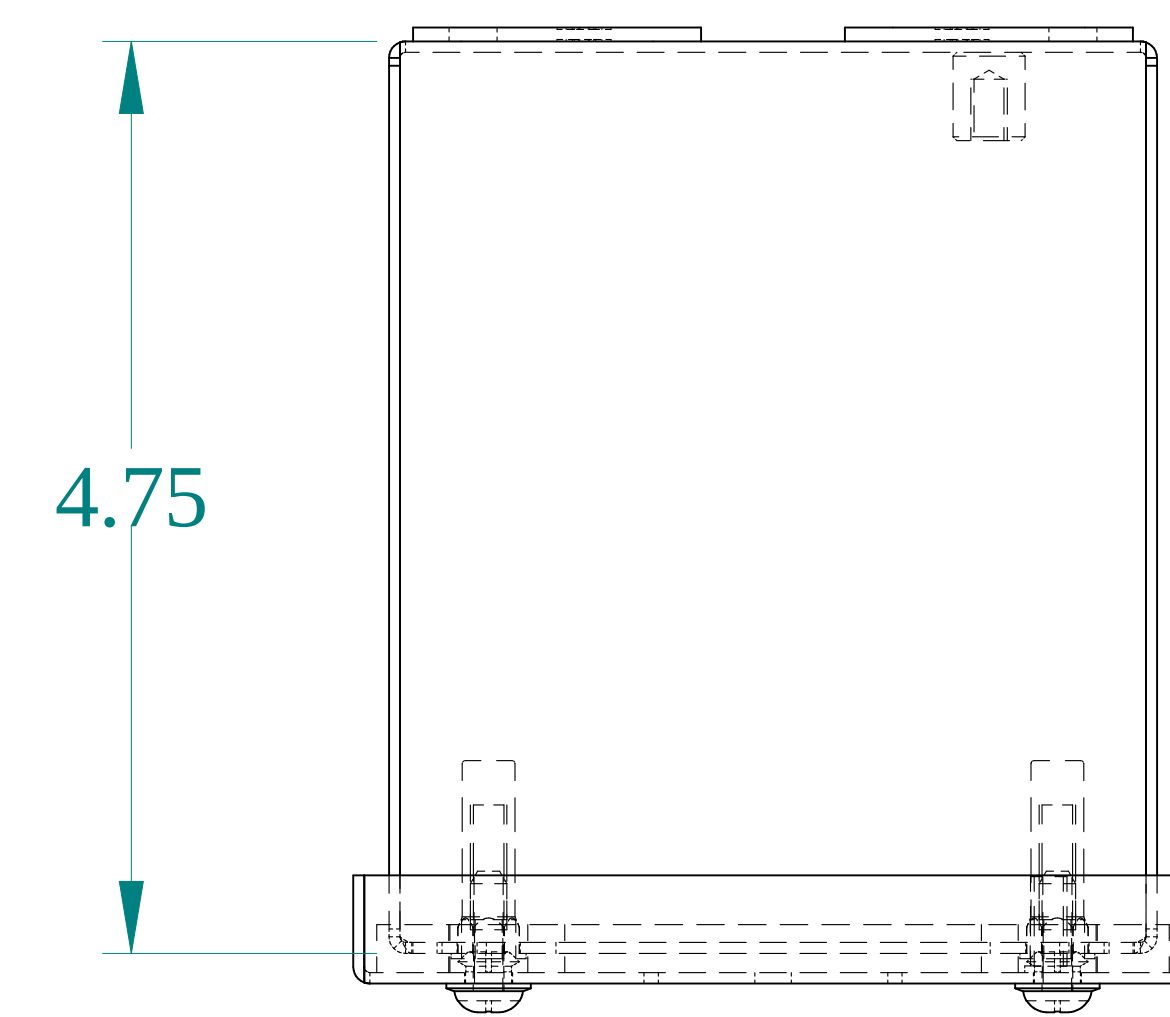
TOP VIEW
