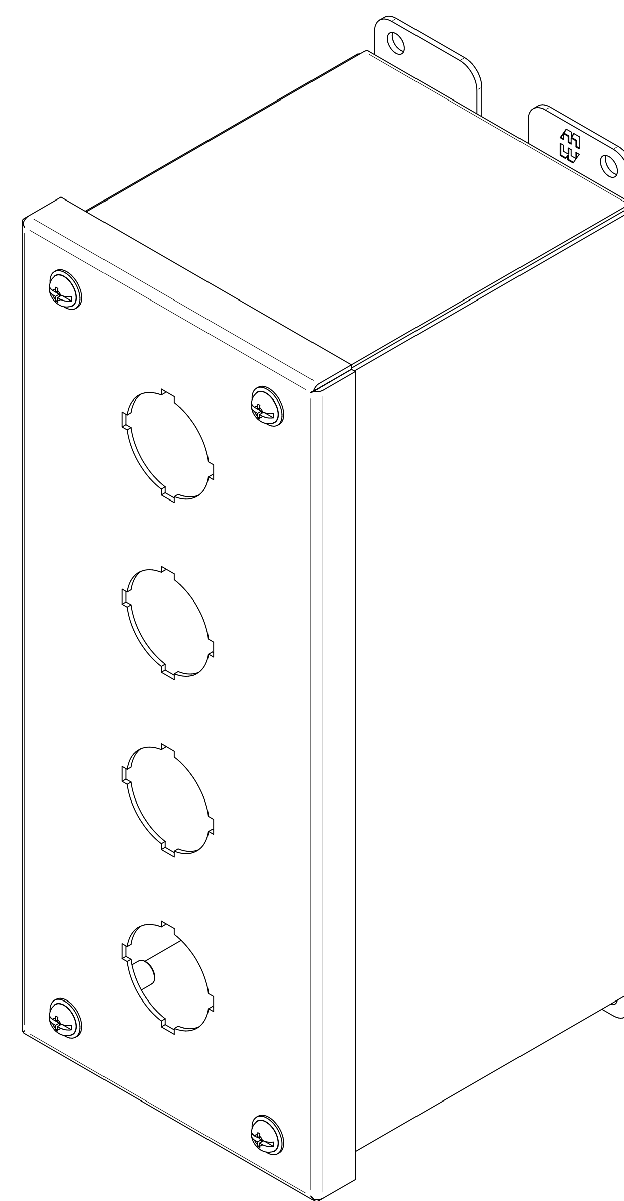
ISOMETRIC VIEWS
