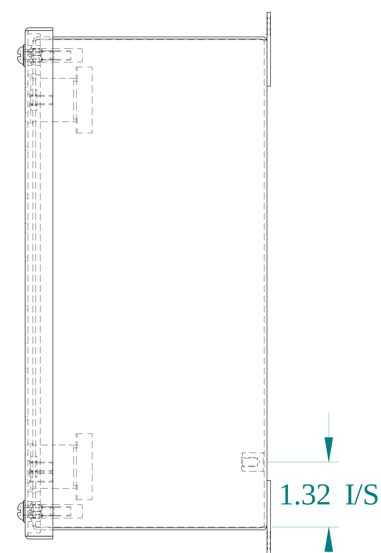
SIDE VIEW
