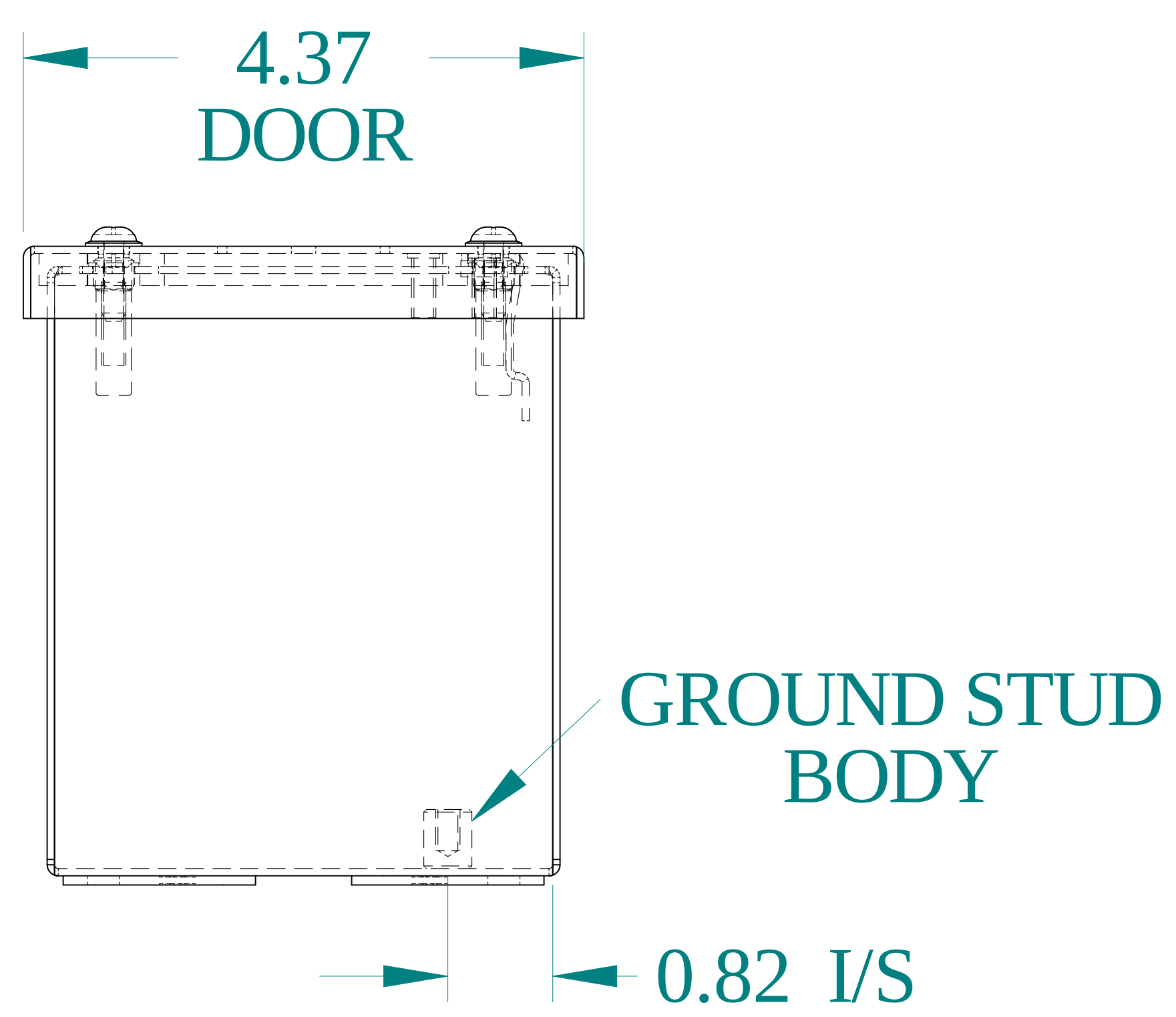
BOTTOM VIEW
