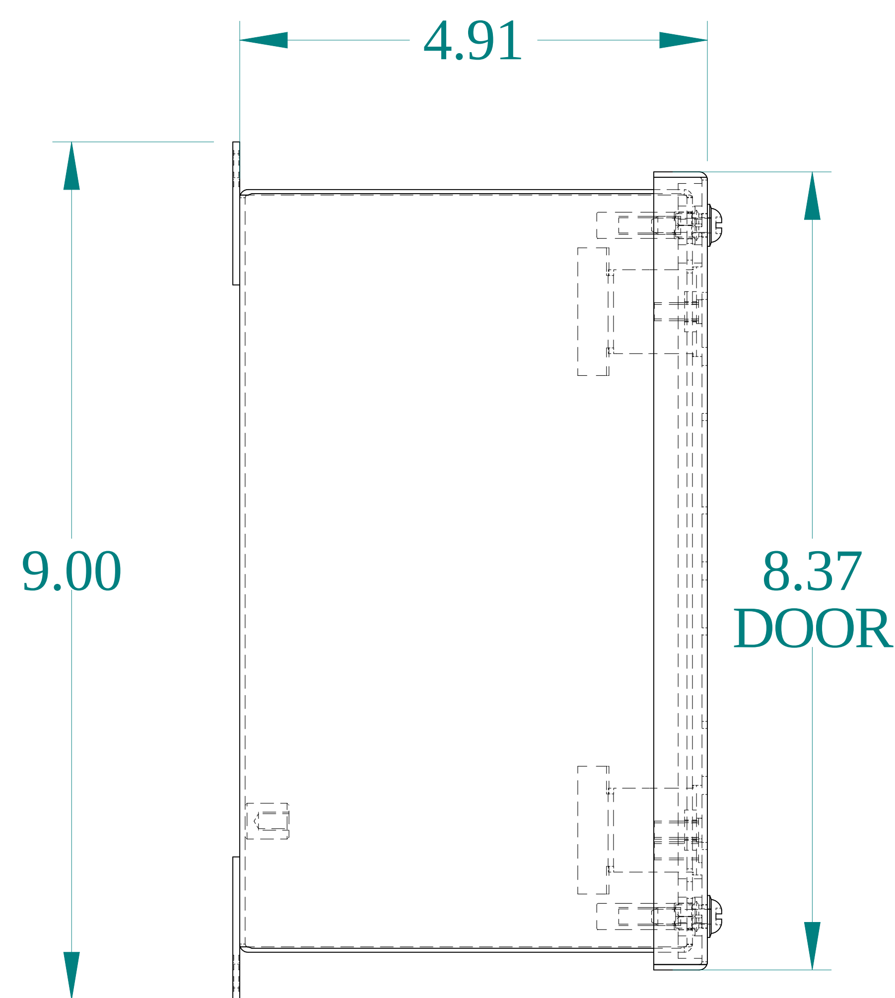
SIDE VIEW
