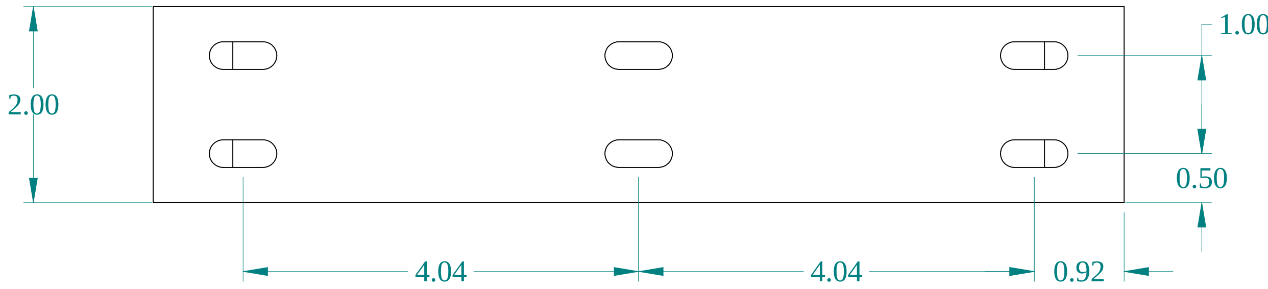
BOTTOM VIEW
