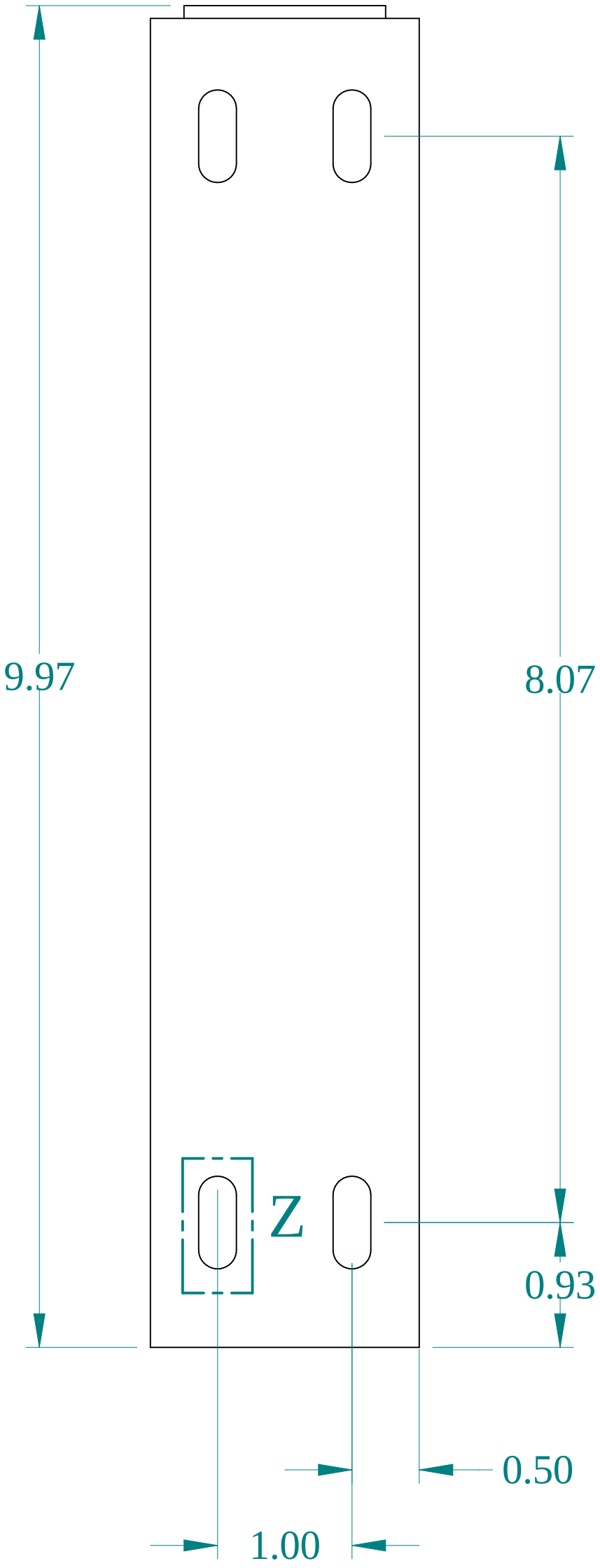
SIDE VIEW
