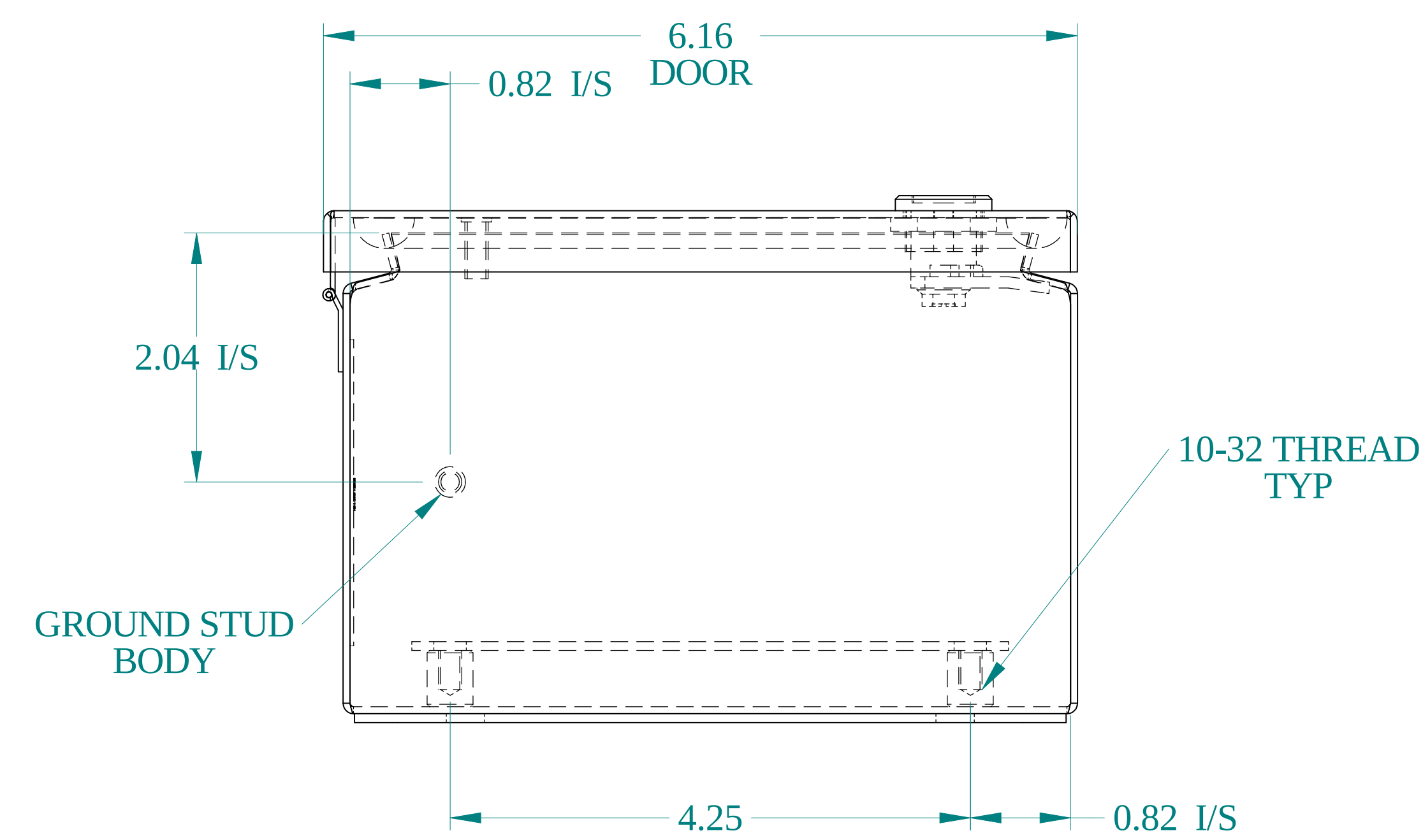
BOTTOM VIEW
