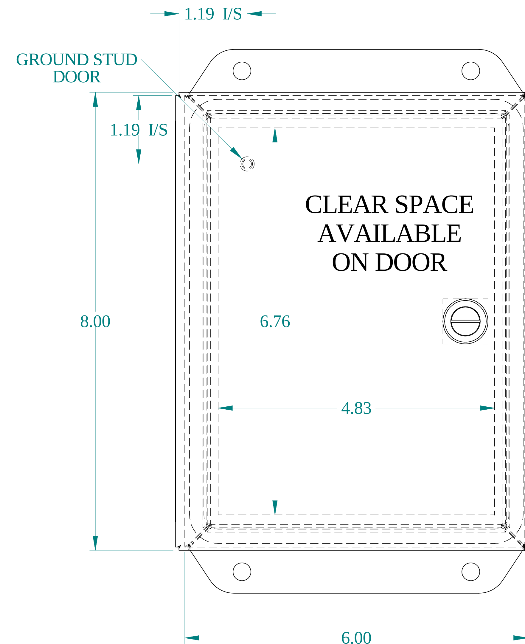
FRONT VIEW
