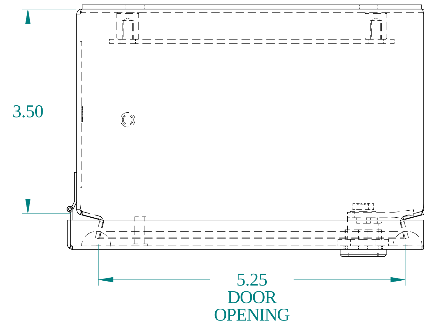
TOP VIEW
