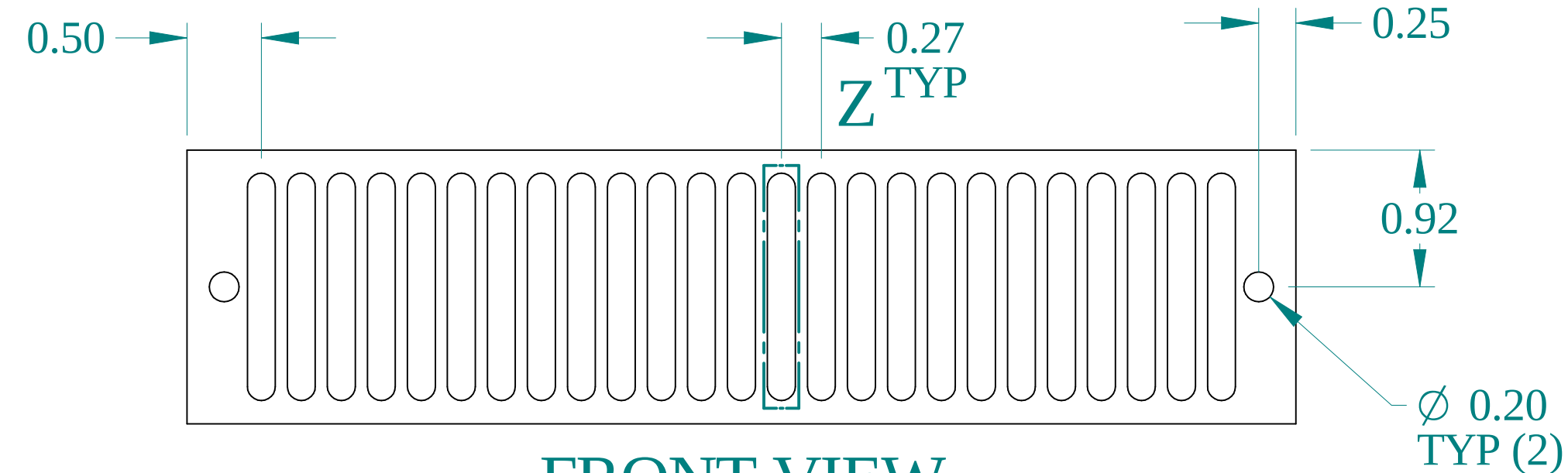
FRONT VIEW
