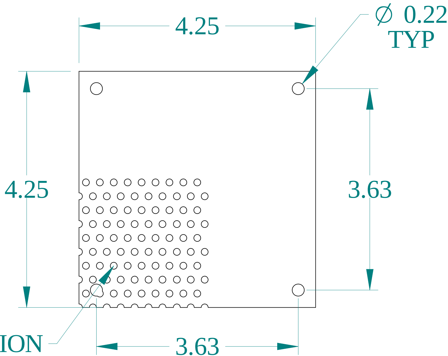
TOP VIEW
