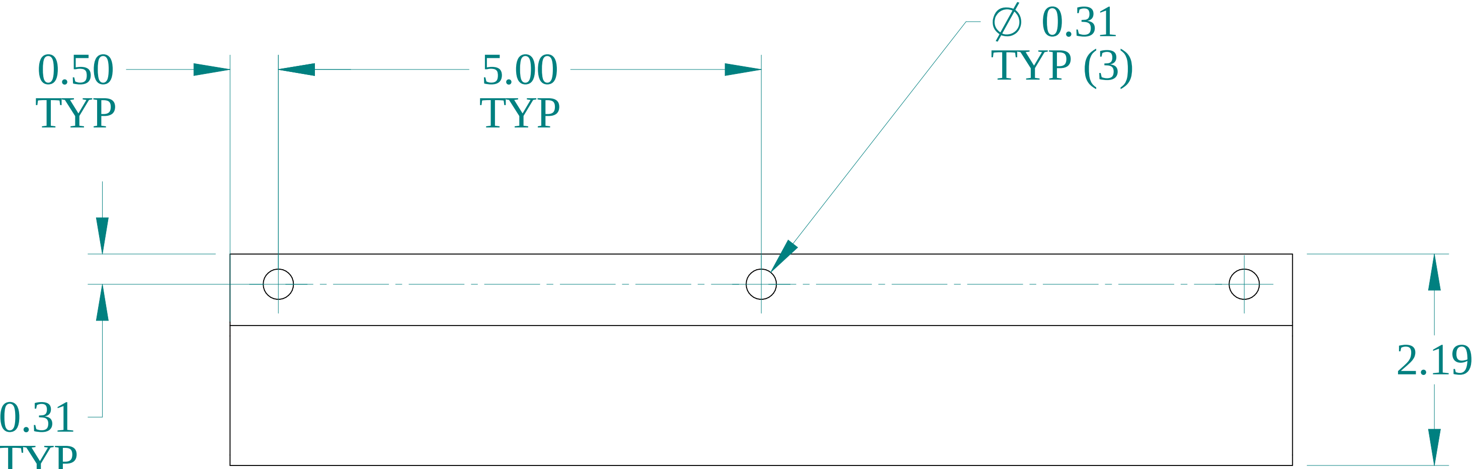
TOP VIEW
