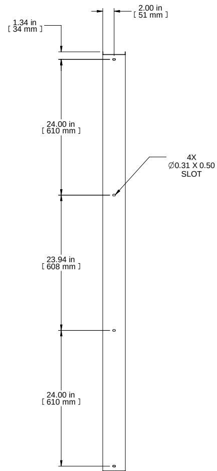
R.S. VIEW
