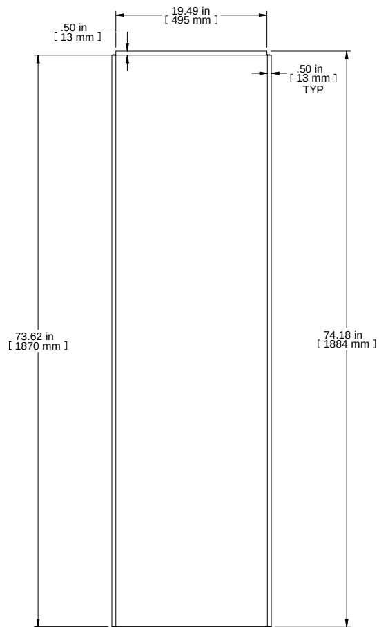
FRONT VIEW
