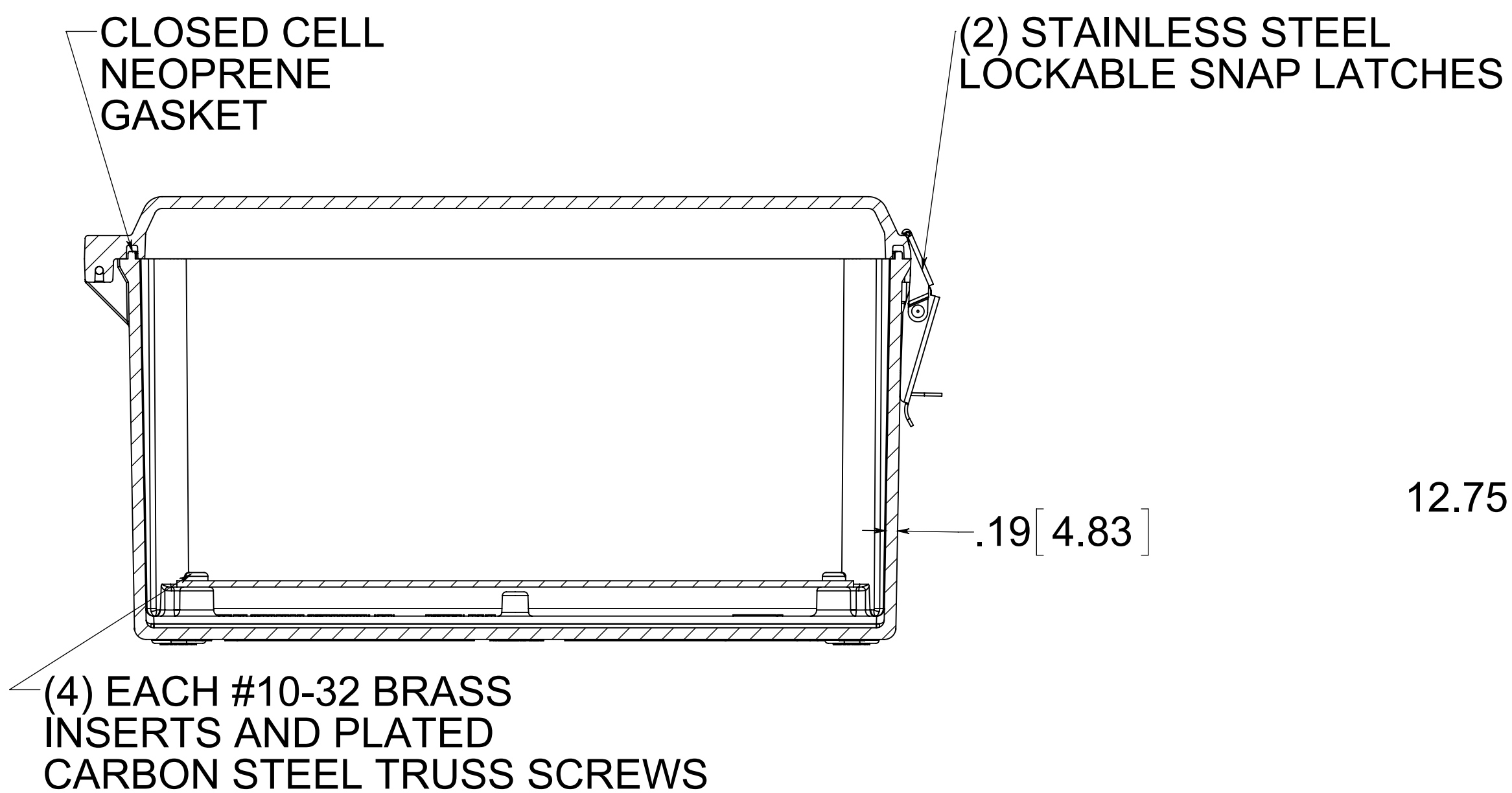
SECTION B-B
