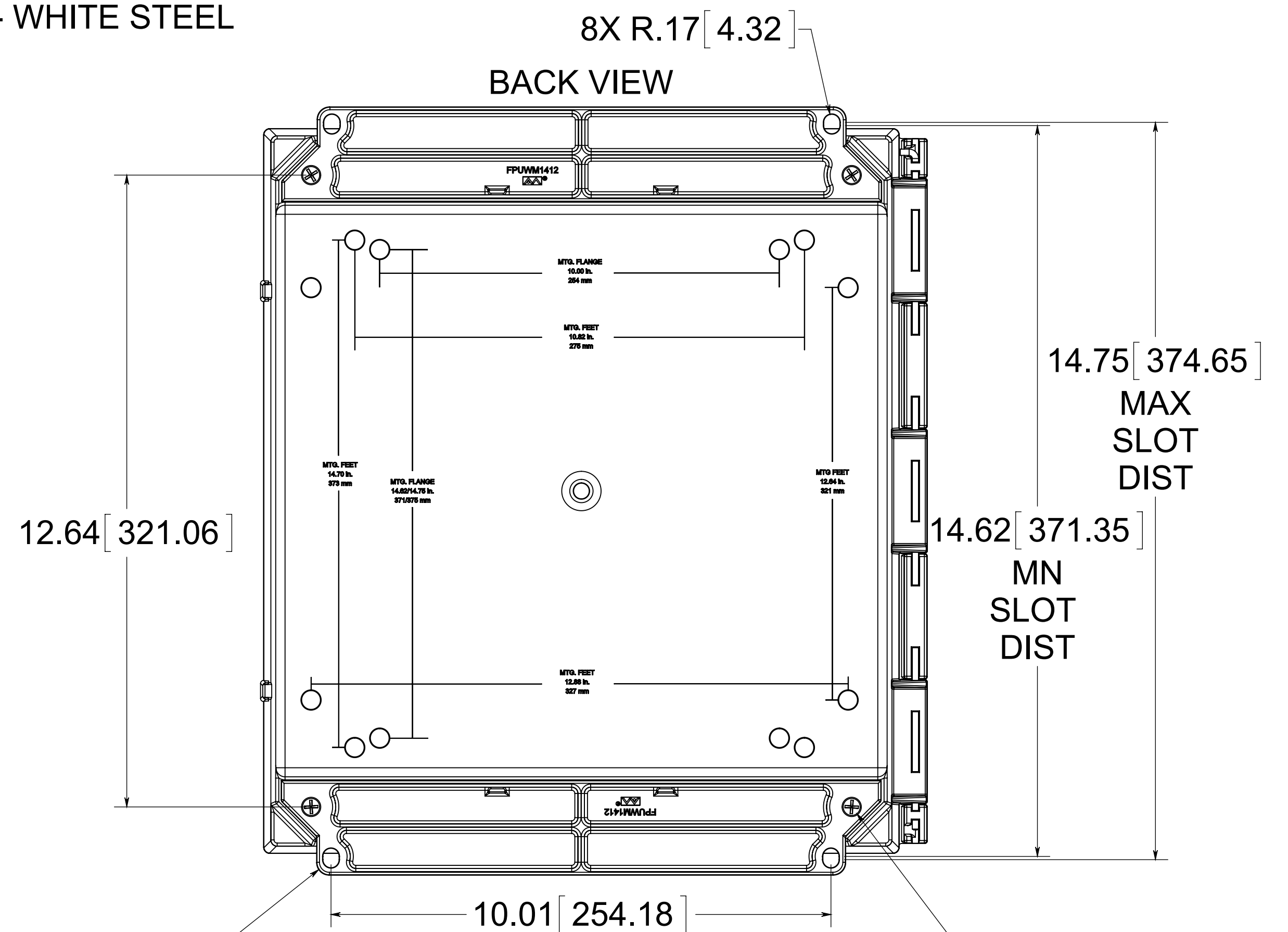
(4) POLYCARBONATE FLANGE(GLUED)
