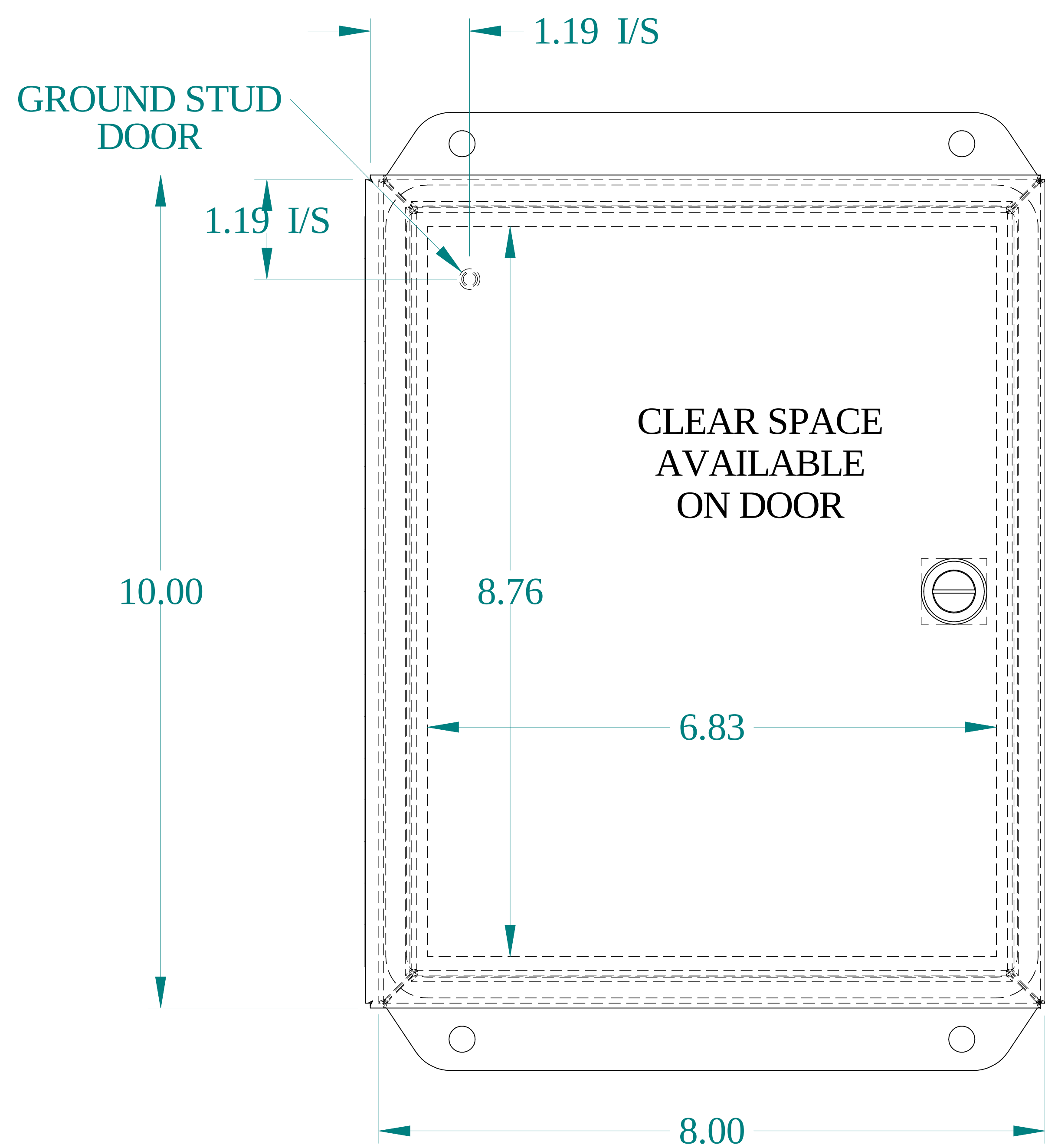
FRONT VIEW
