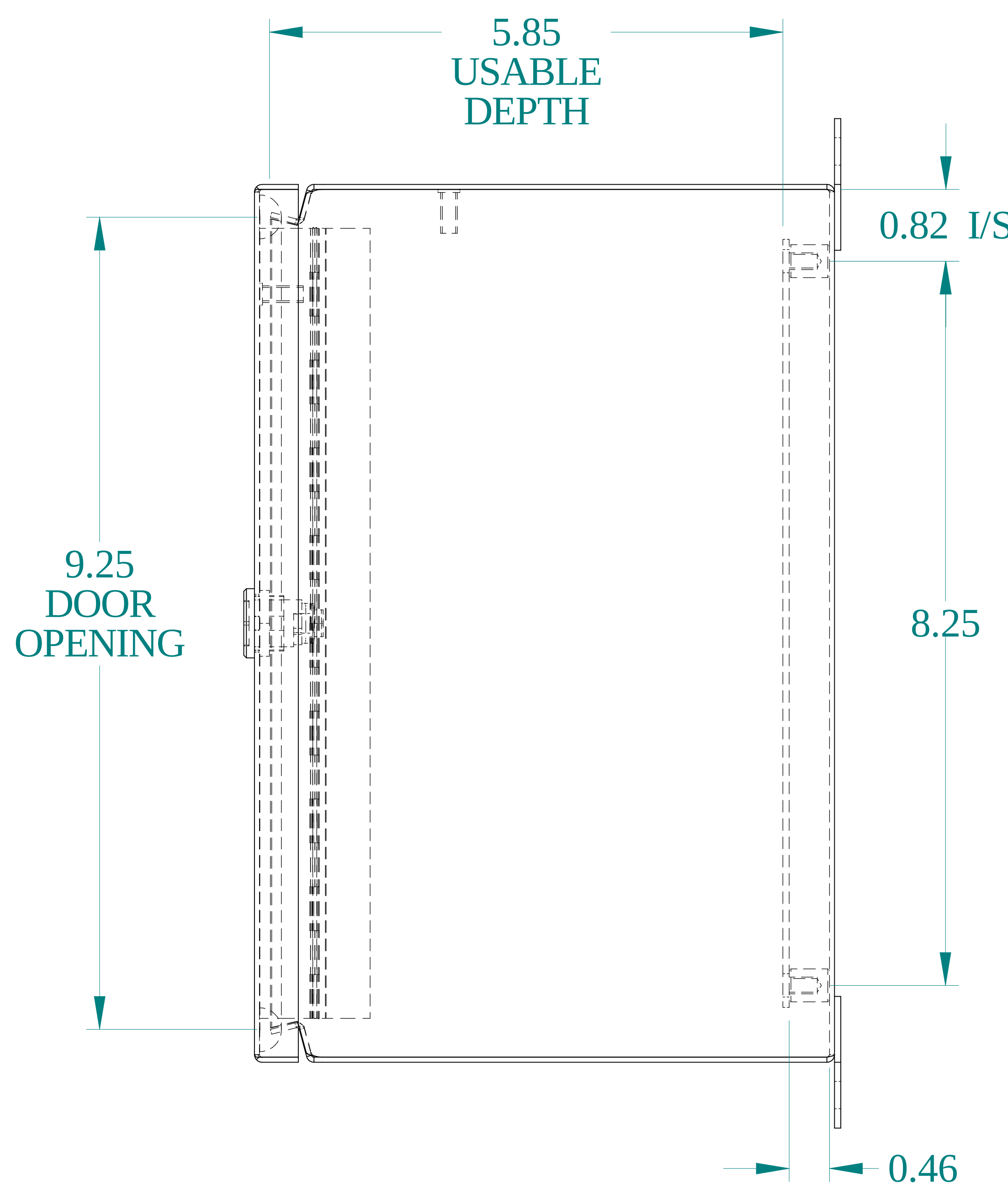
SIDE VIEW
