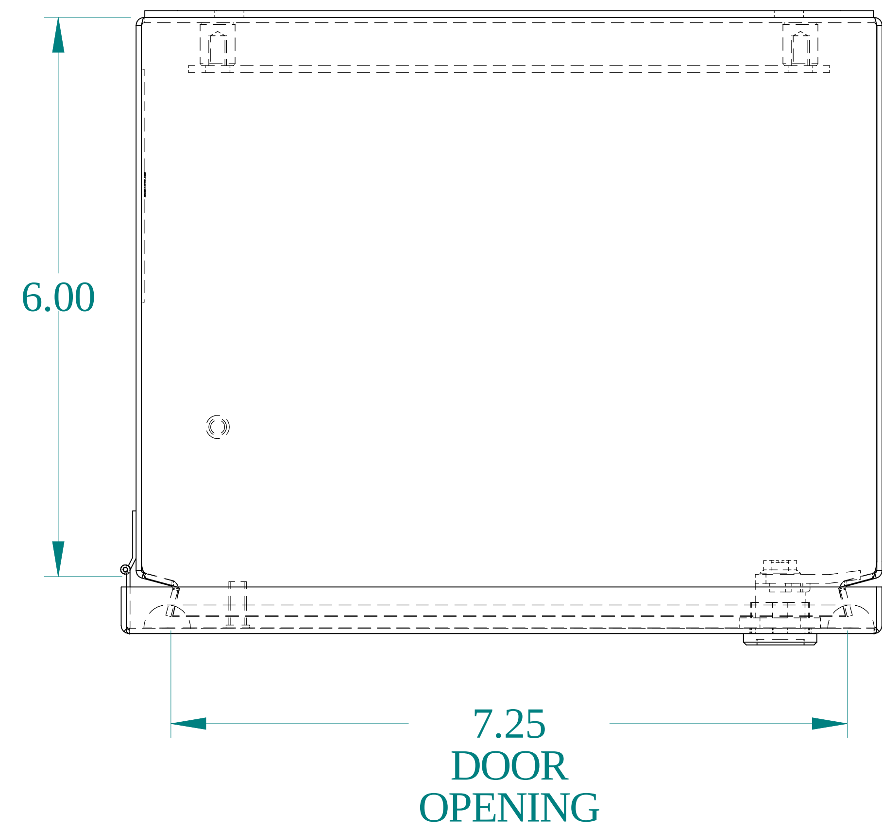
TOP VIEW
