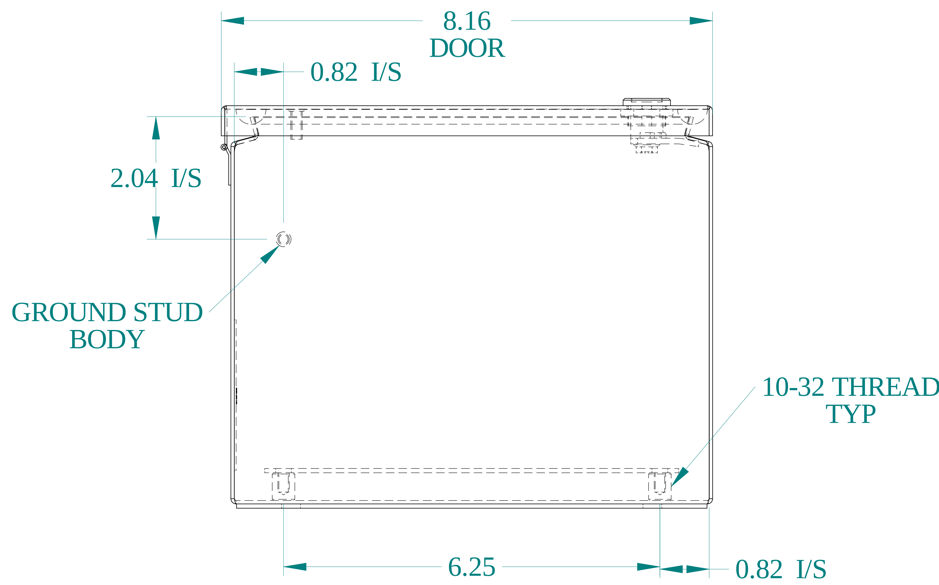
BOTTOM VIEW
