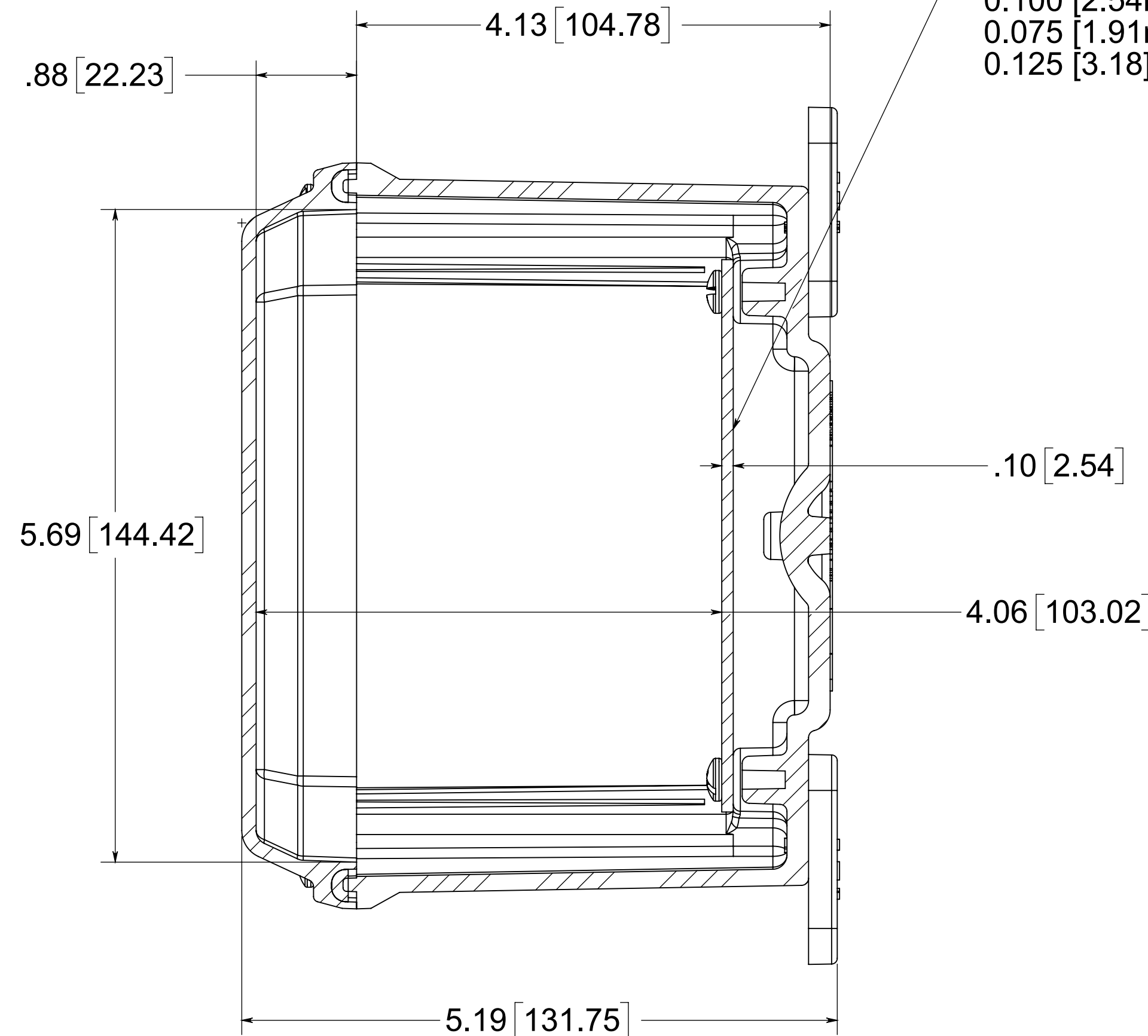
SECTION B-B
