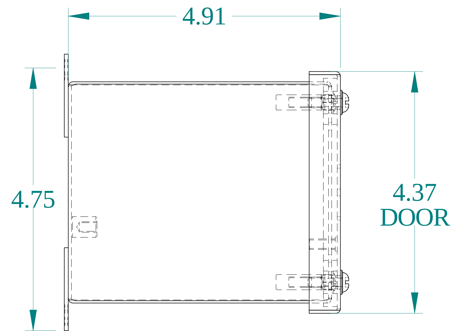
SIDE VIEW
