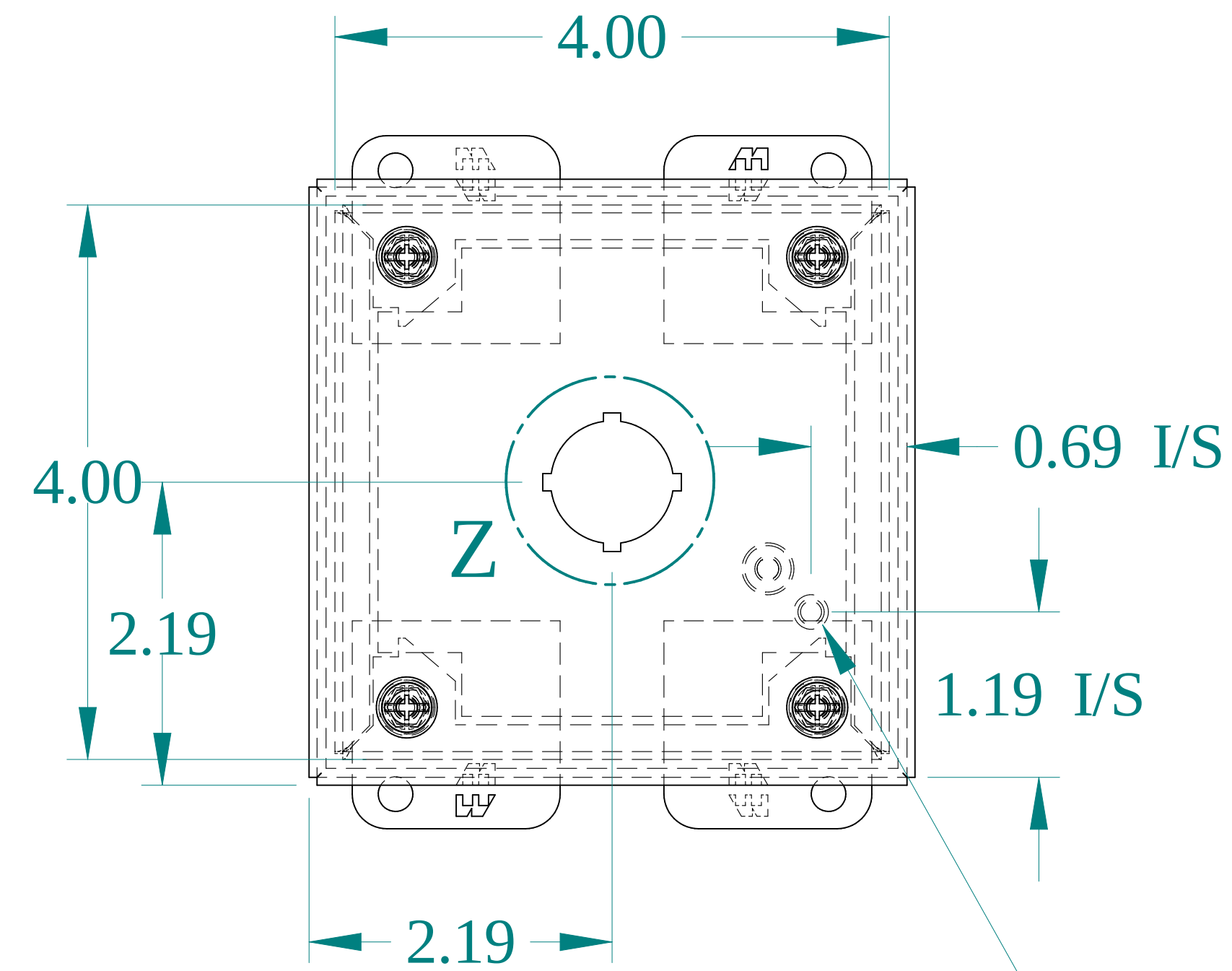
FRONT VIEW
