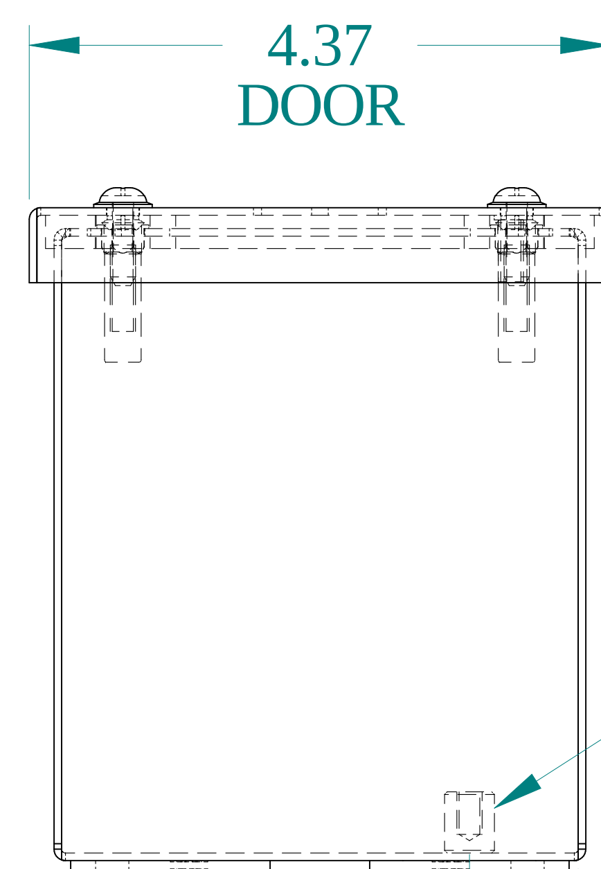
BOTTOM VIEW
