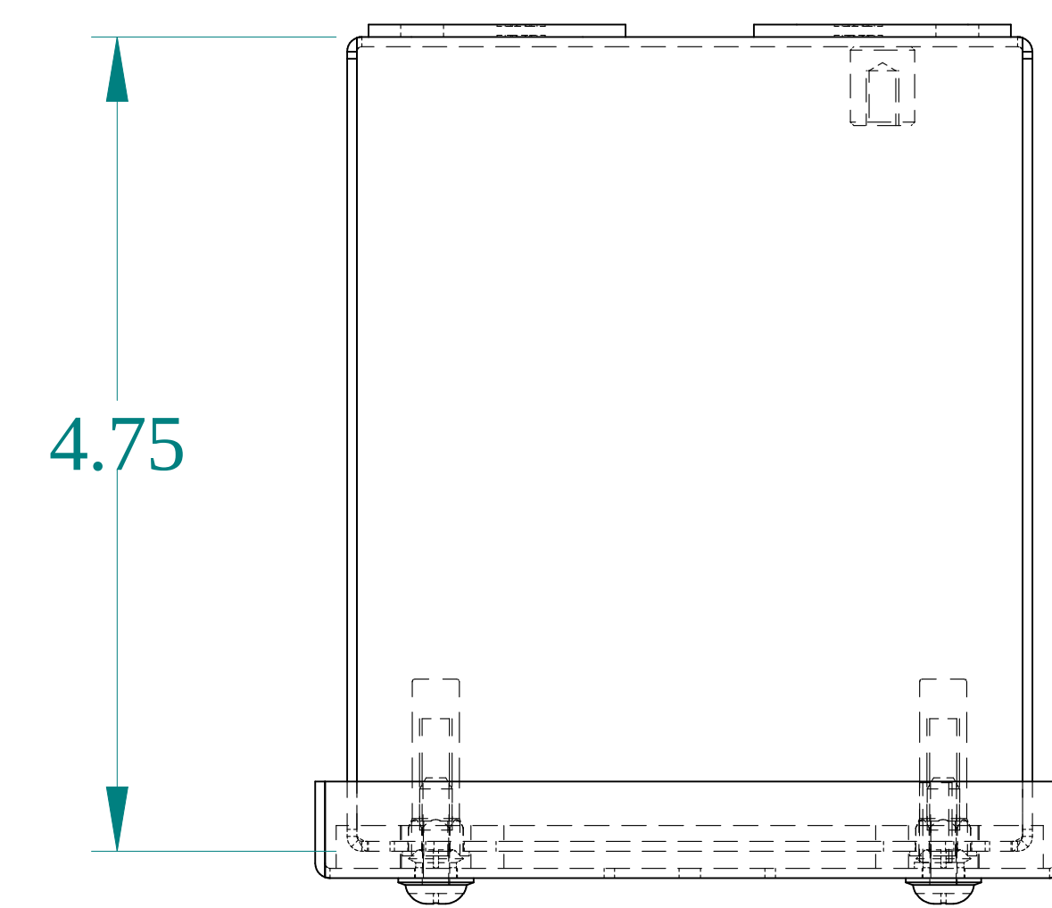
TOP VIEW
