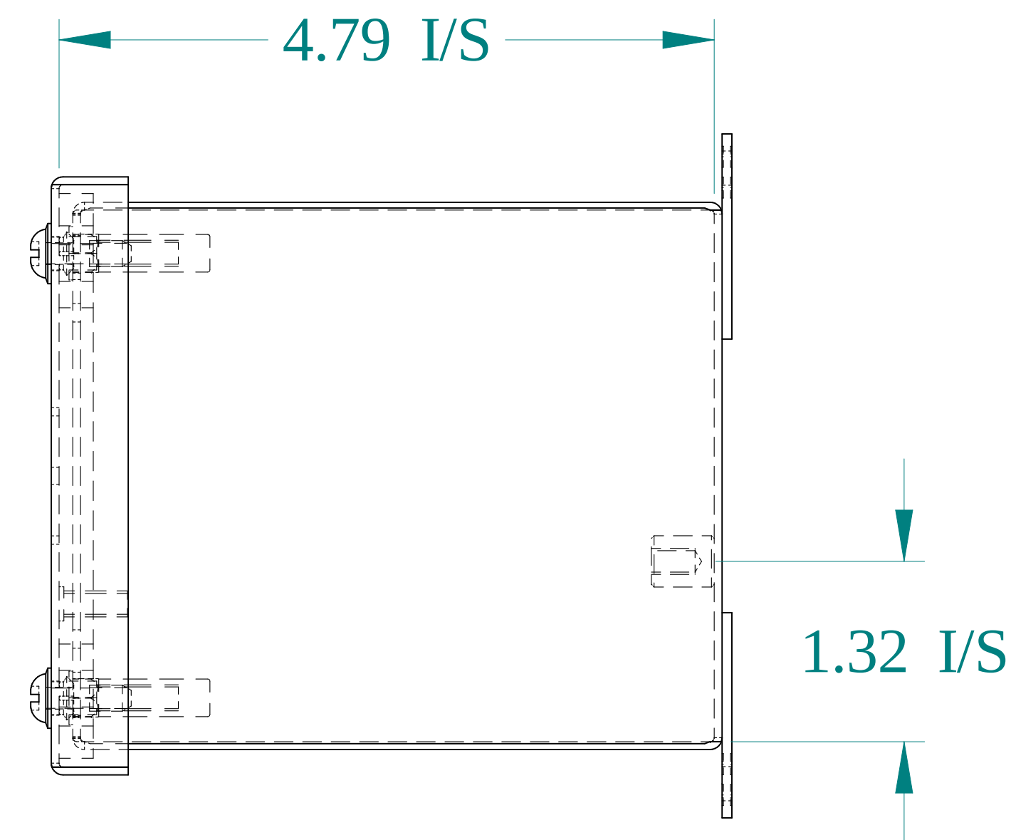
SIDE VIEW
