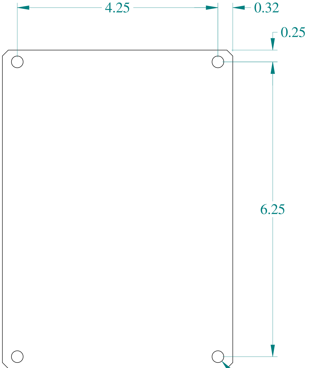
FRONT VIEW
