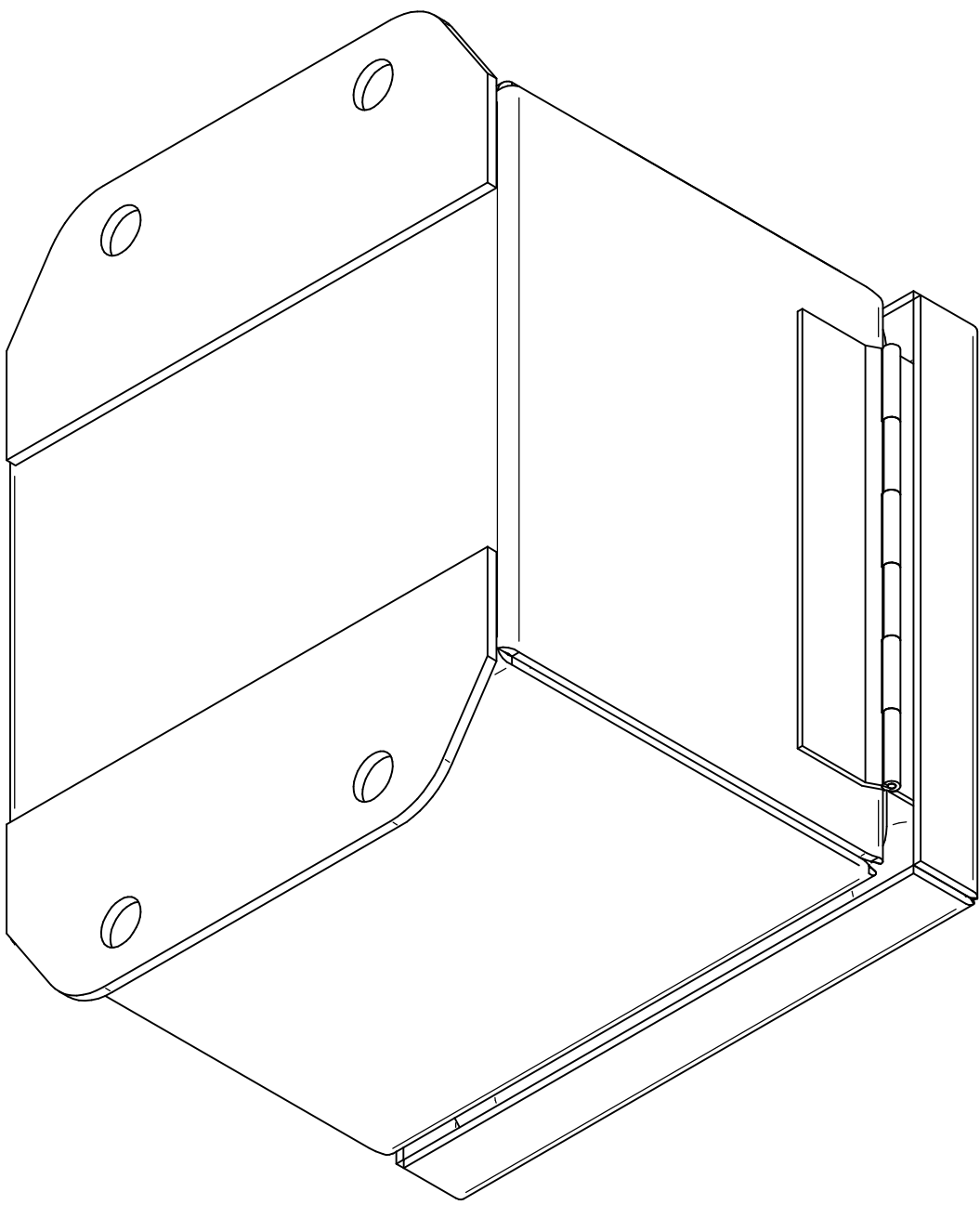
ISOMETRIC VIEWS
