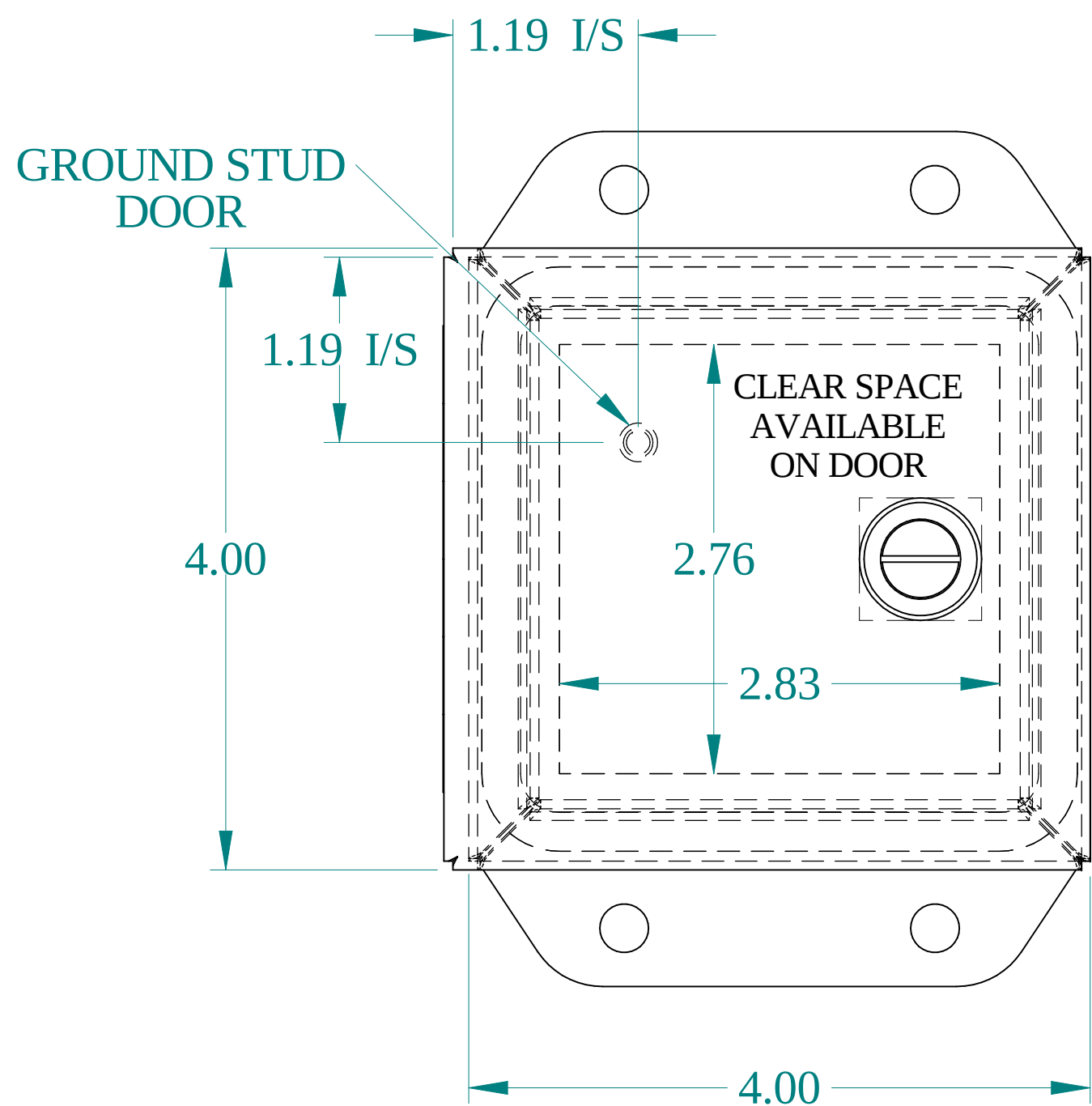
FRONT VIEW
