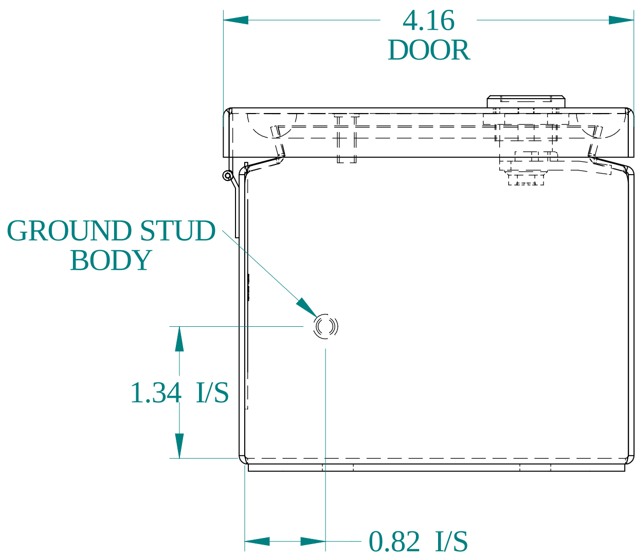
BOTTOM VIEW
