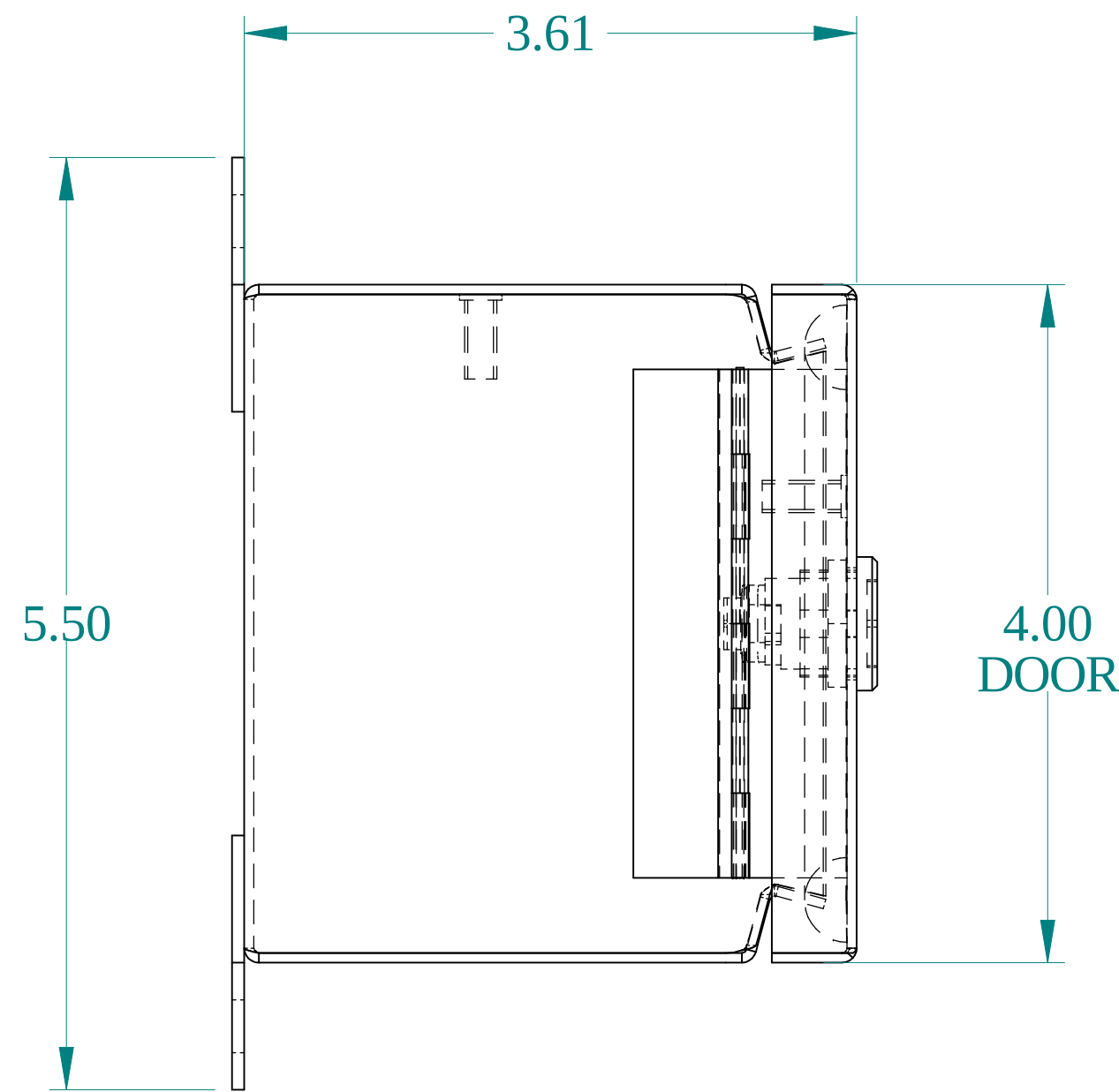
SIDE VIEW
