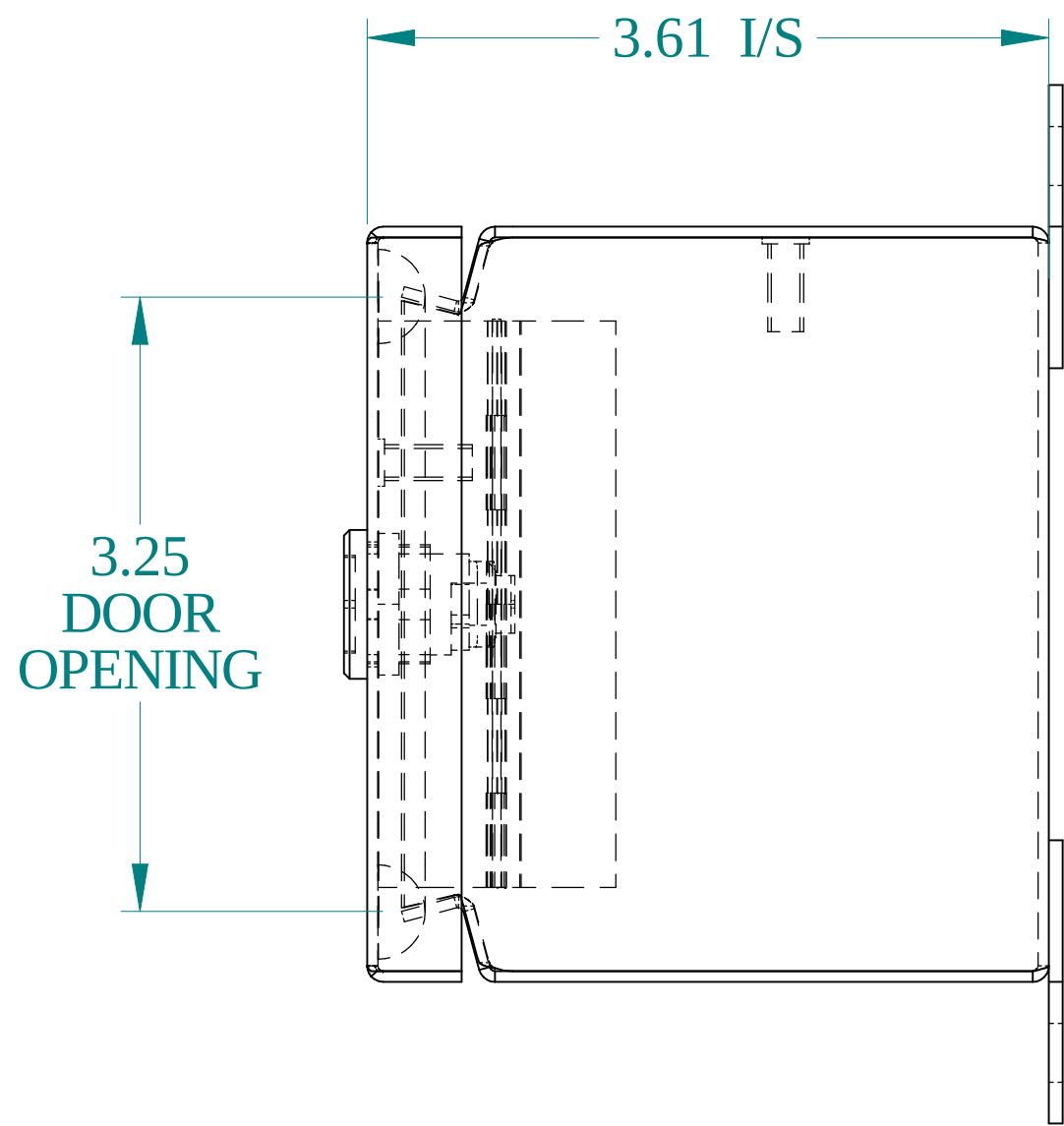
SIDE VIEW
