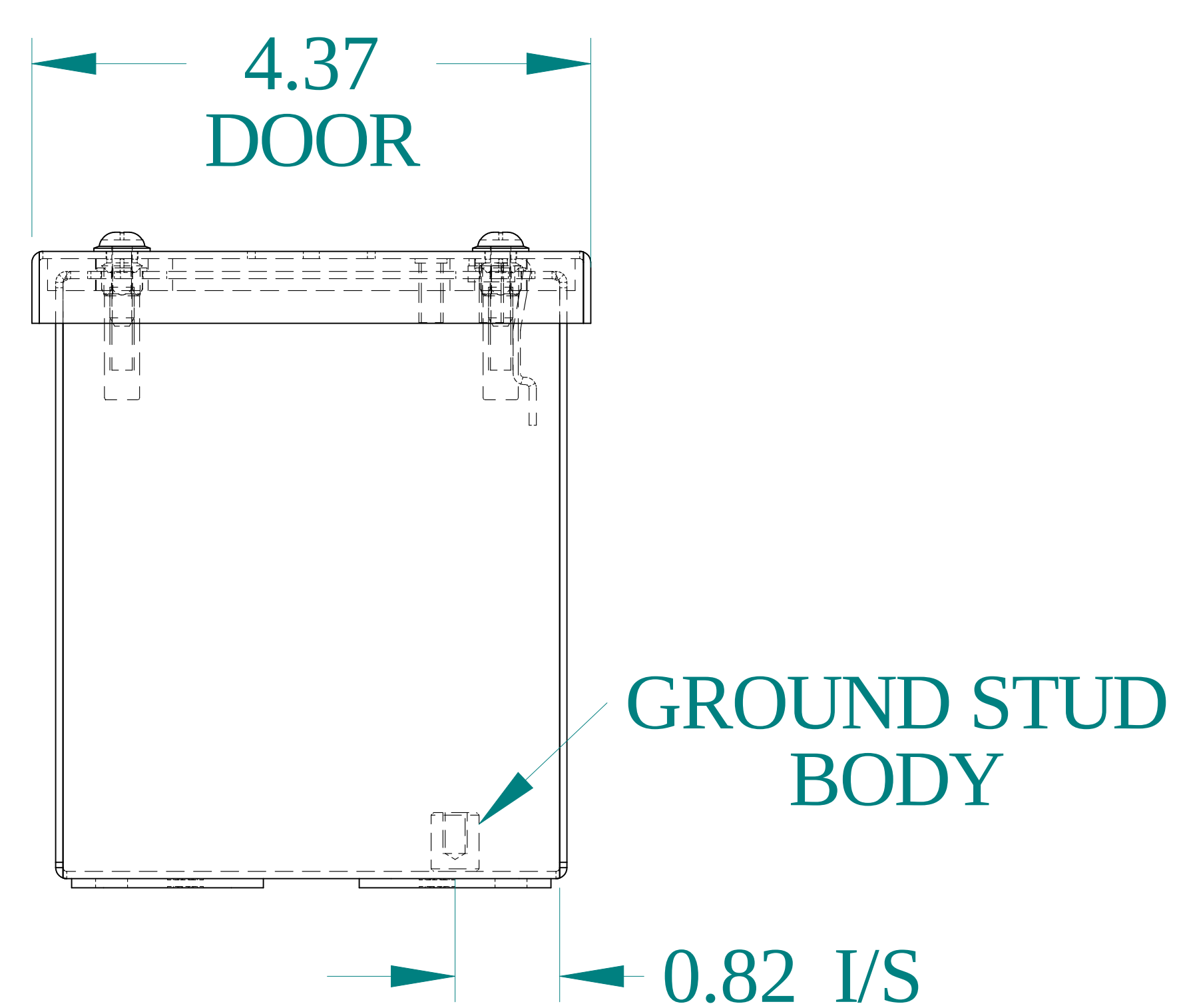
BOTTOM VIEW
