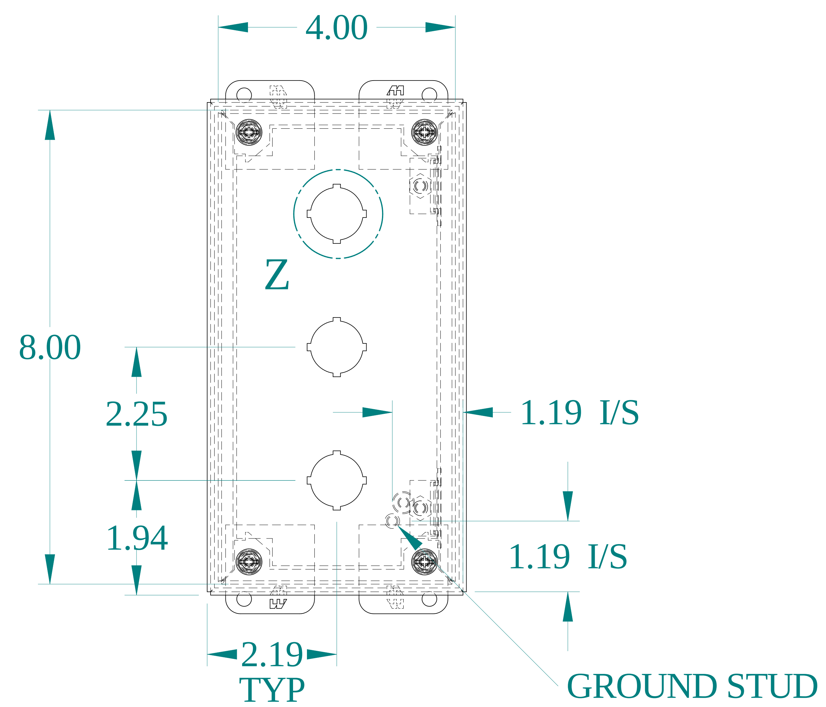
FRONT VIEW
