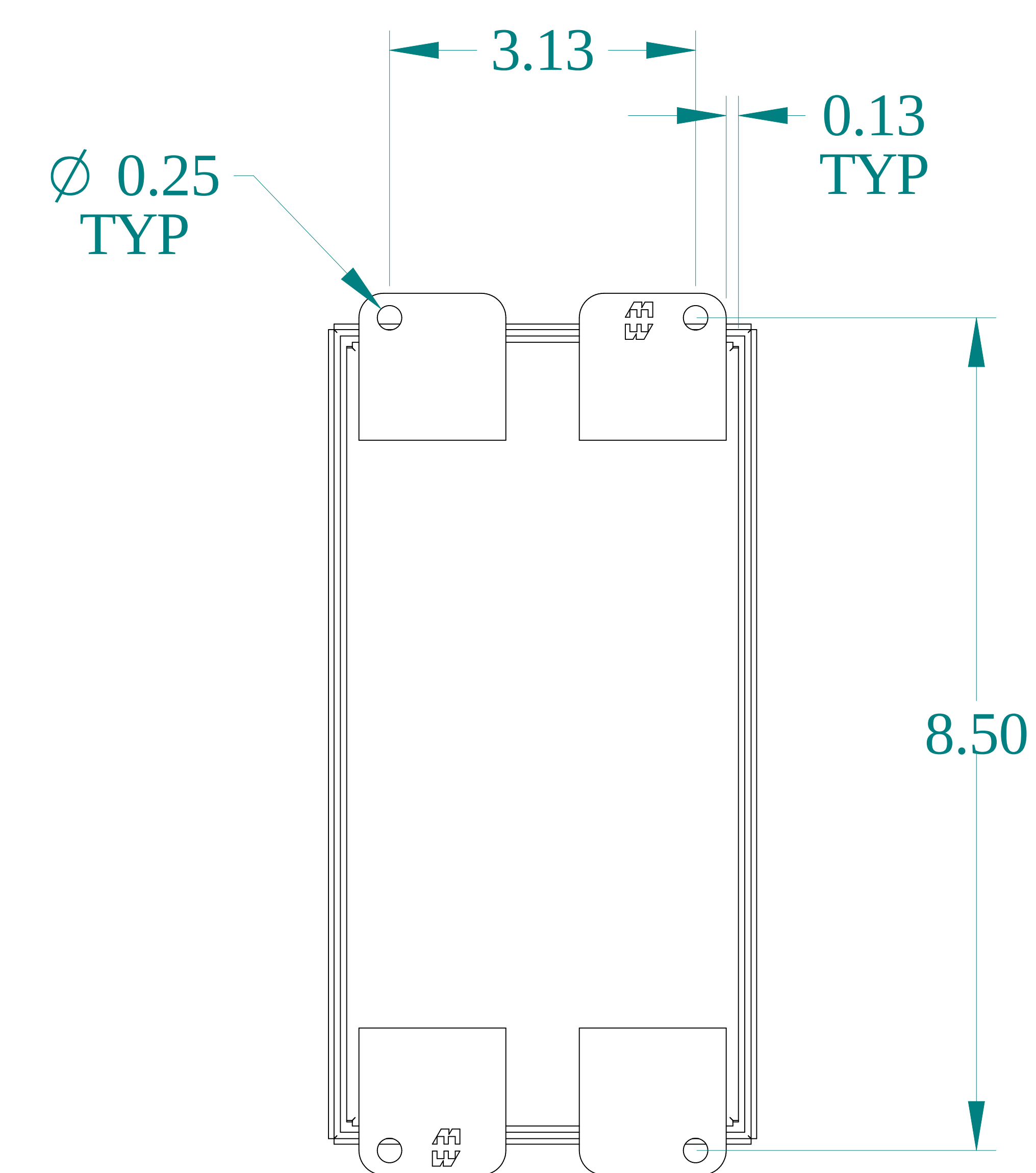
BACK VIEW
