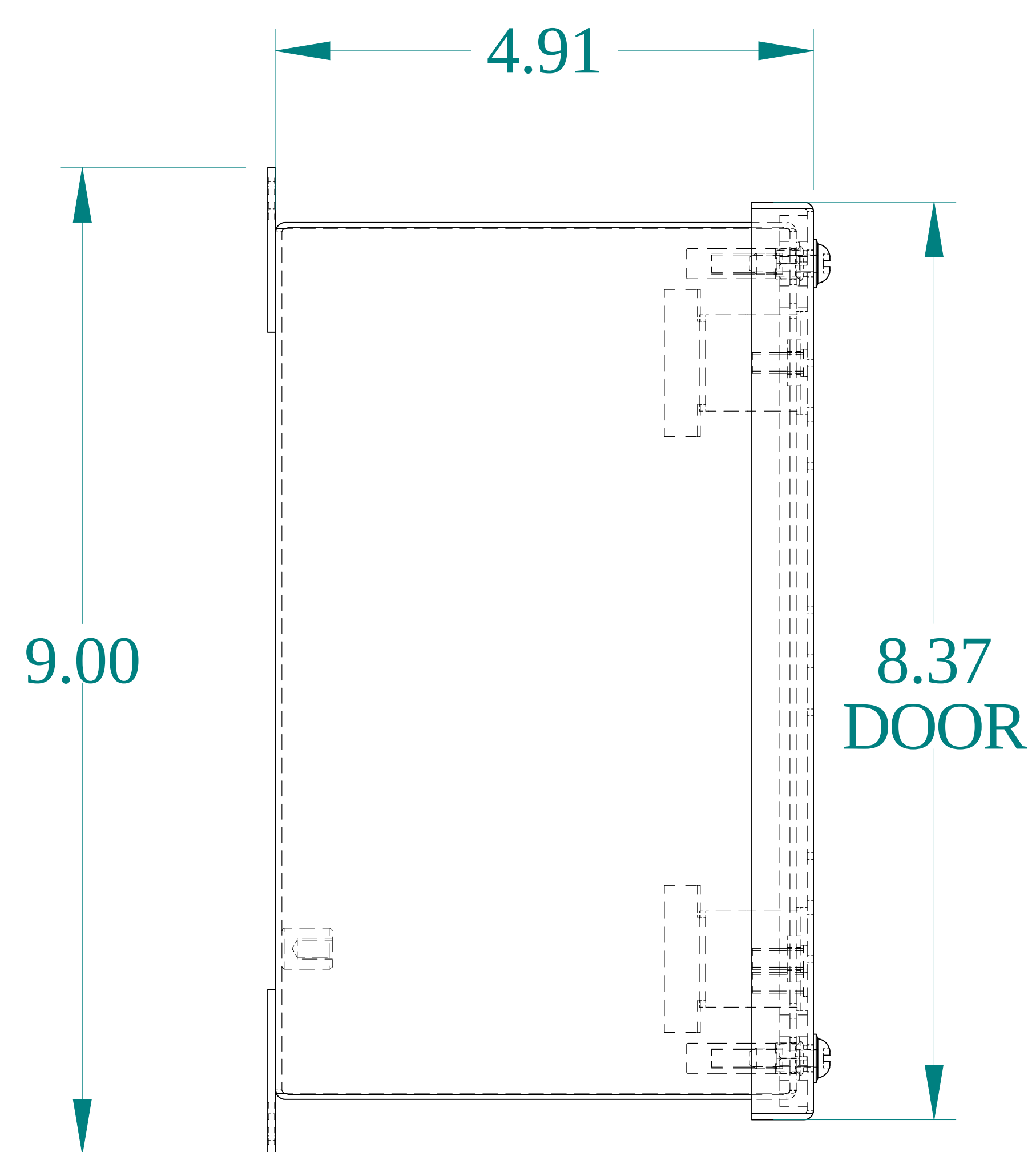
SIDE VIEW
