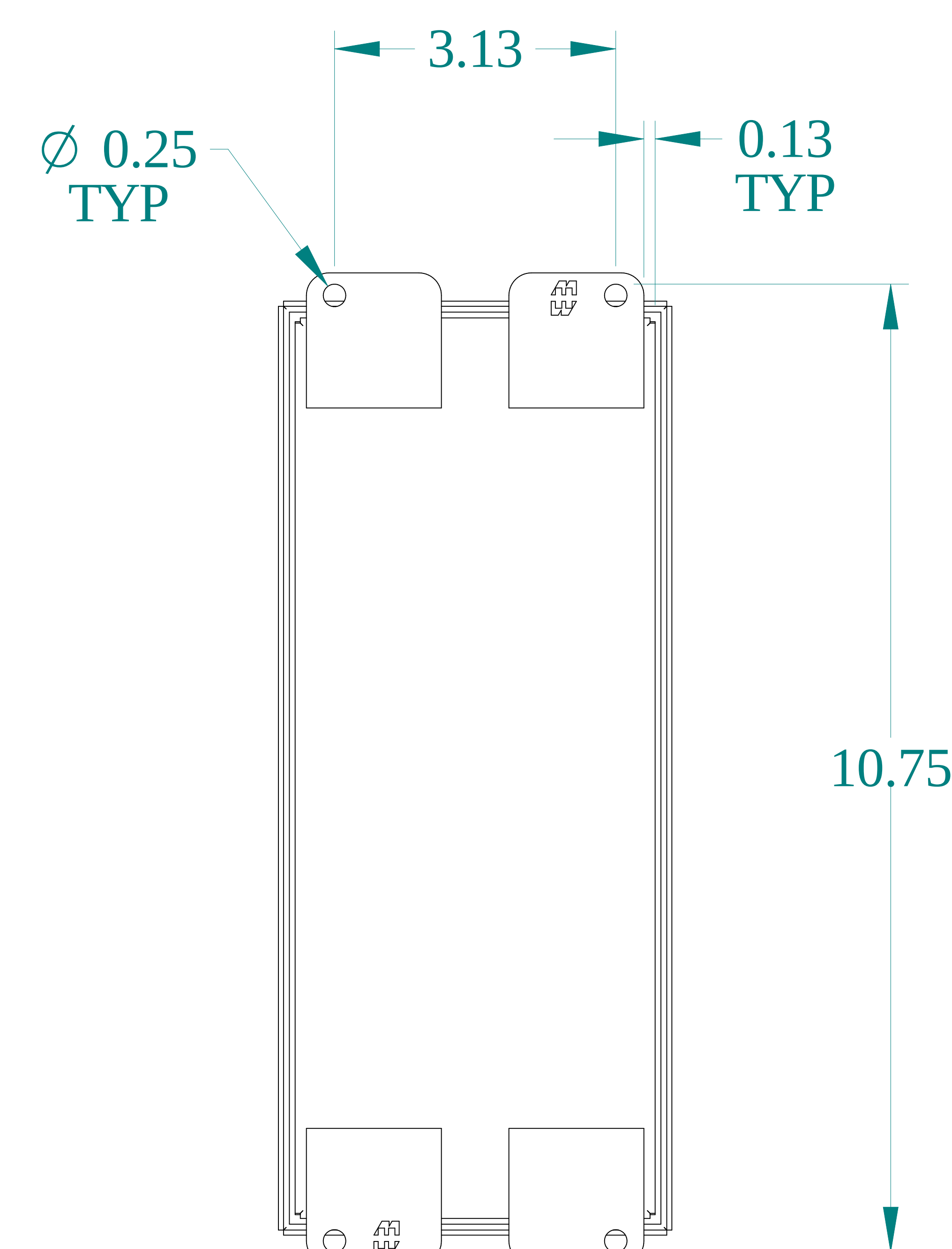
BACK VIEW
