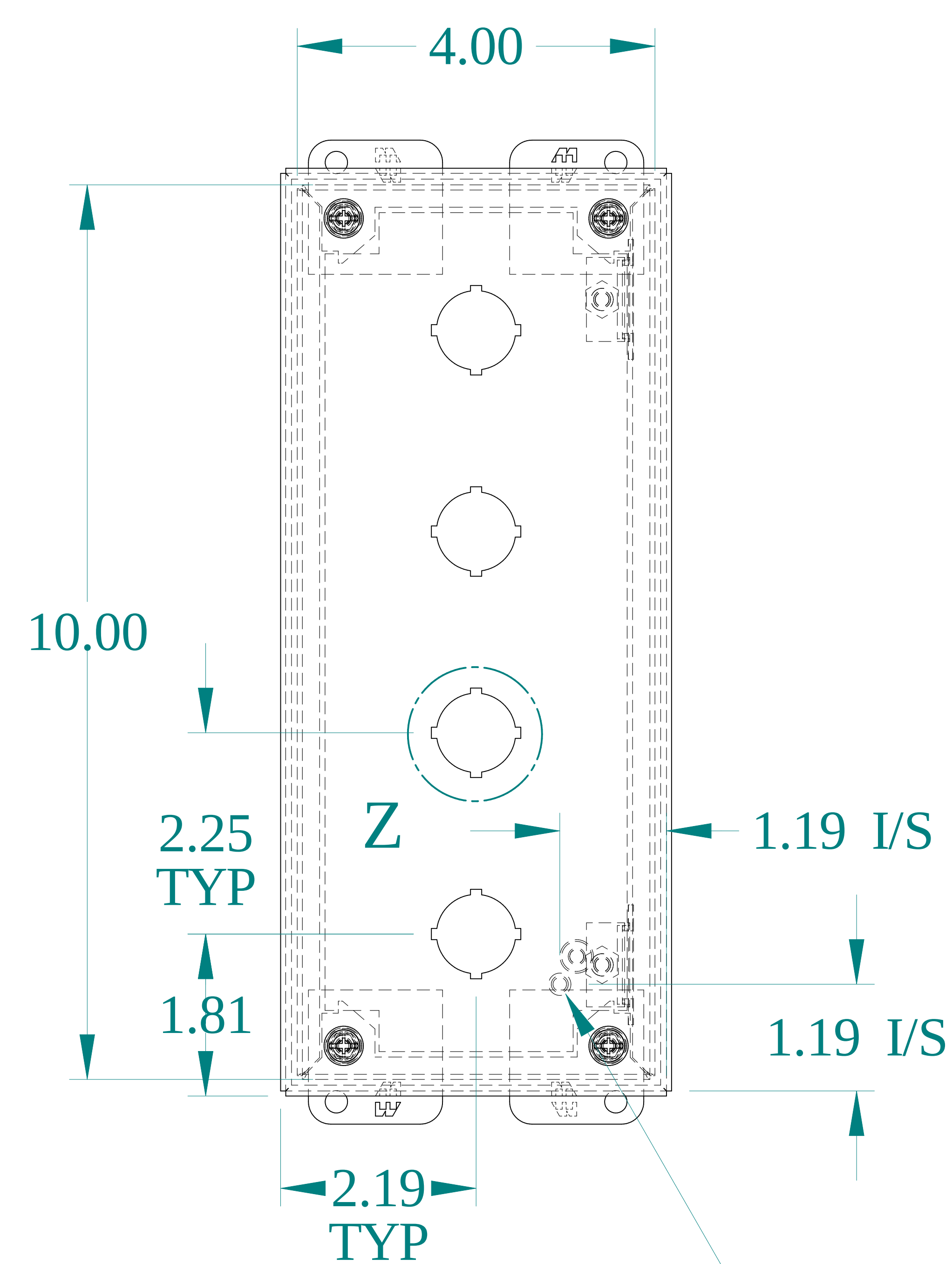
FRONT VIEW
