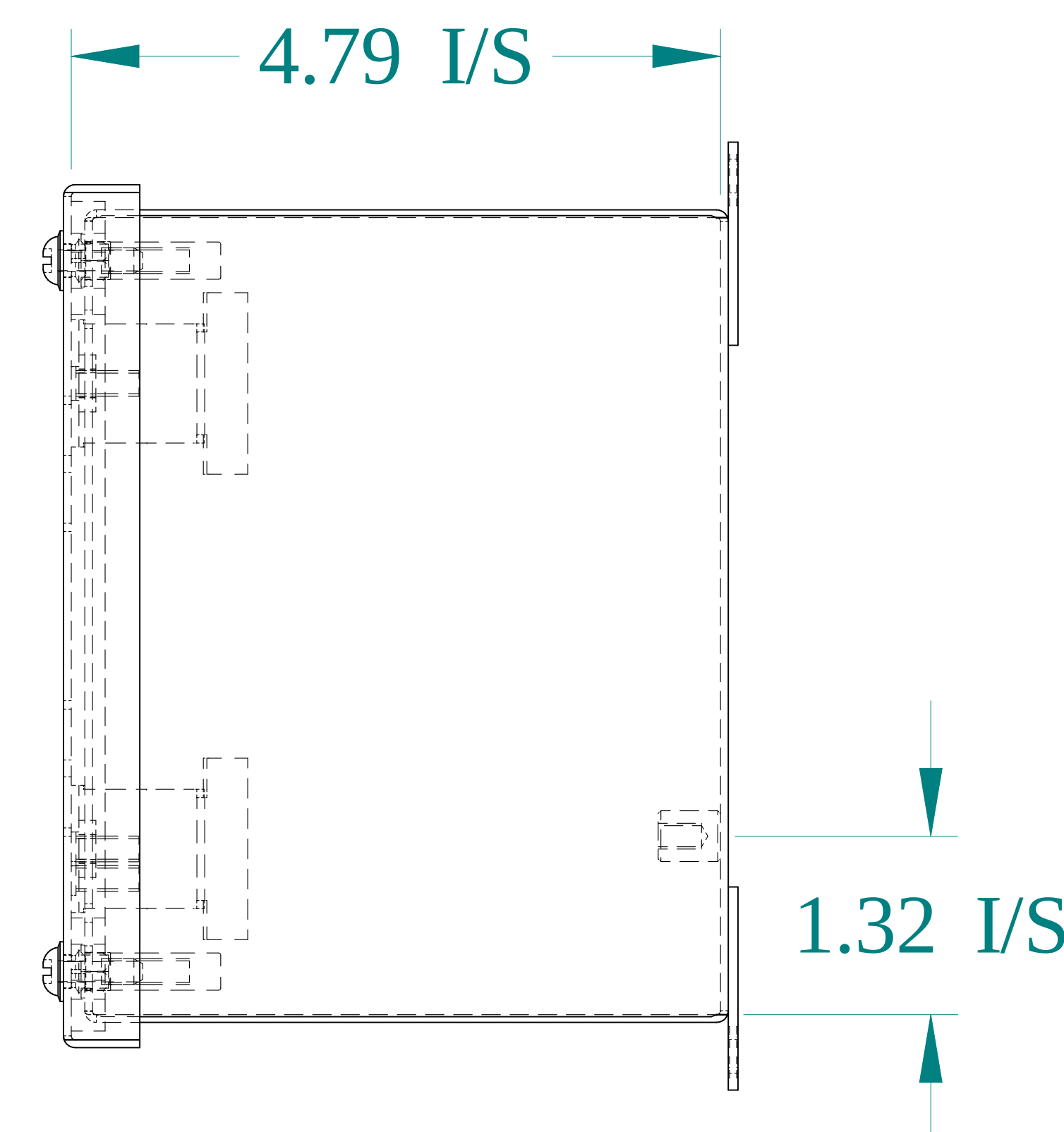
SIDE VIEW
