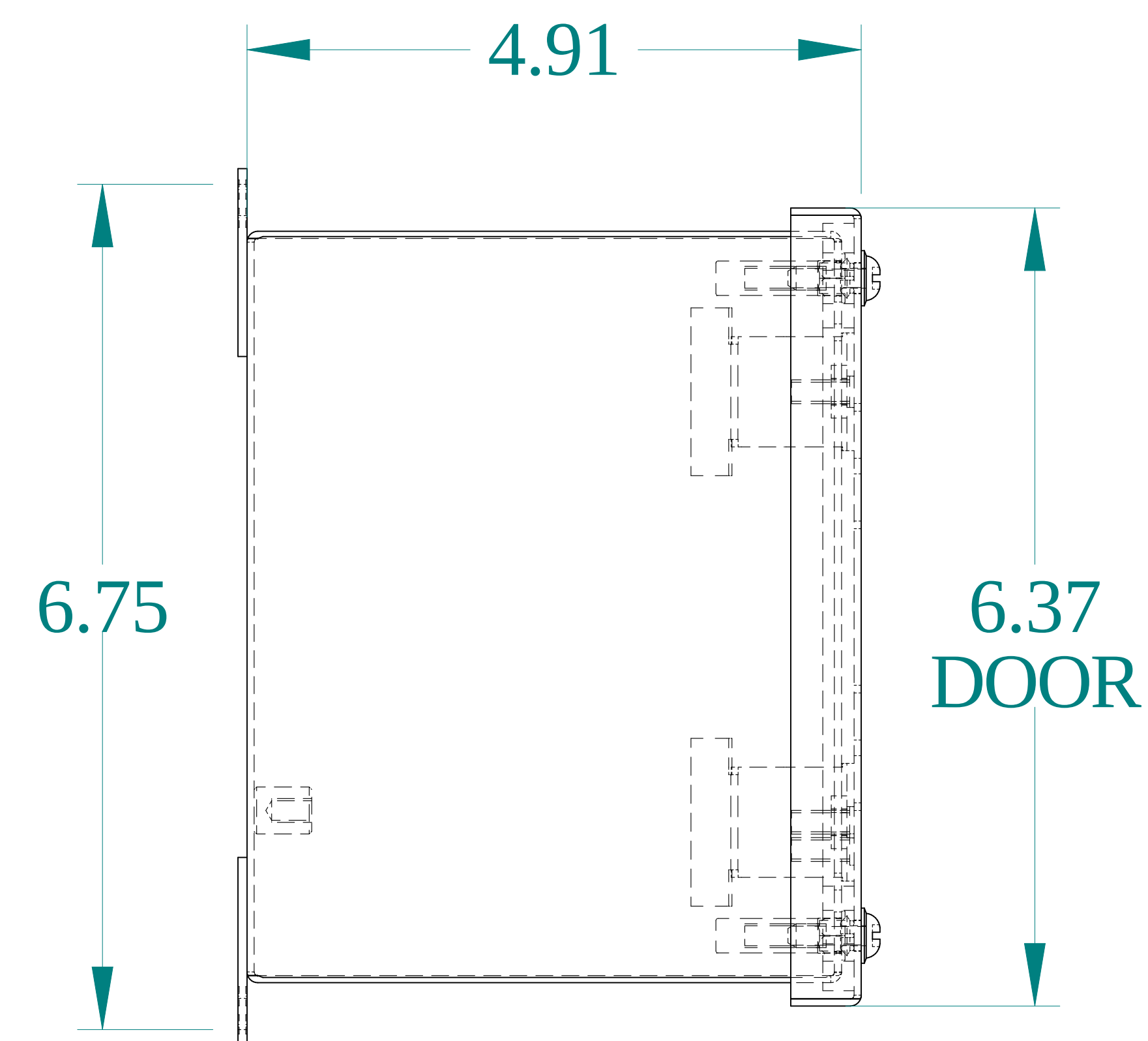
SIDE VIEW
