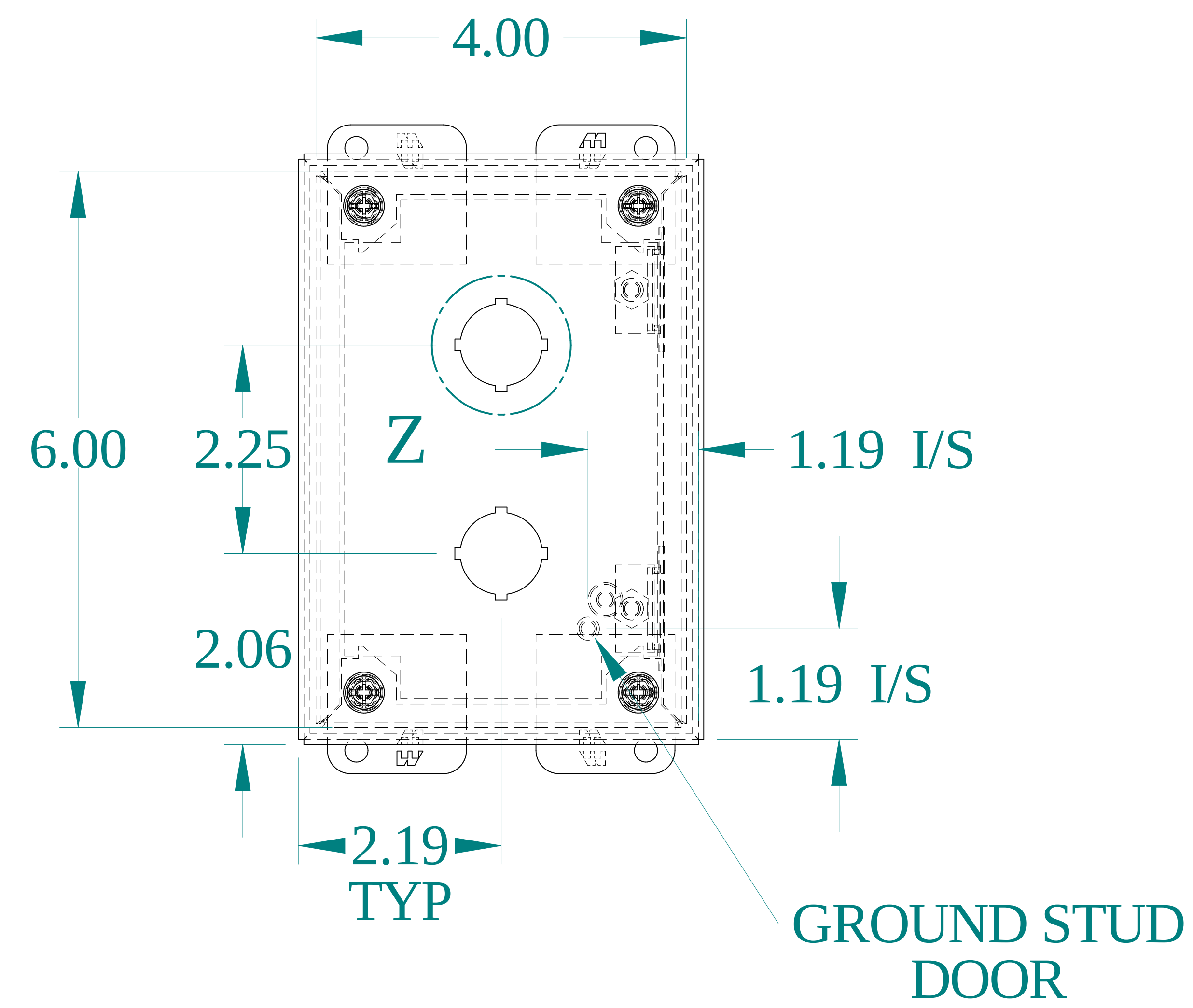
FRONT VIEW
