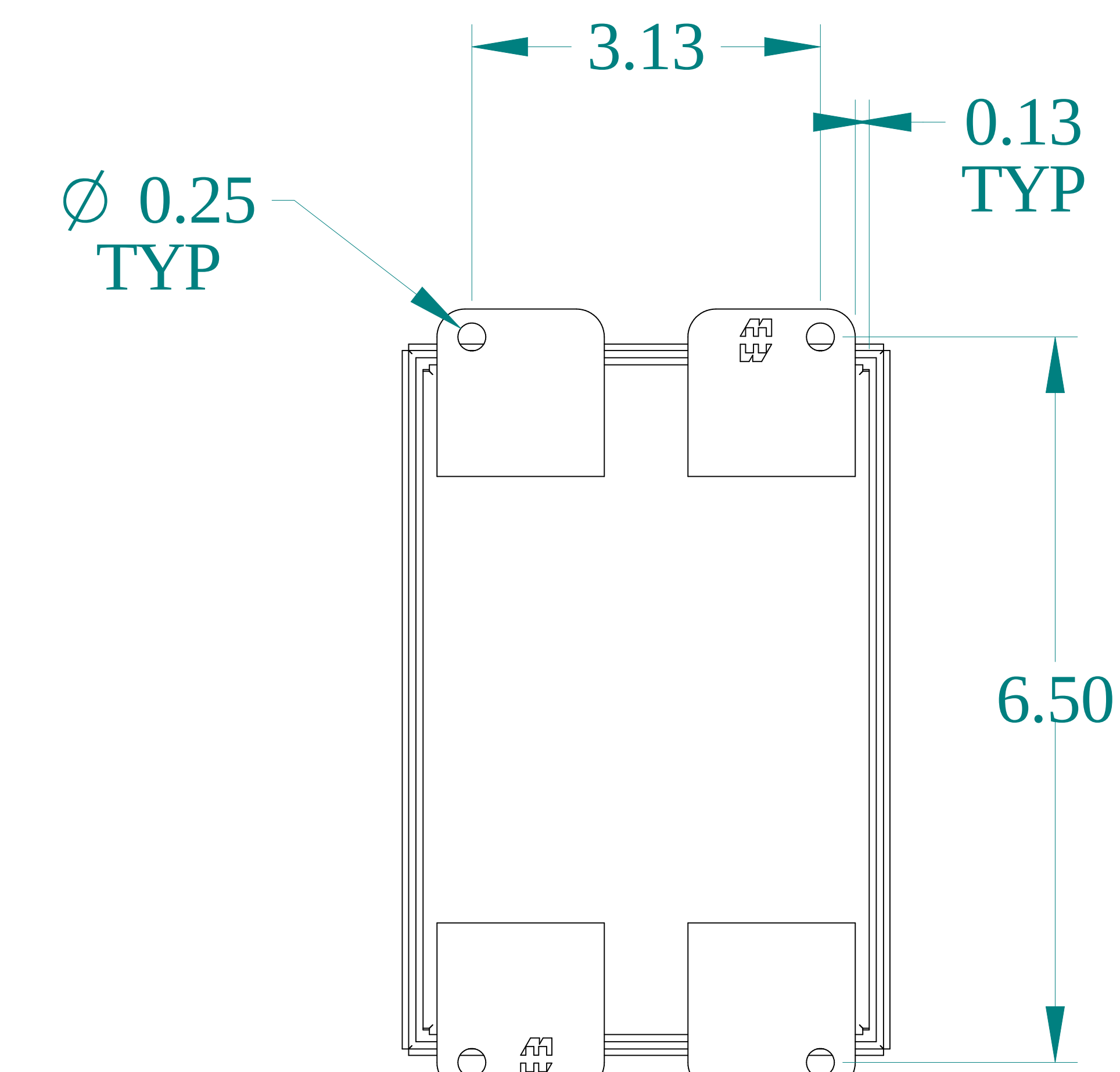
BACK VIEW
