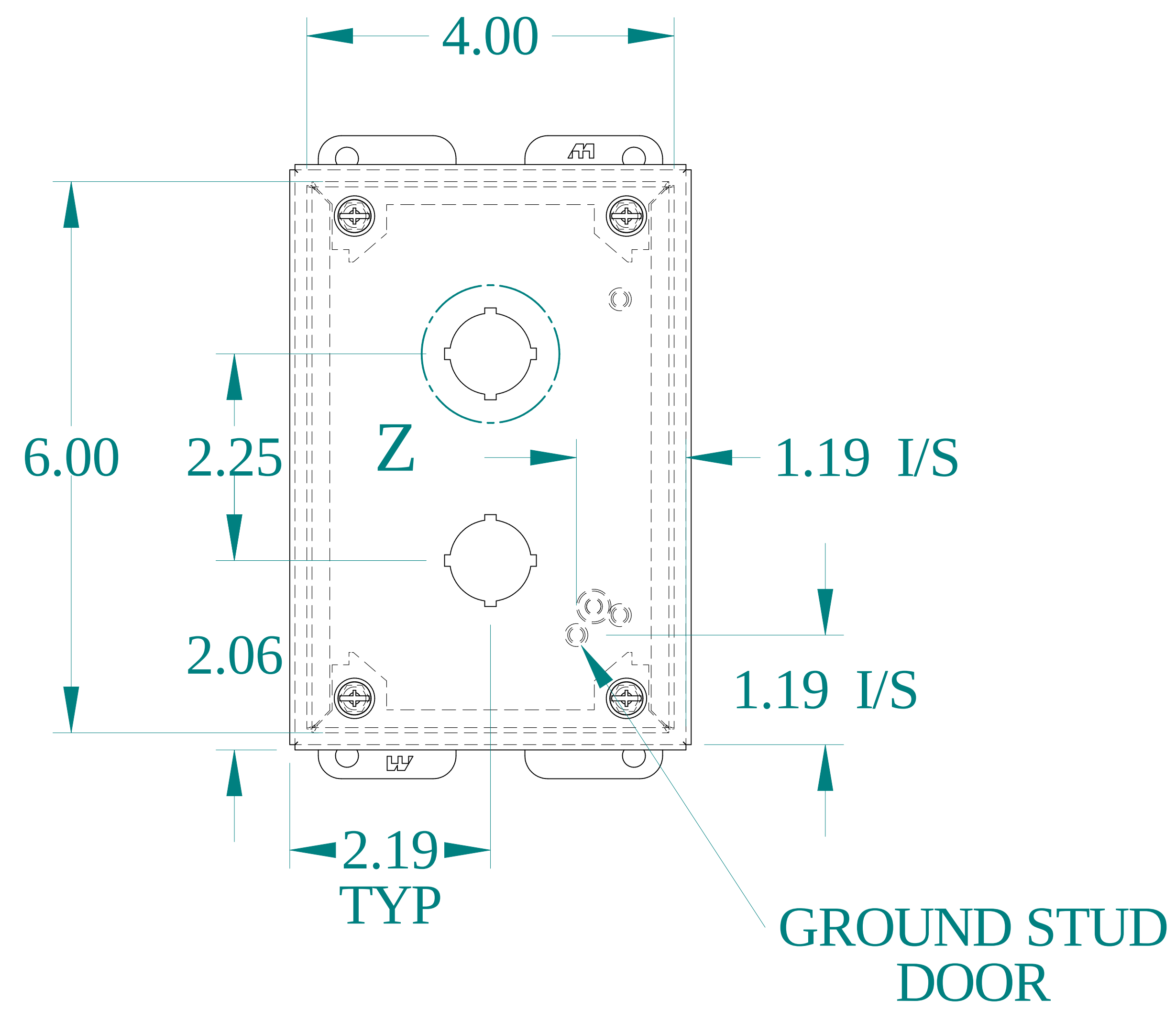
FRONT VIEW
