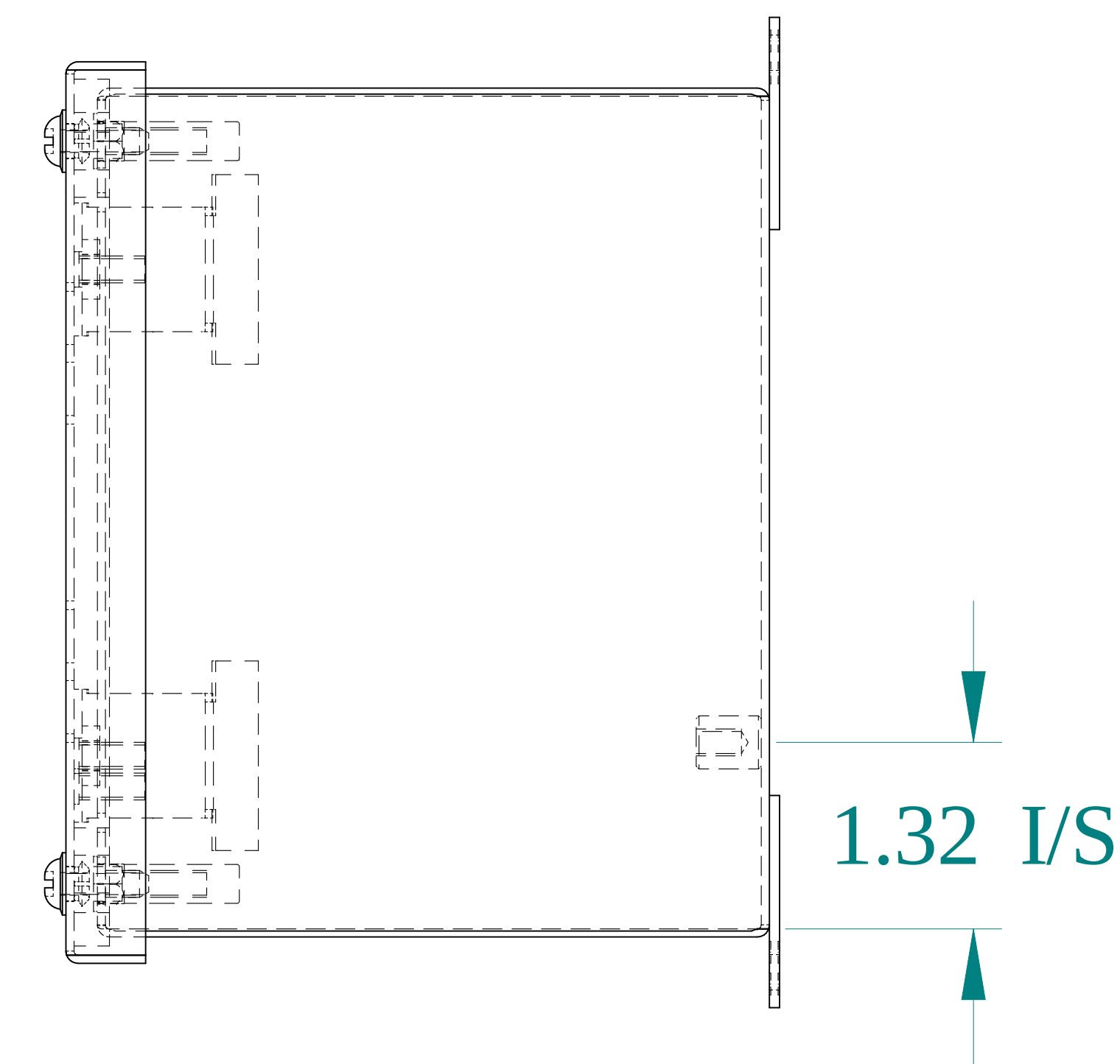
SIDE VIEW
