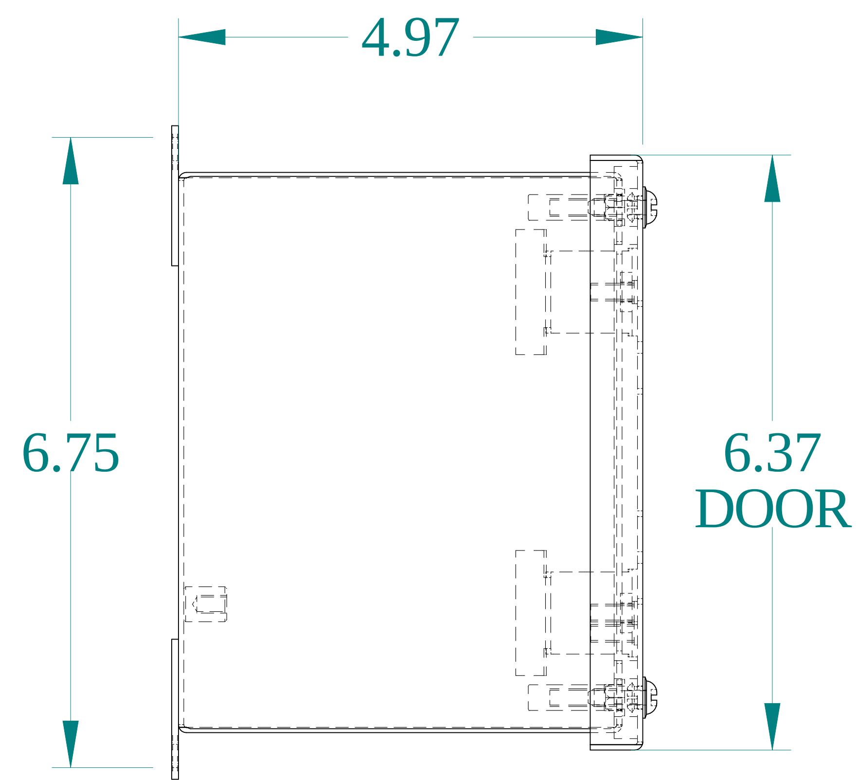
SIDE VIEW
