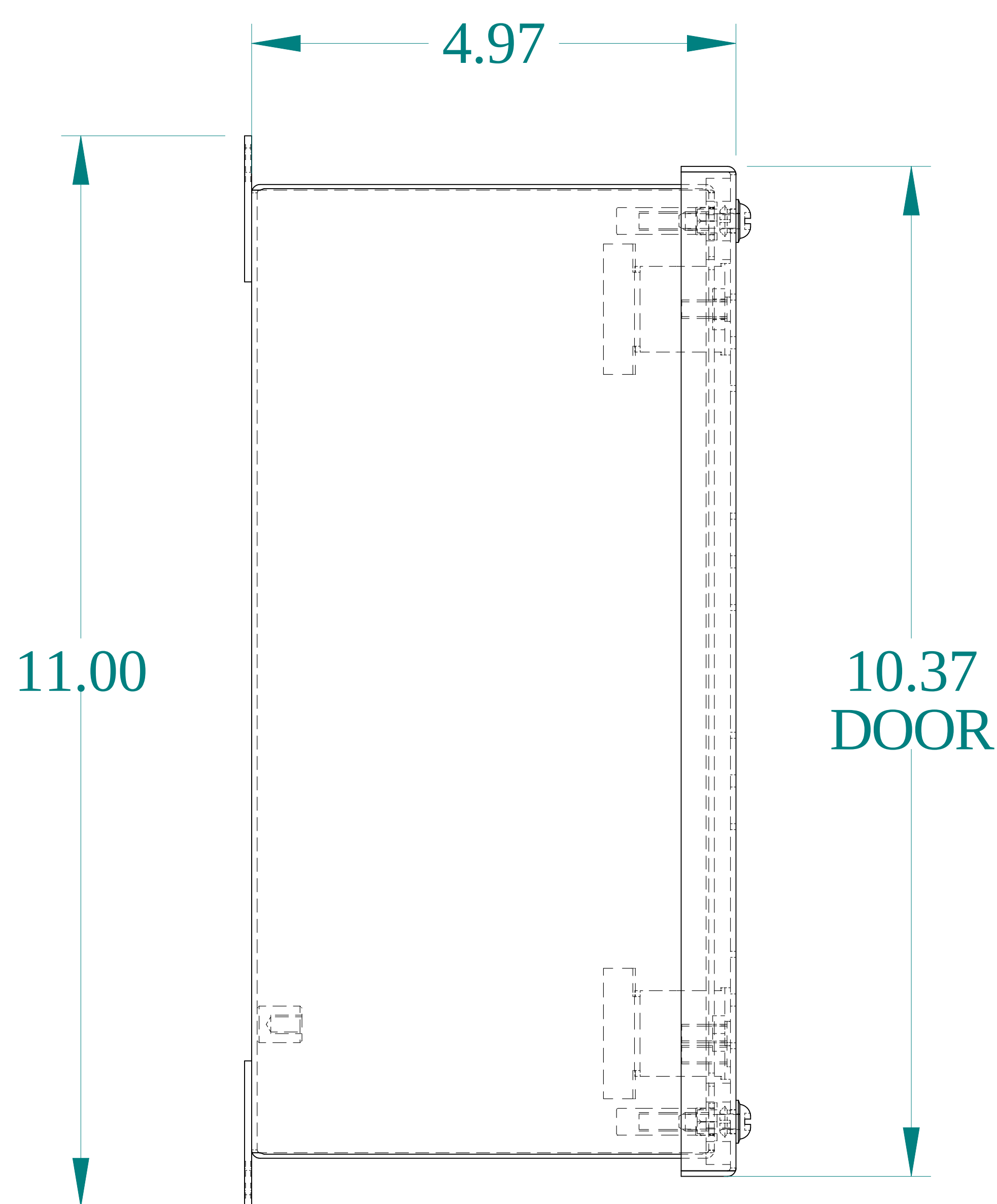
SIDE VIEW
