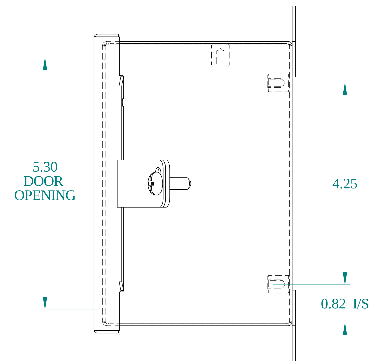
SIDE VIEW
