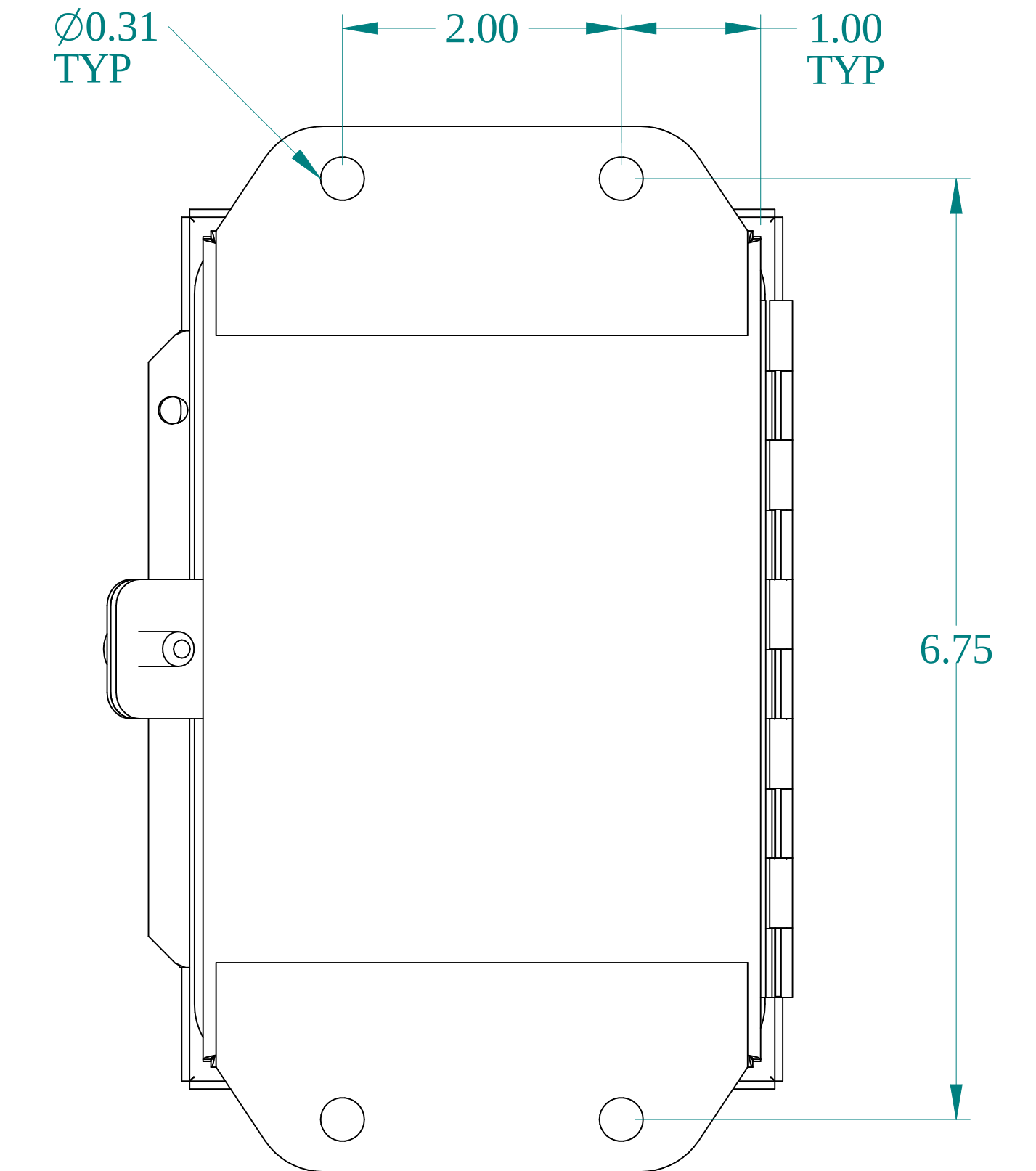
BACK VIEW
