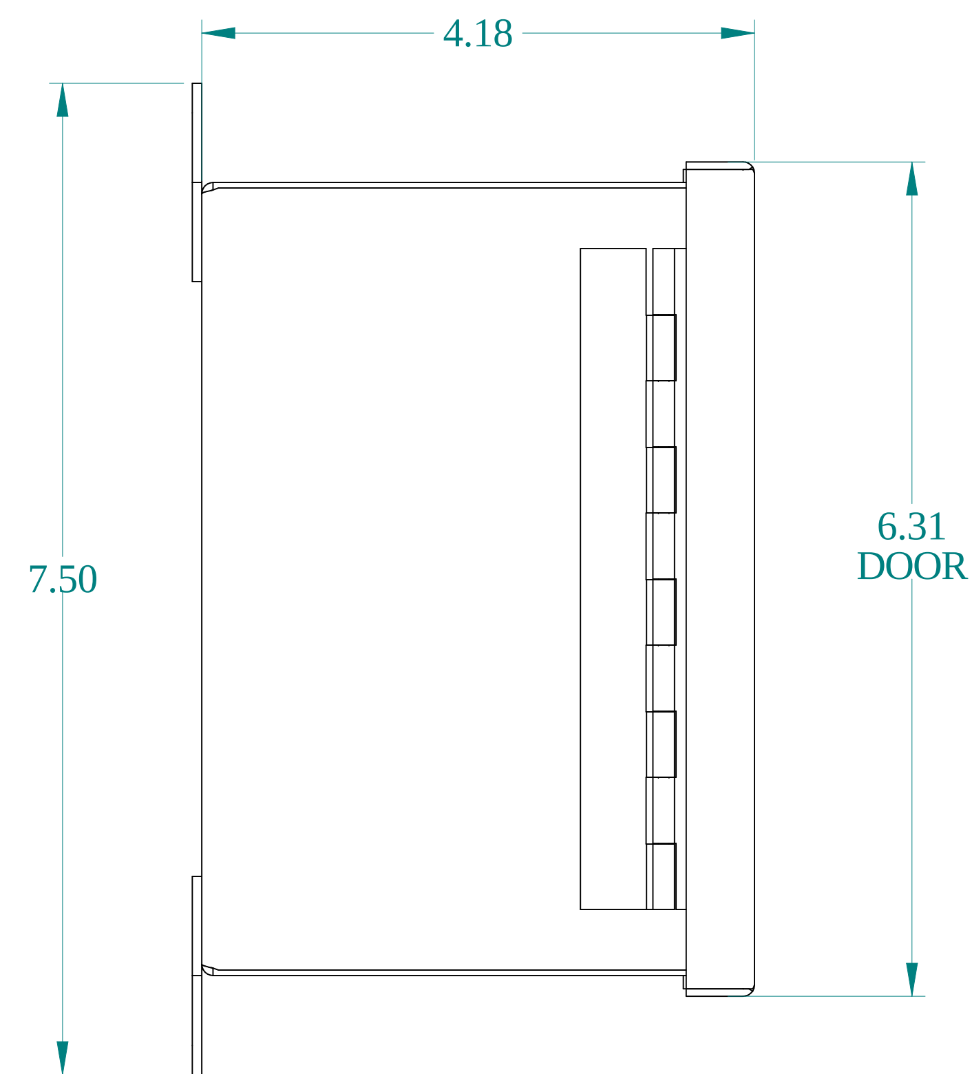
SIDE VIEW
