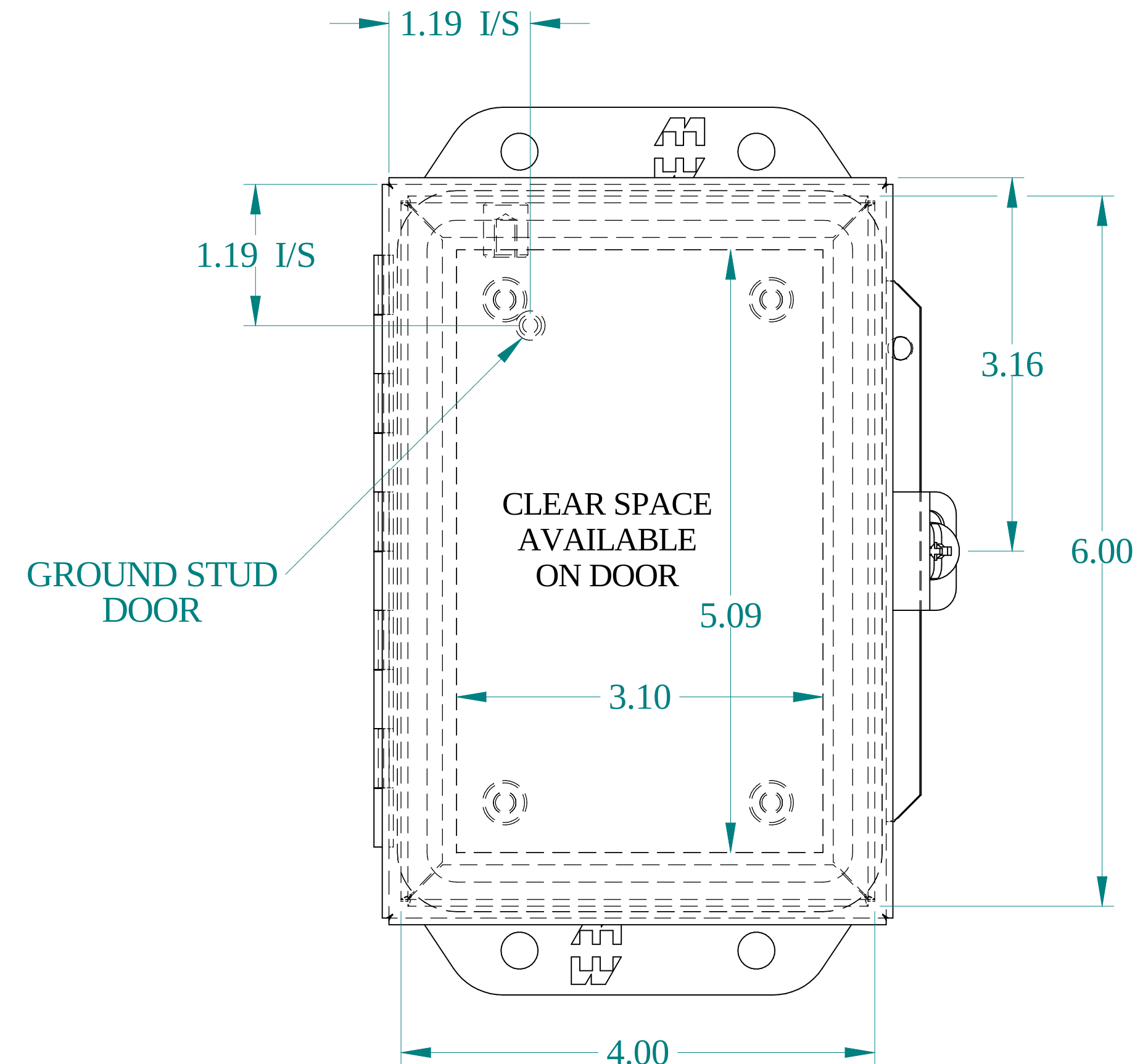
FRONT VIEW
