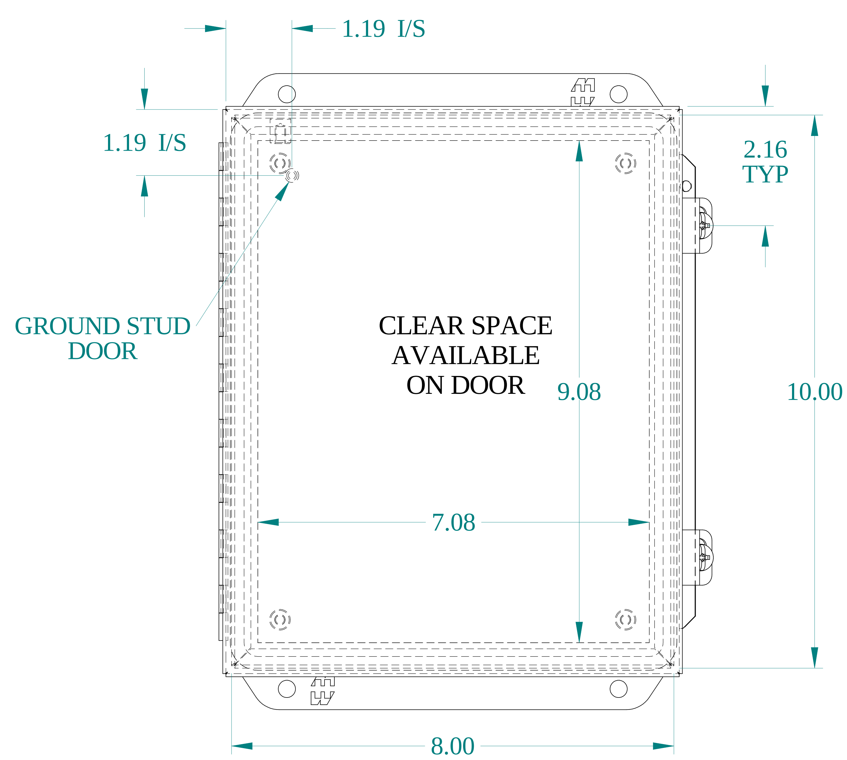
FRONT VIEW
