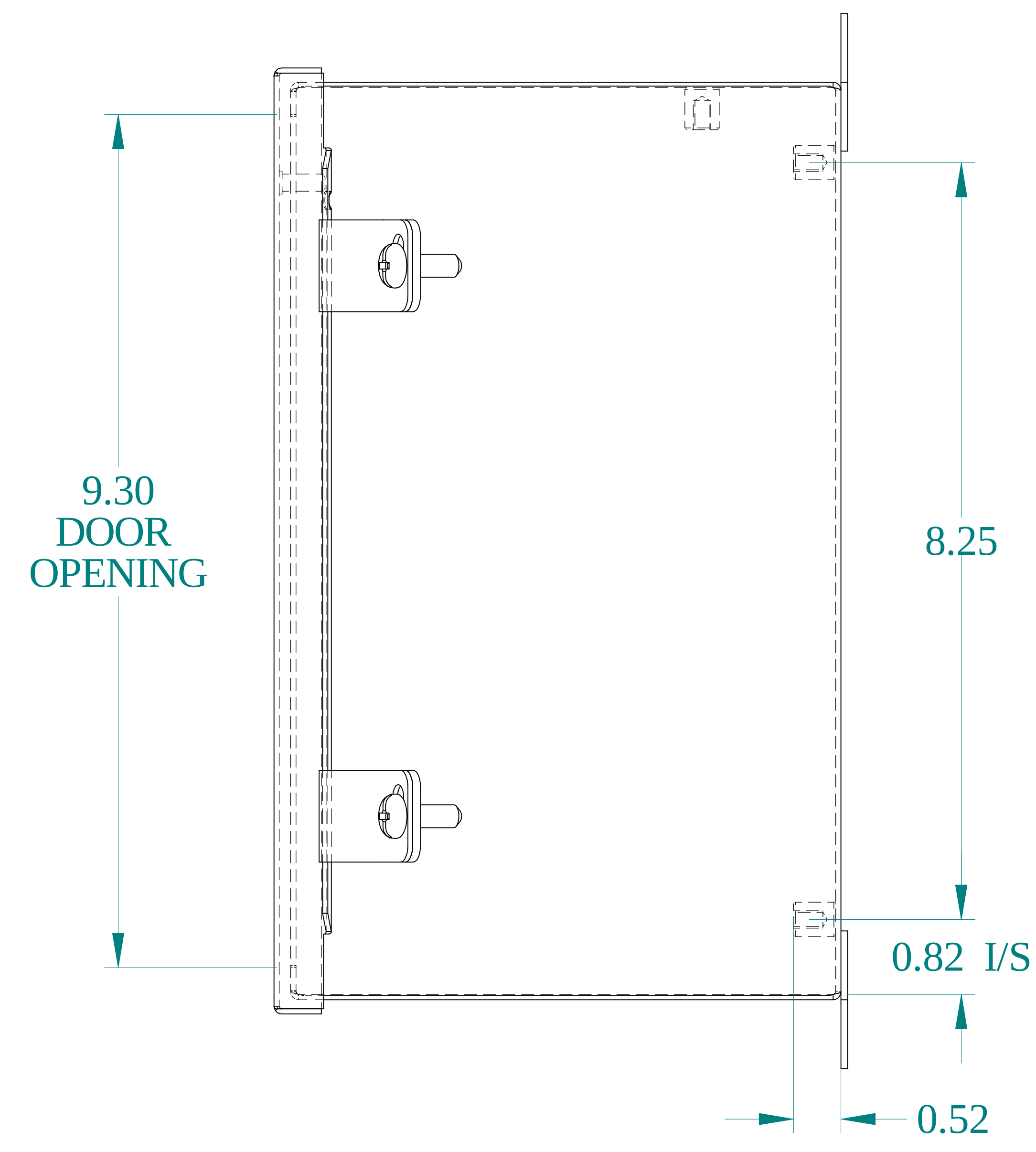
SIDE VIEW
