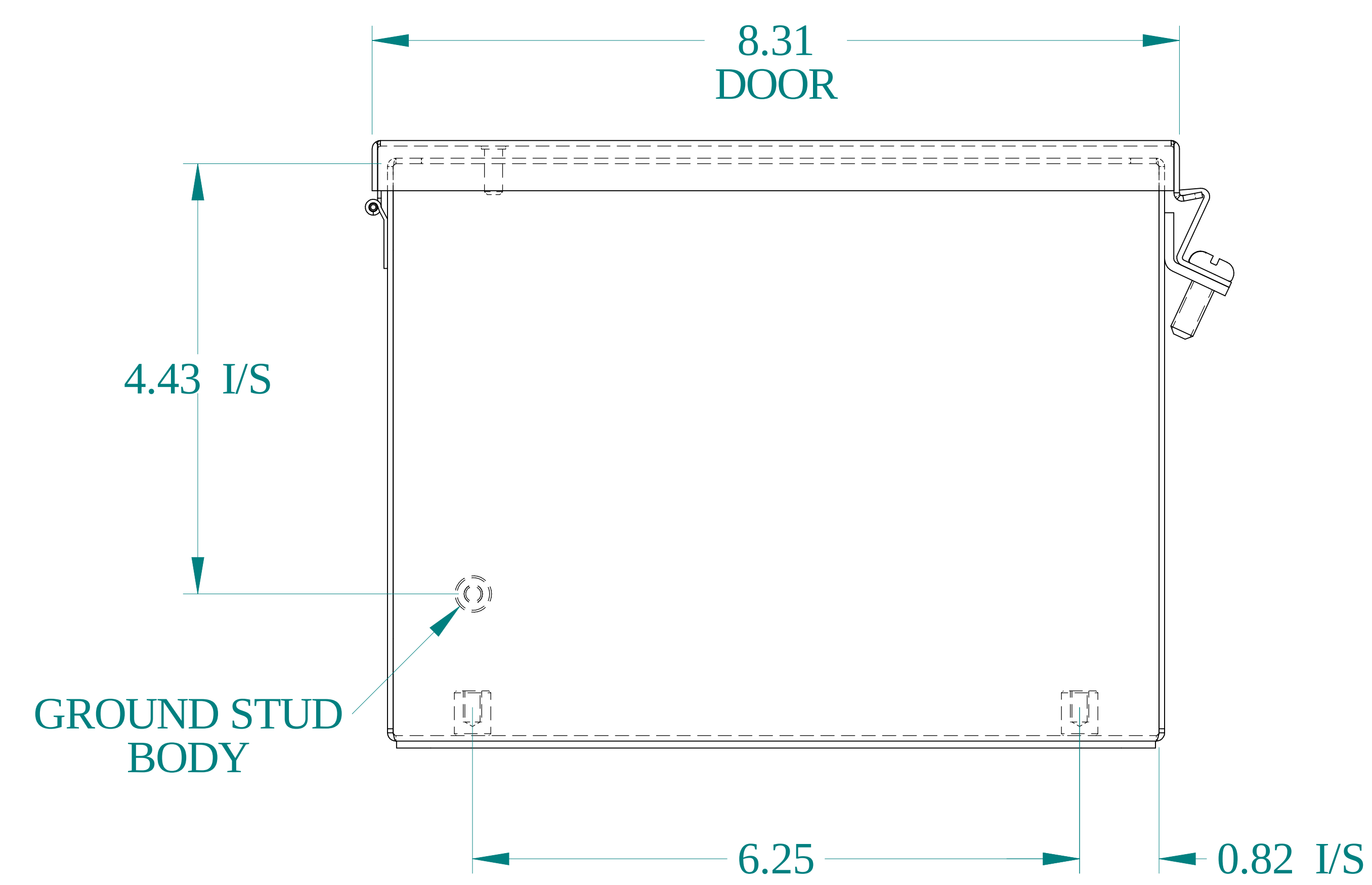
BOTTOM VIEW
