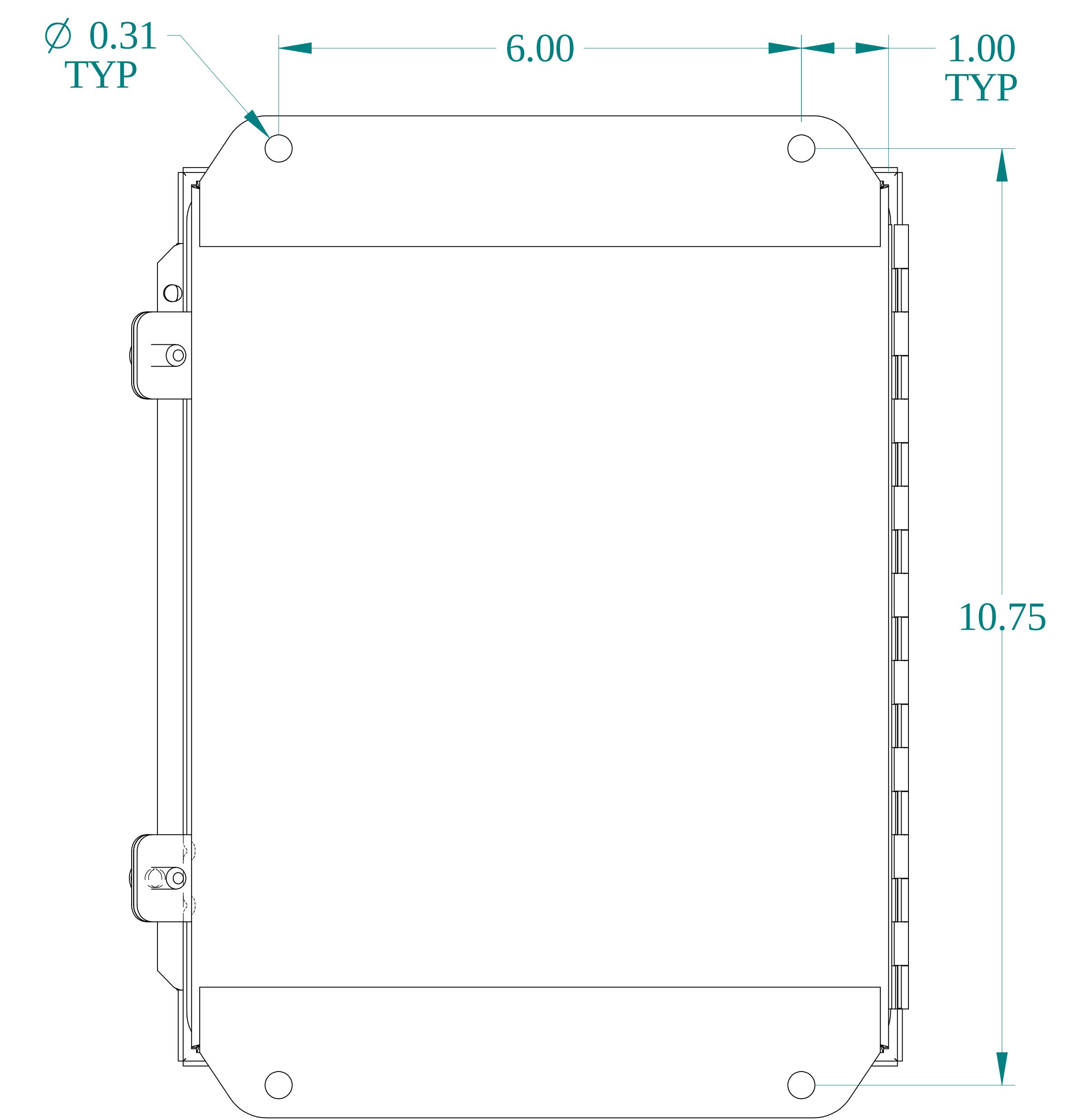
BACK VIEW
