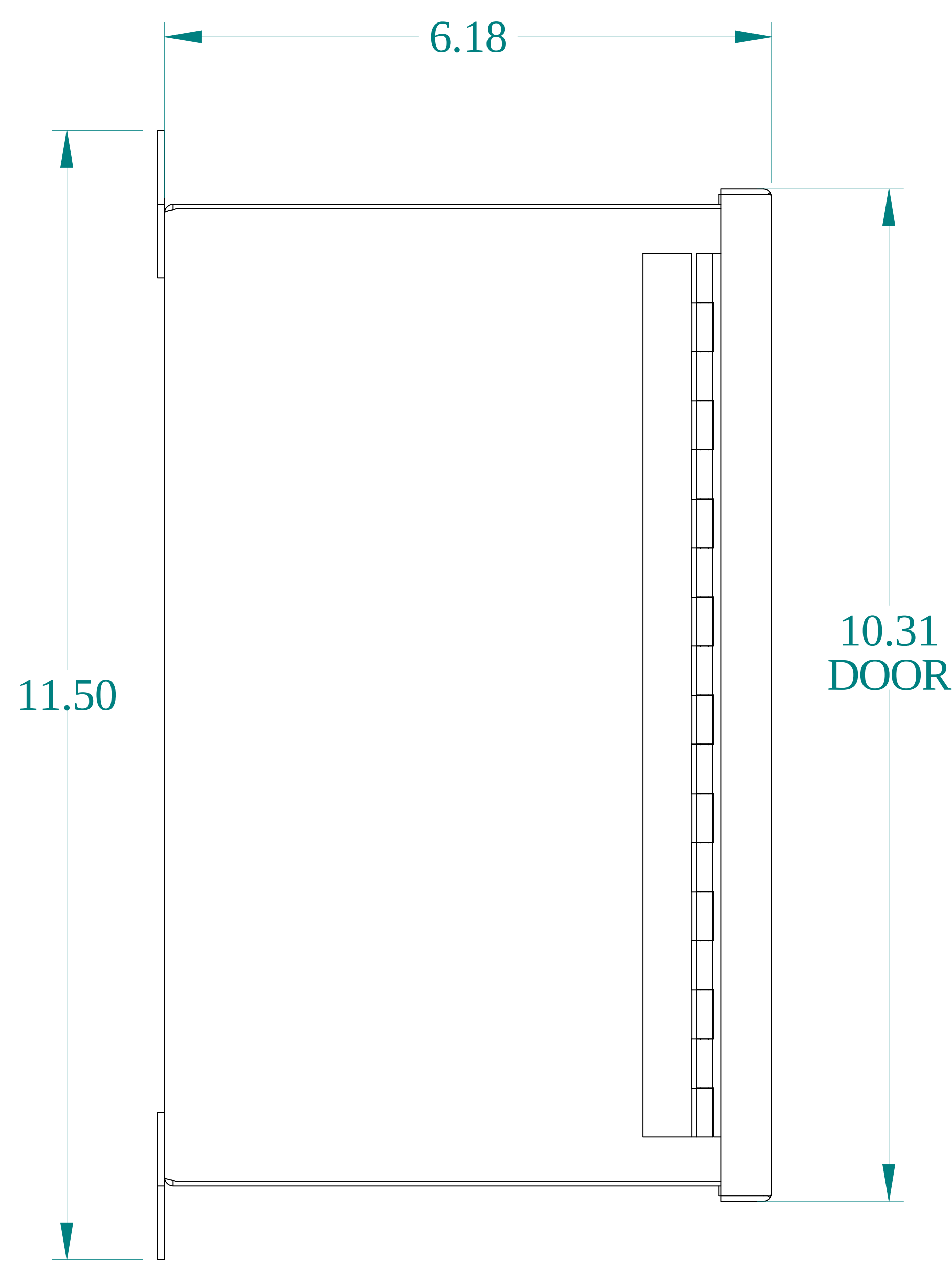
SIDE VIEW
