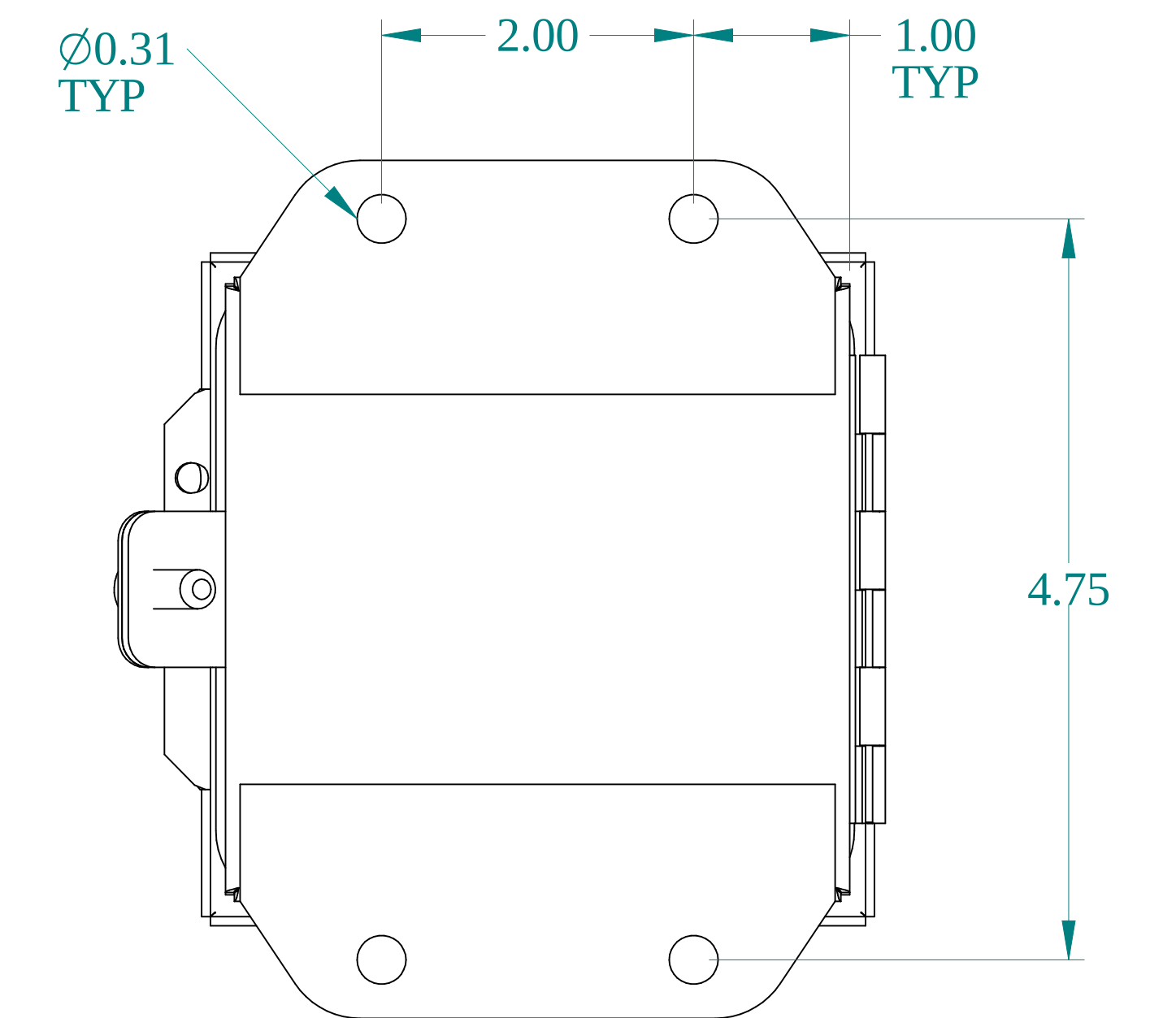
BACK VIEW
