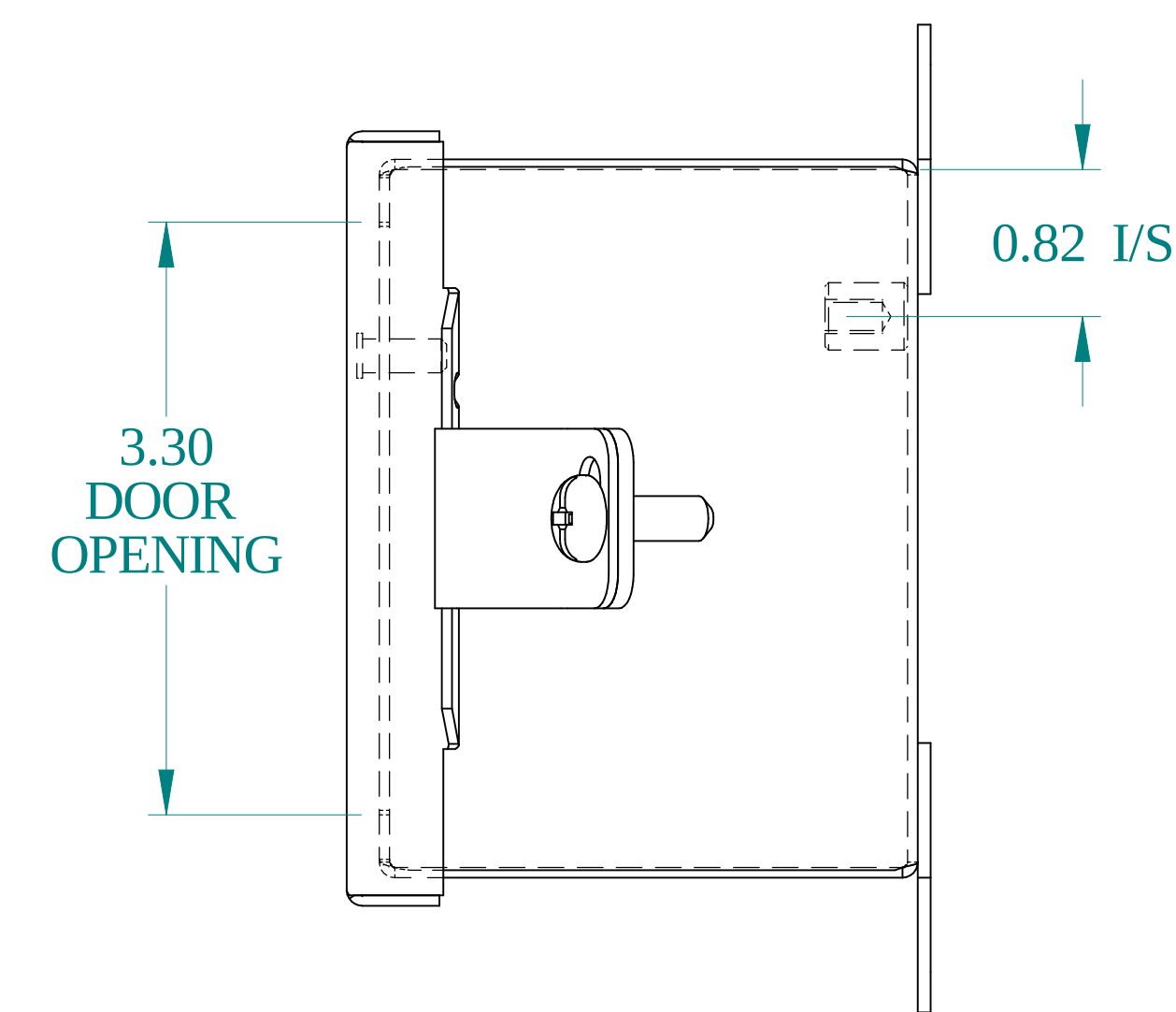
SIDE VIEW
