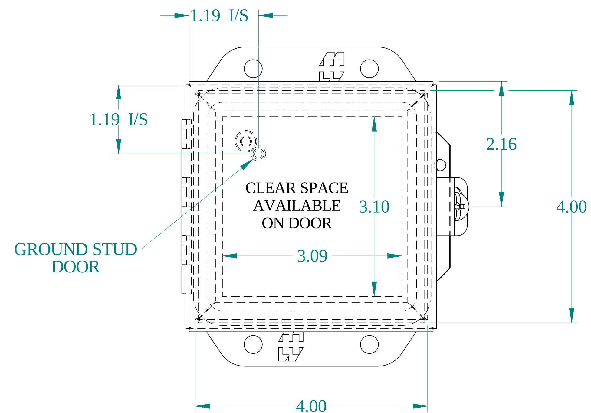
FRONT VIEW
