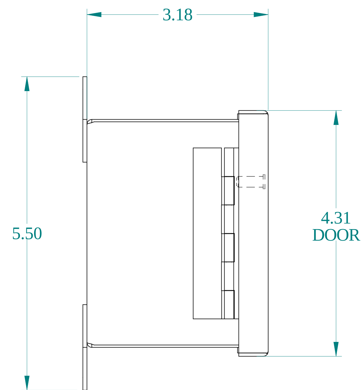
SIDE VIEW
