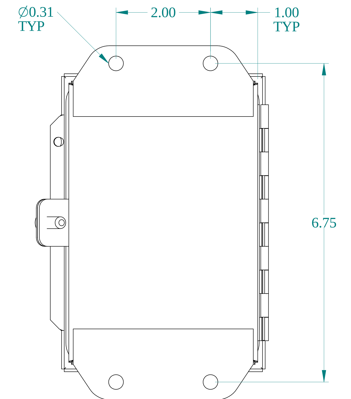
BACK VIEW
