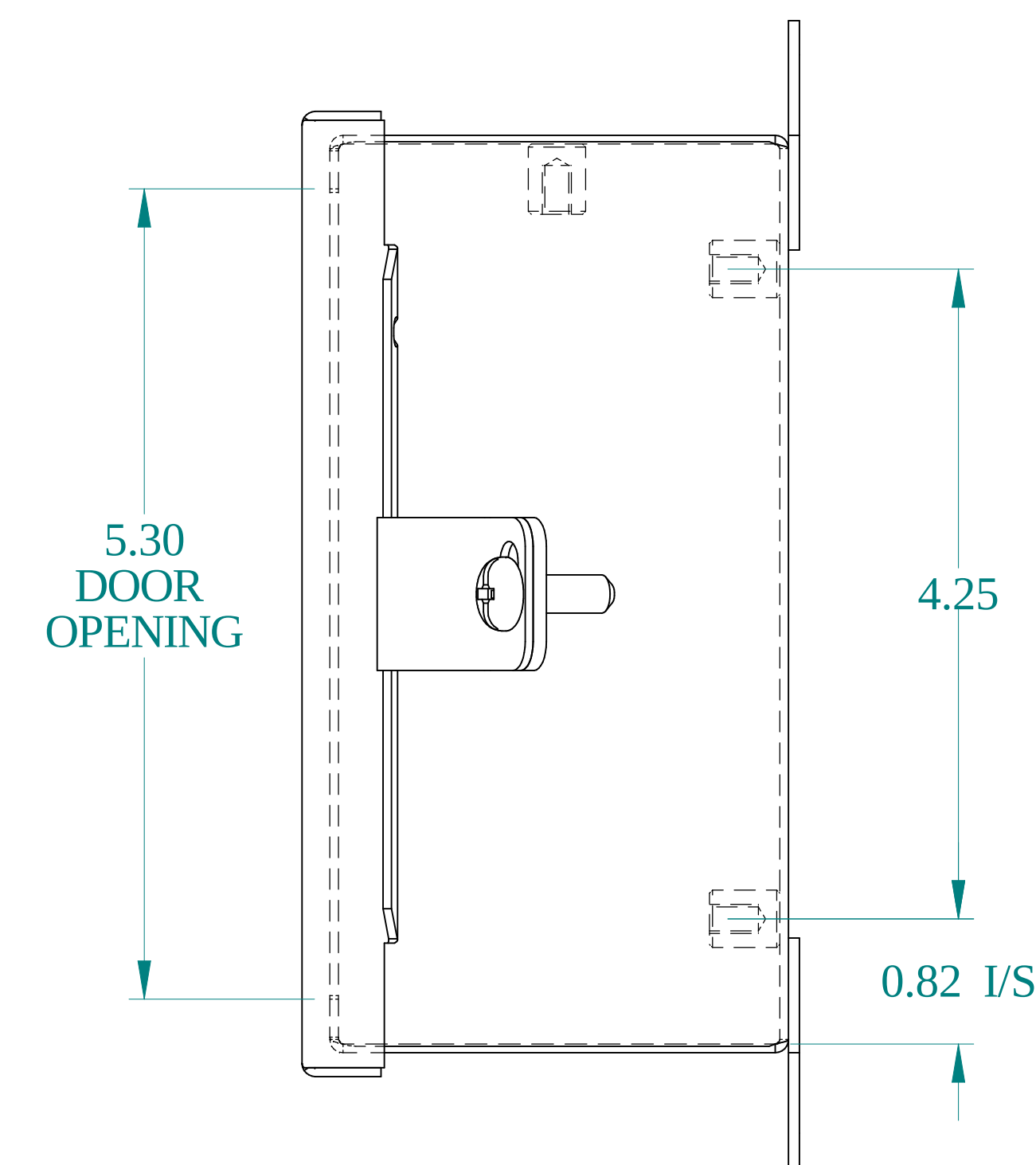
SIDE VIEW
