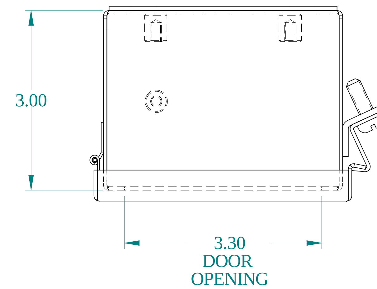
TOP VIEW
