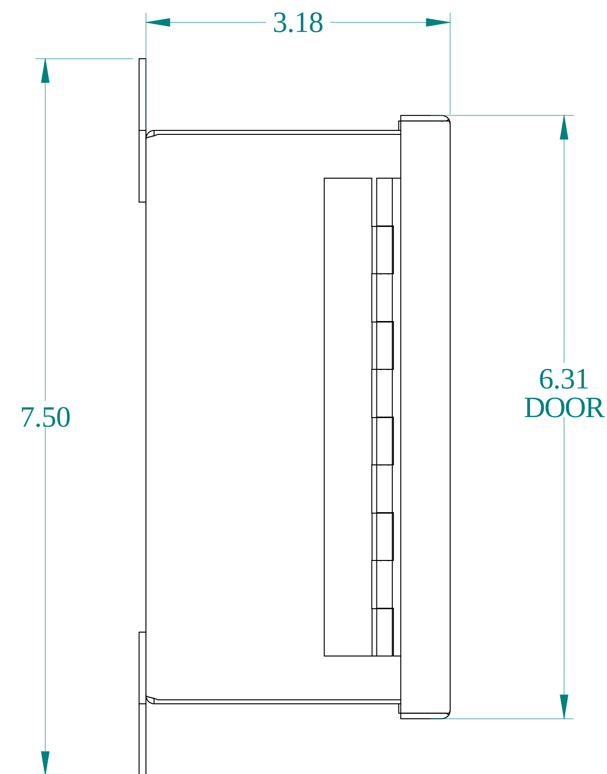
SIDE VIEW
