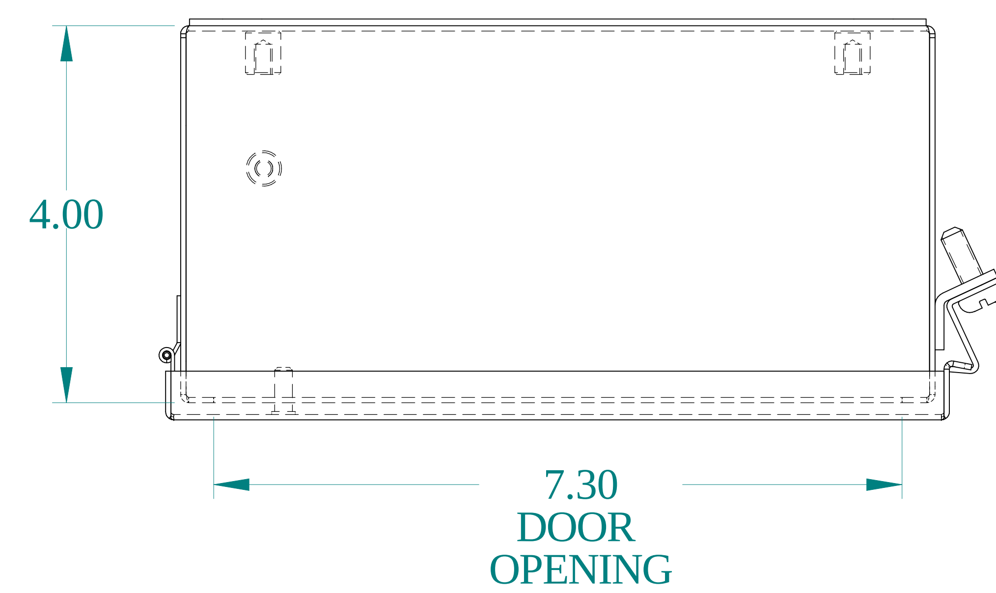
TOP VIEW
