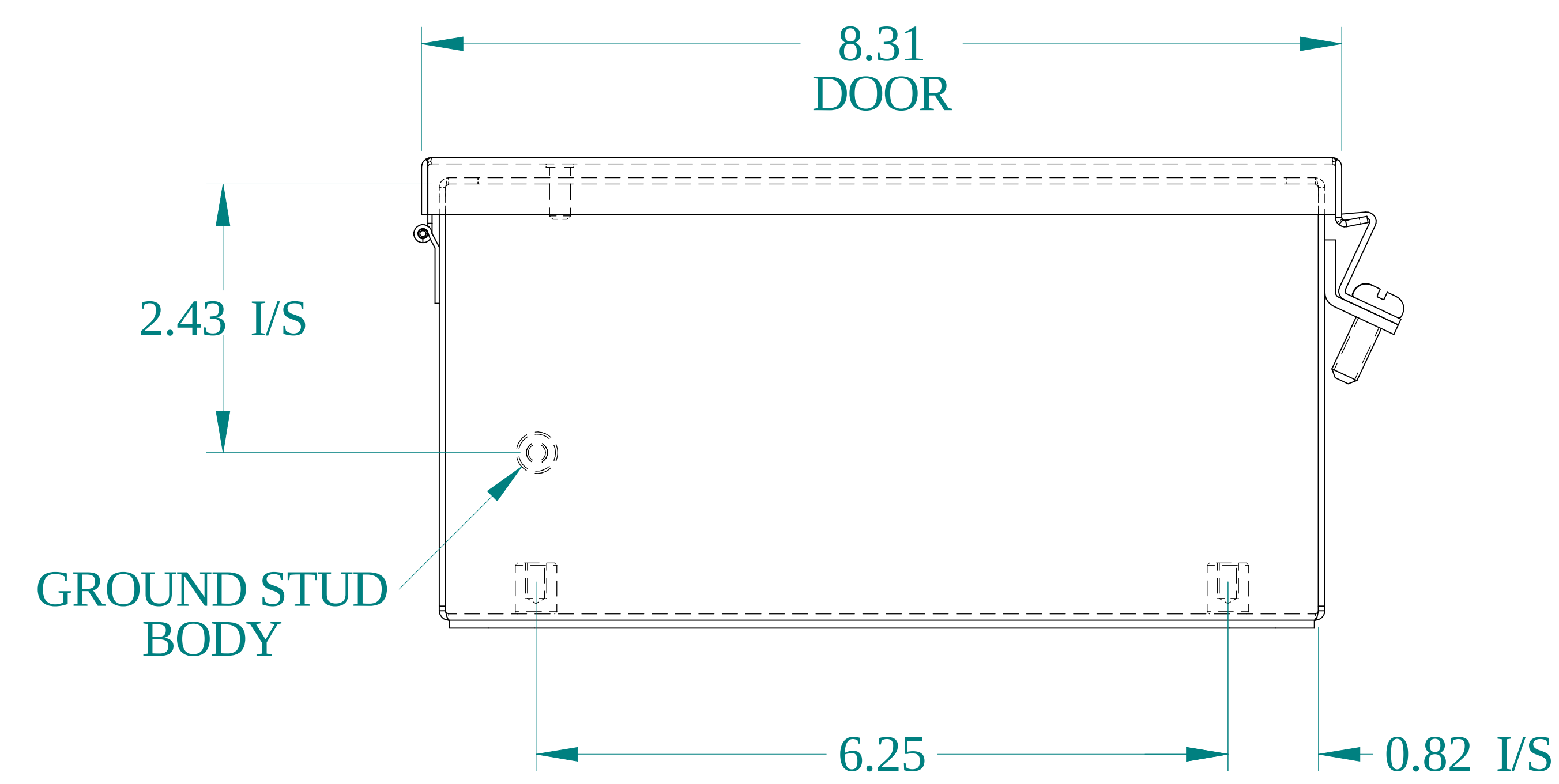
BOTTOM VIEW
