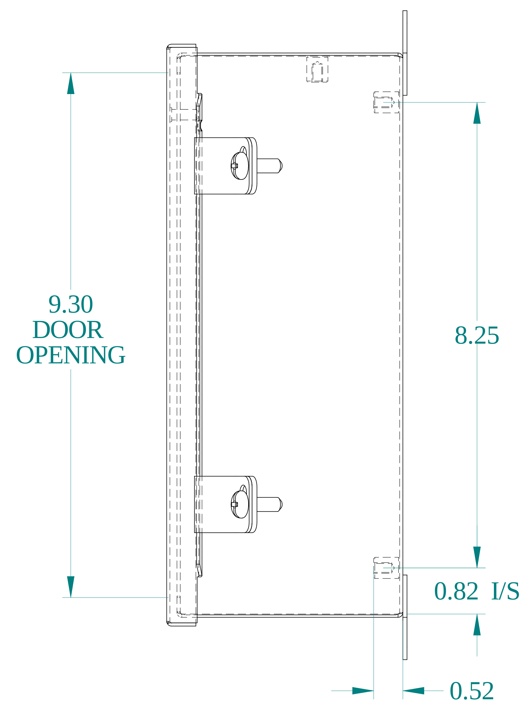
SIDE VIEW
