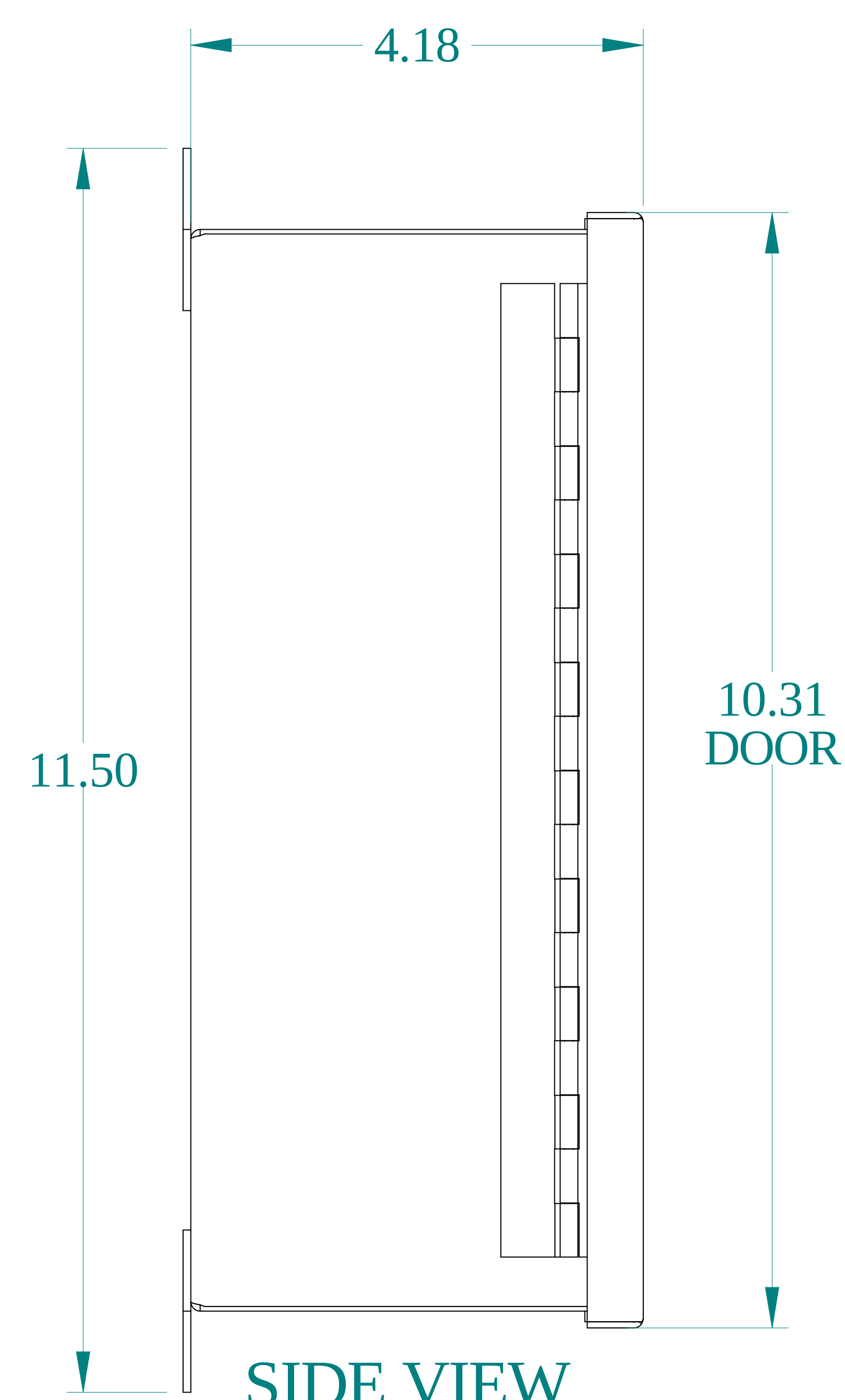
SIDE VIEW
