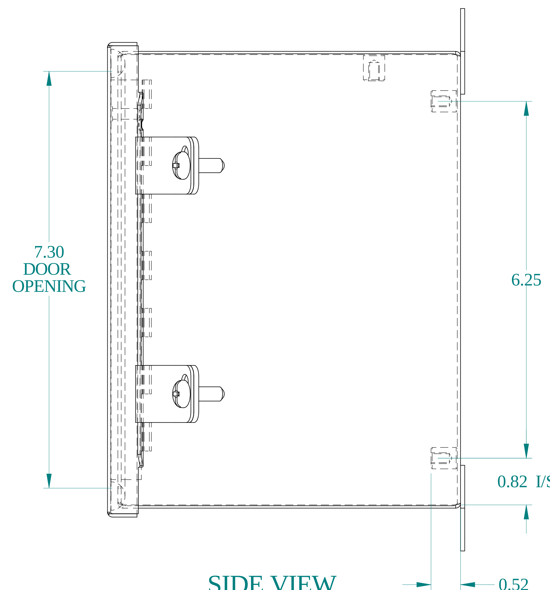
SIDE VIEW
