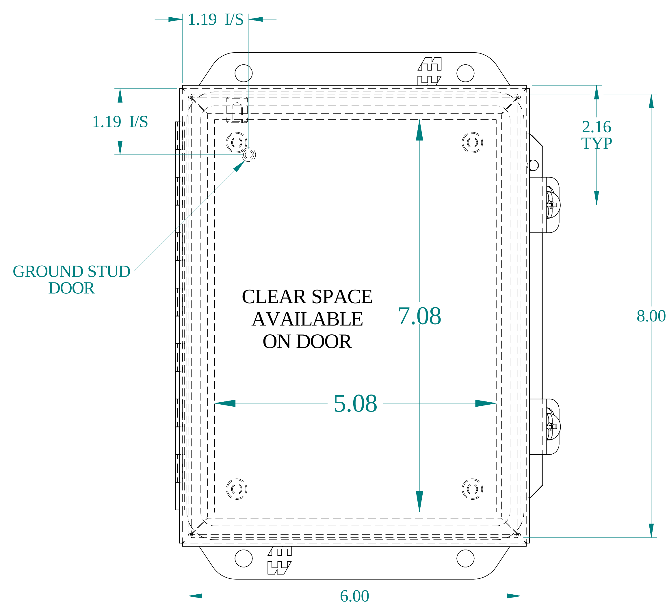
FRONT VIEW
