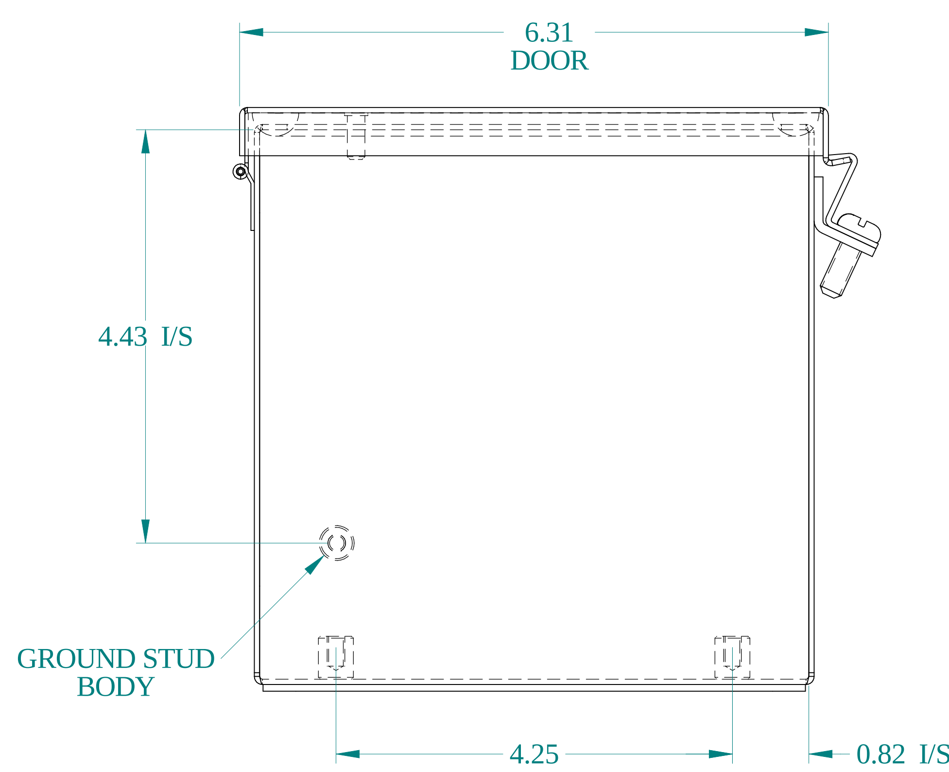
BOTTOM VIEW
