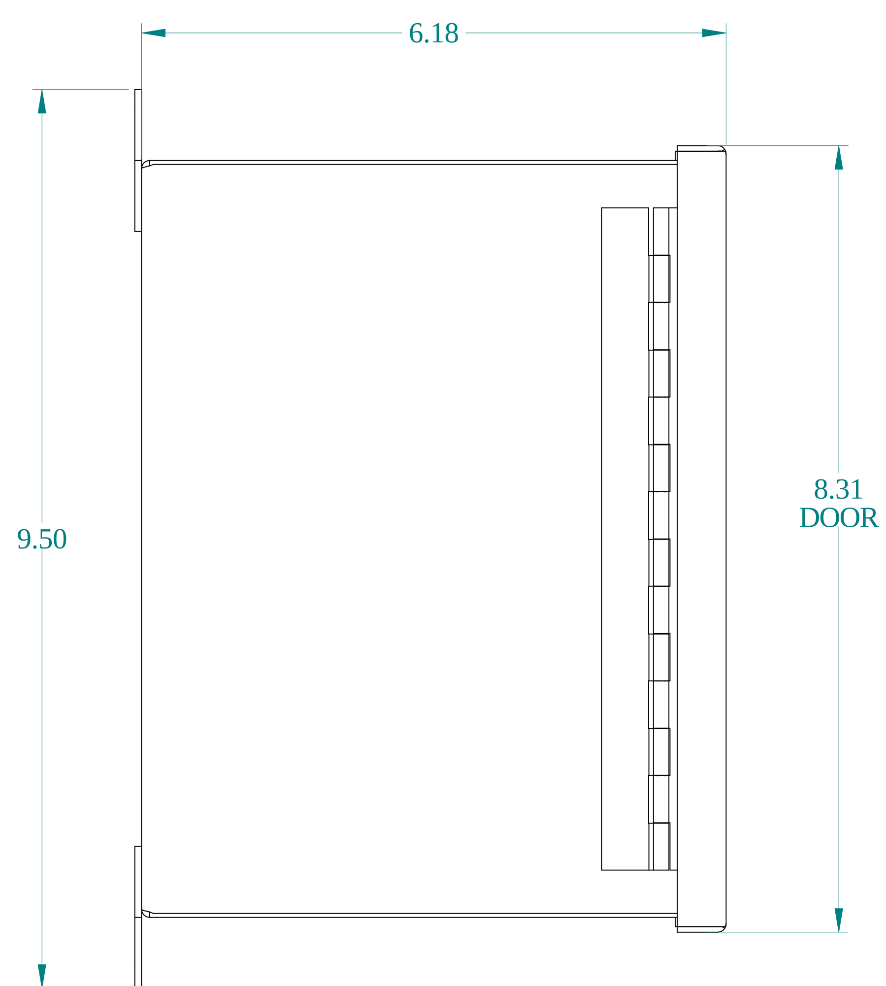
SIDE VIEW
