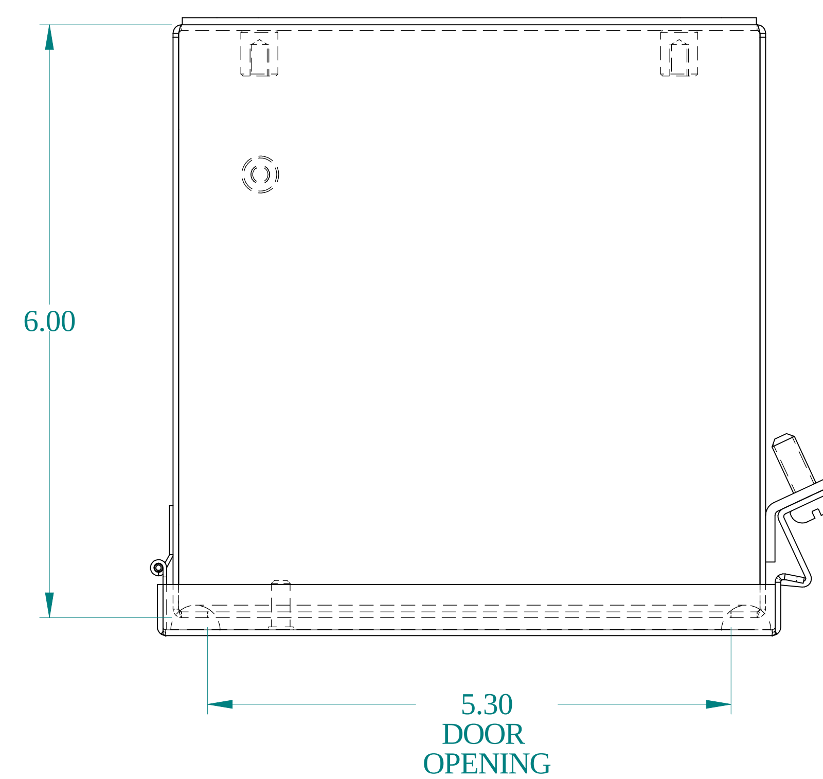
TOP VIEW
