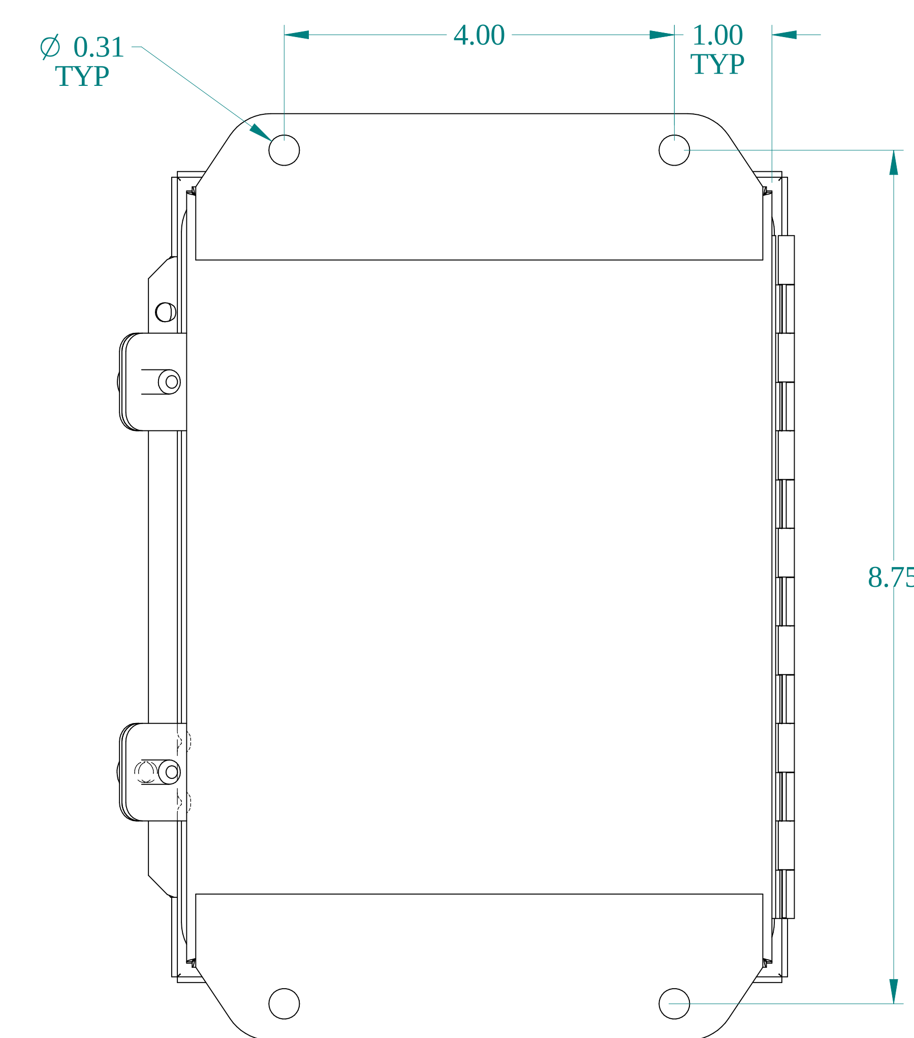
BACK VIEW
