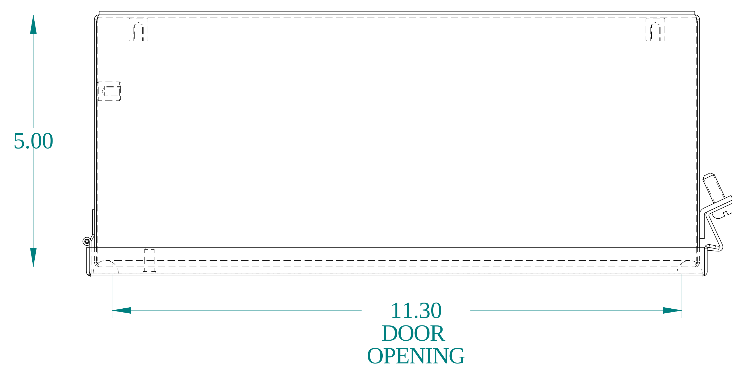
TOP VIEW
