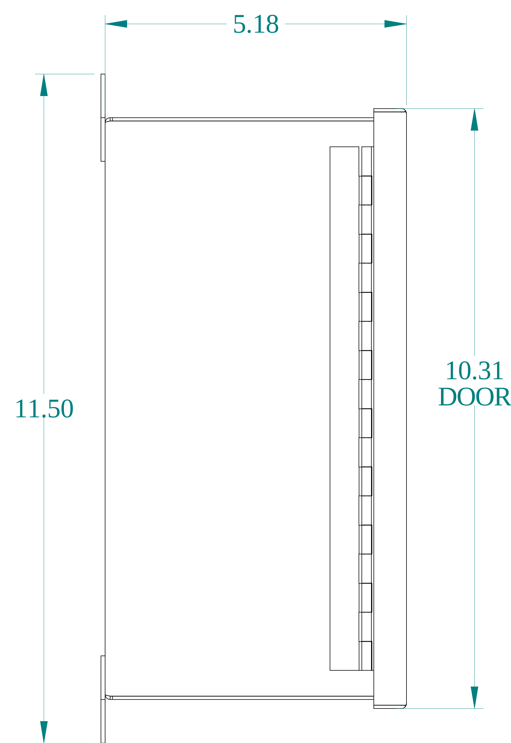
SIDE VIEW
