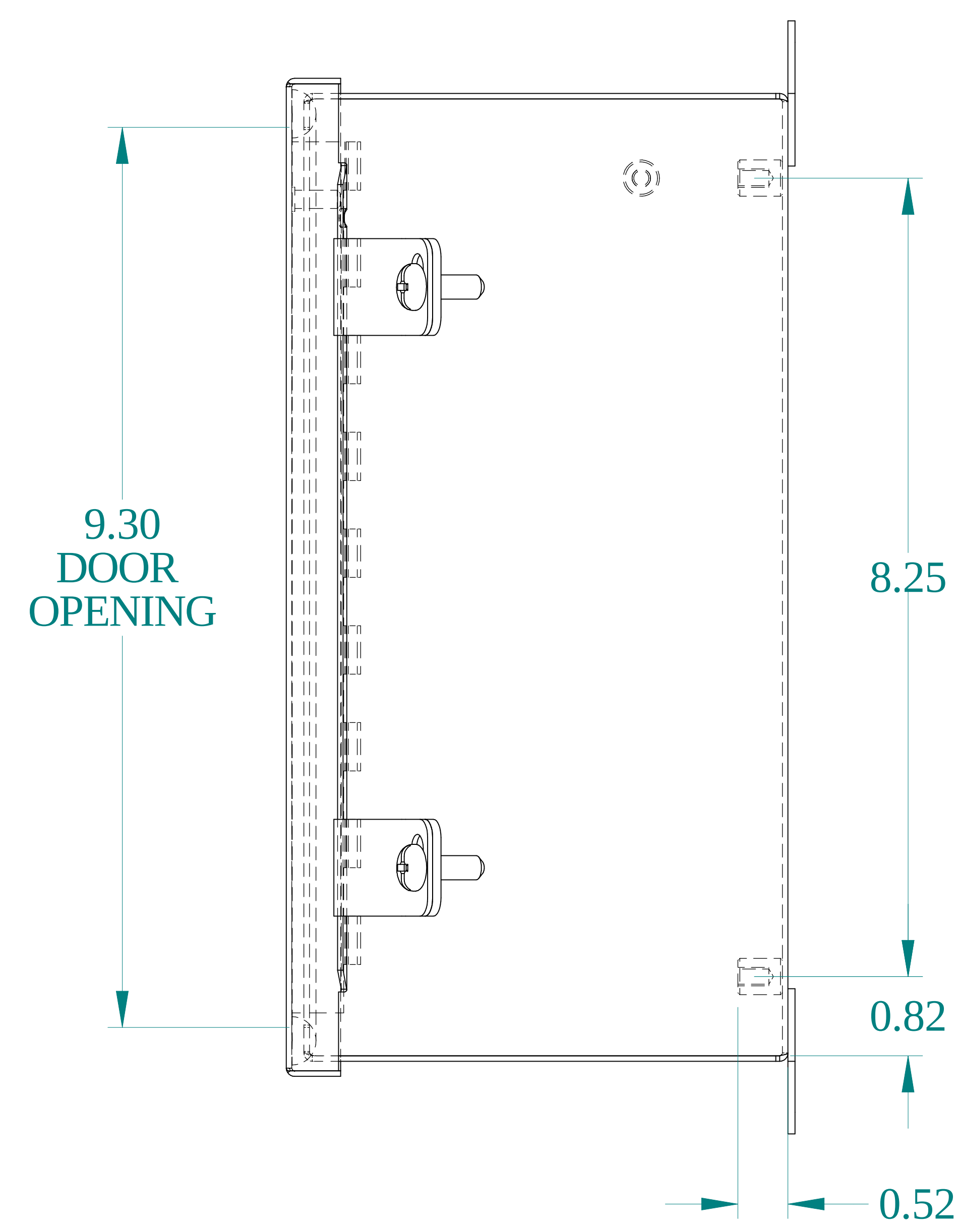
SIDE VIEW
