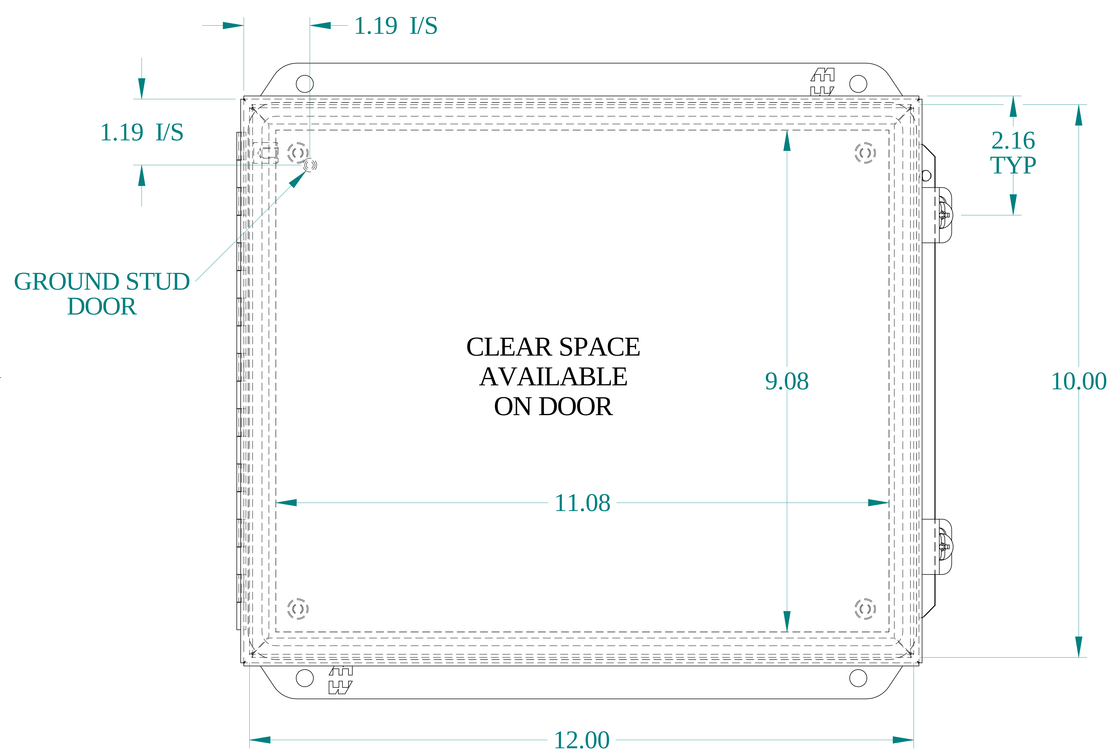
FRONT VIEW
