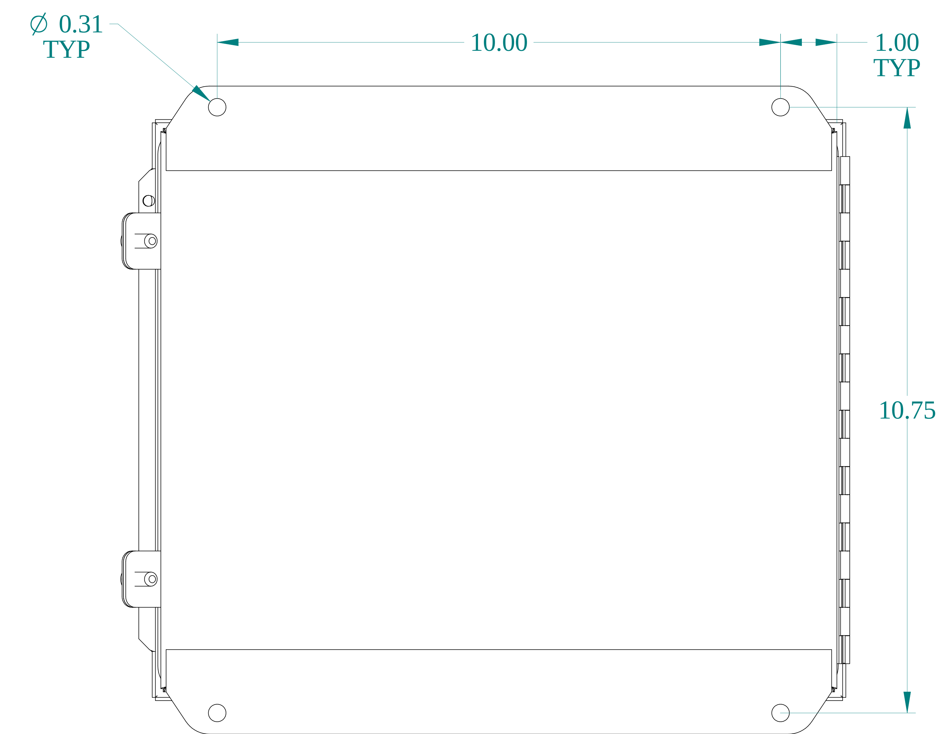
BACK VIEW
