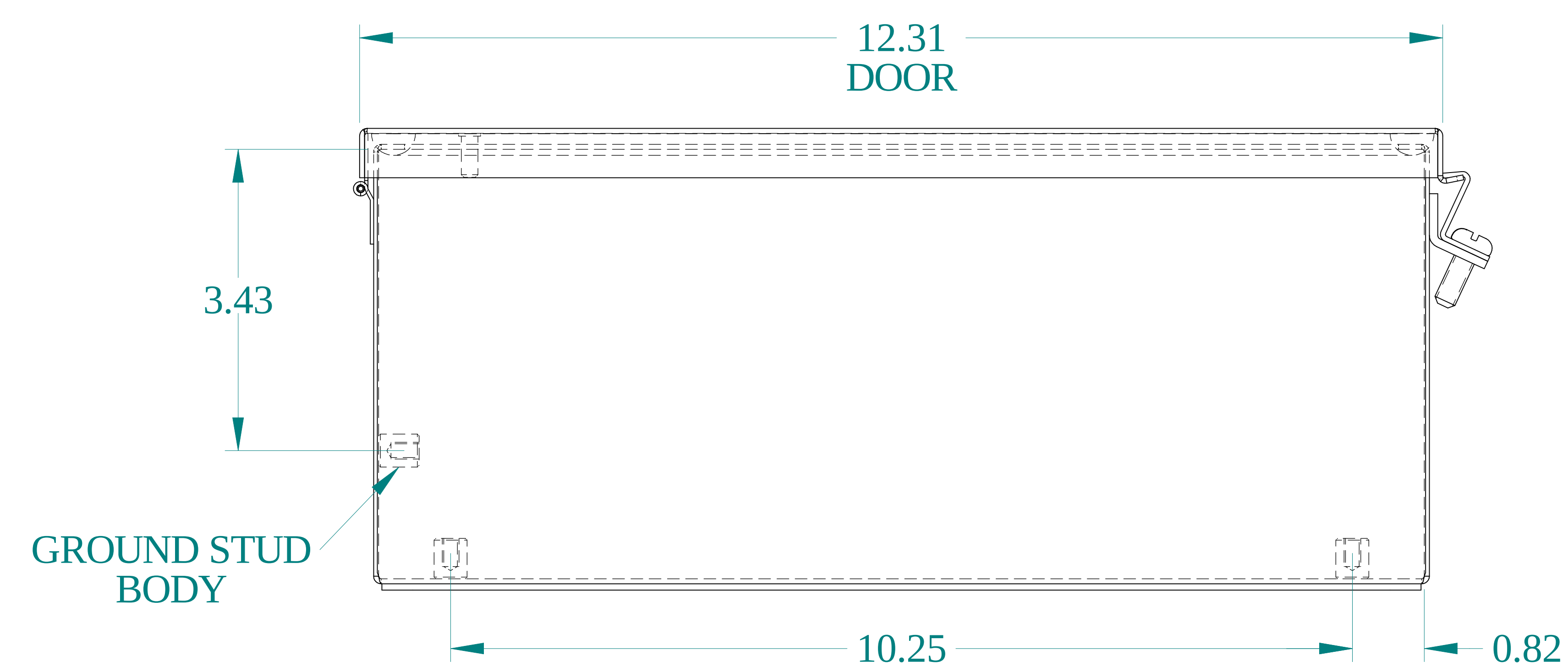
BOTTOM VIEW
