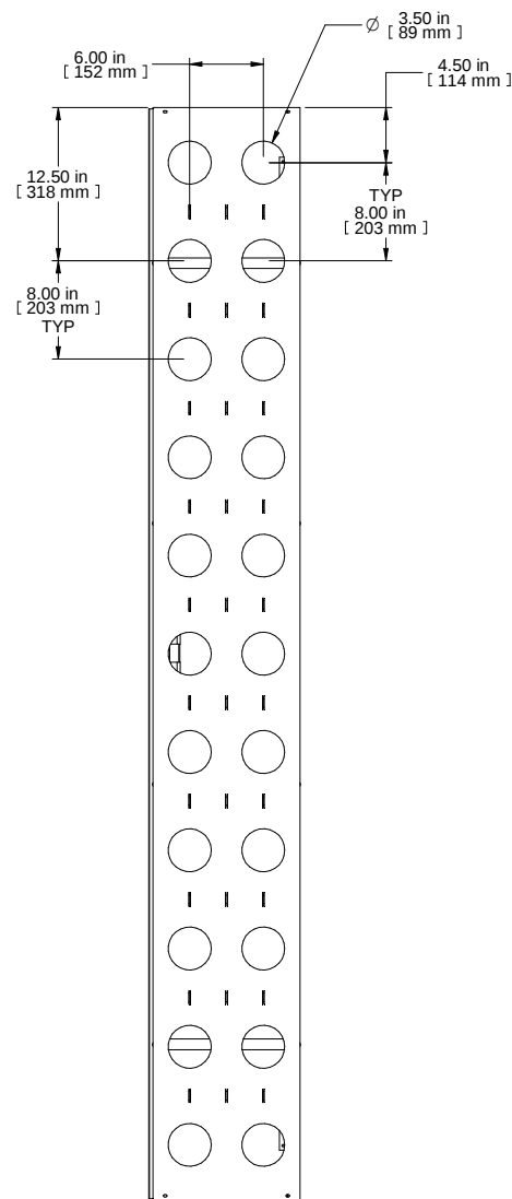
REAR VIEW
