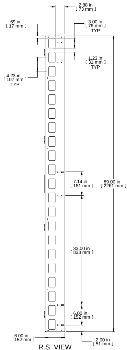
R.S. VIEW
