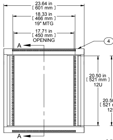
FRONT VIEW DOOR REMOVED
