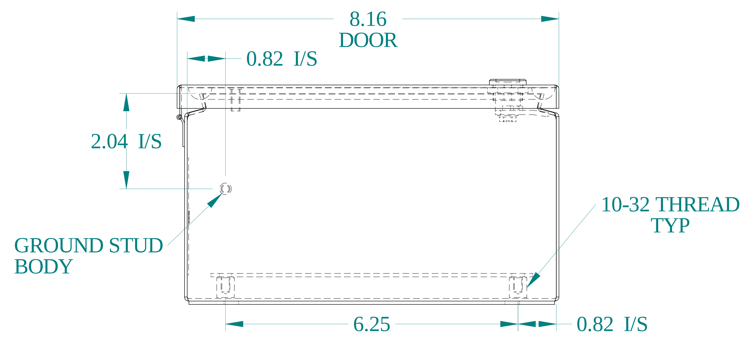
BOTTOM VIEW
