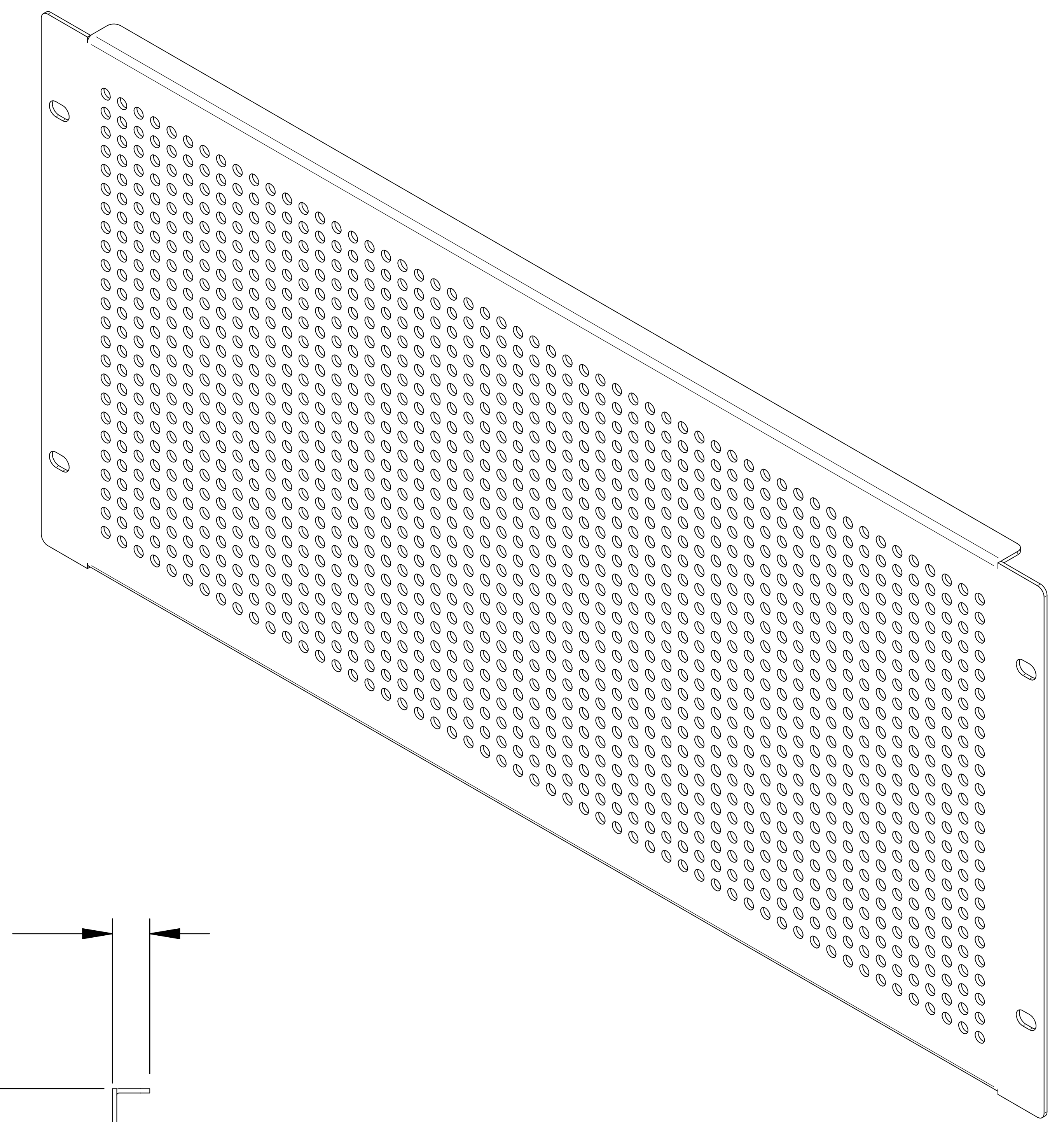
ISOMETRIC
