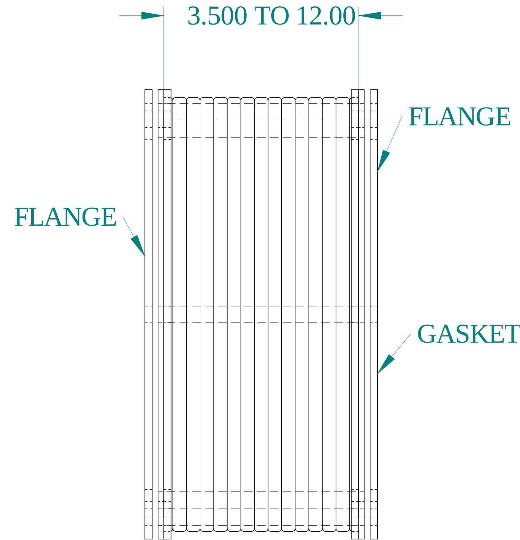
FRONT VIEW
