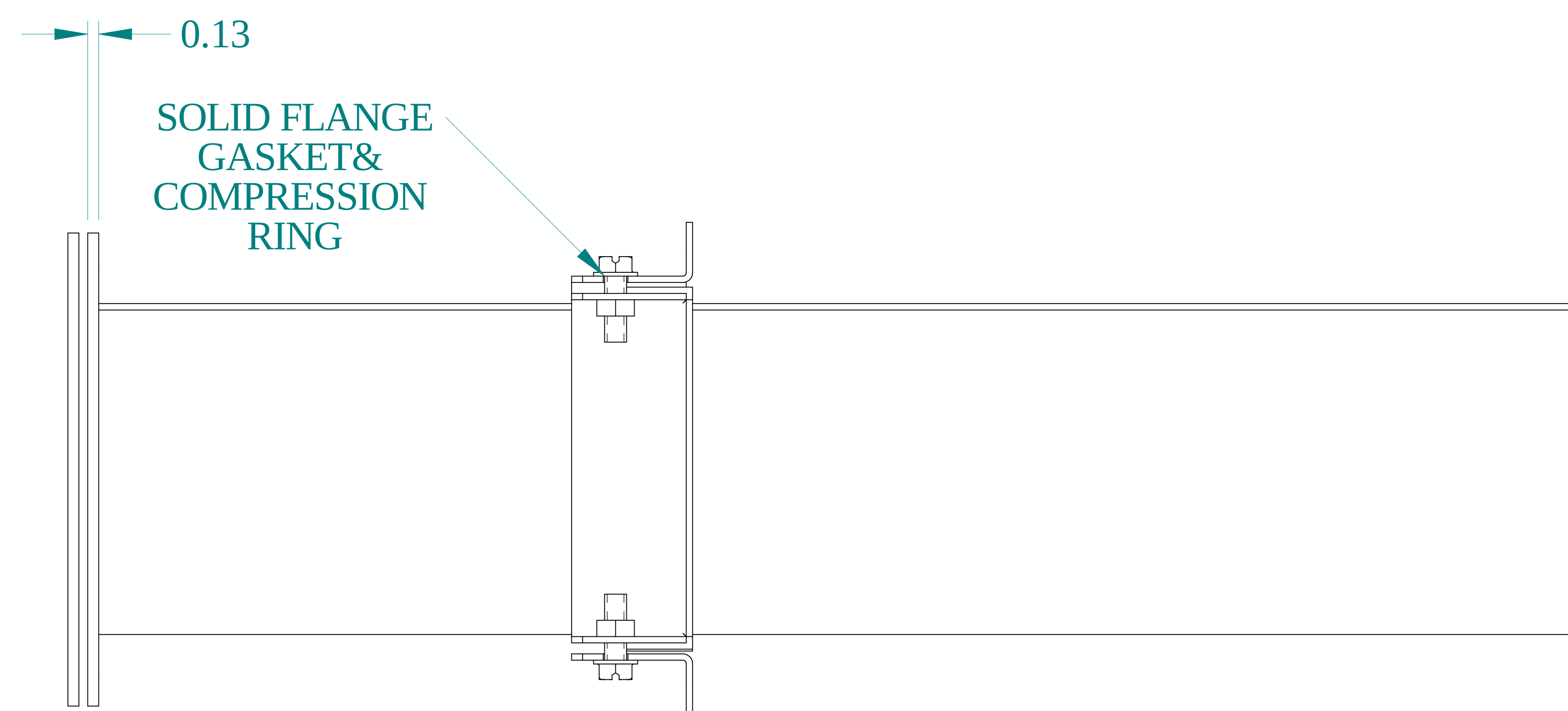
TOP VIEW
