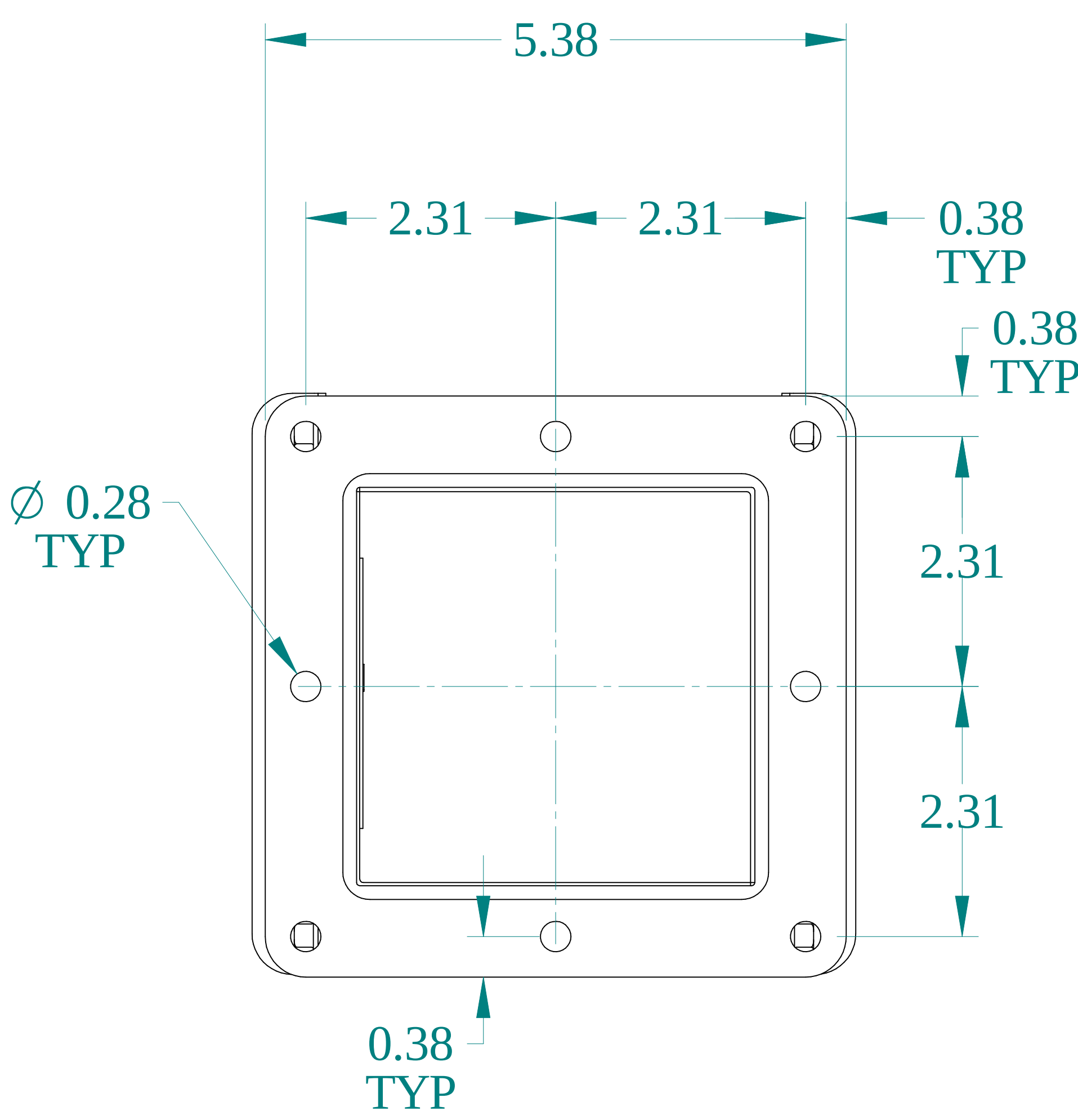
SIDE VIEW
