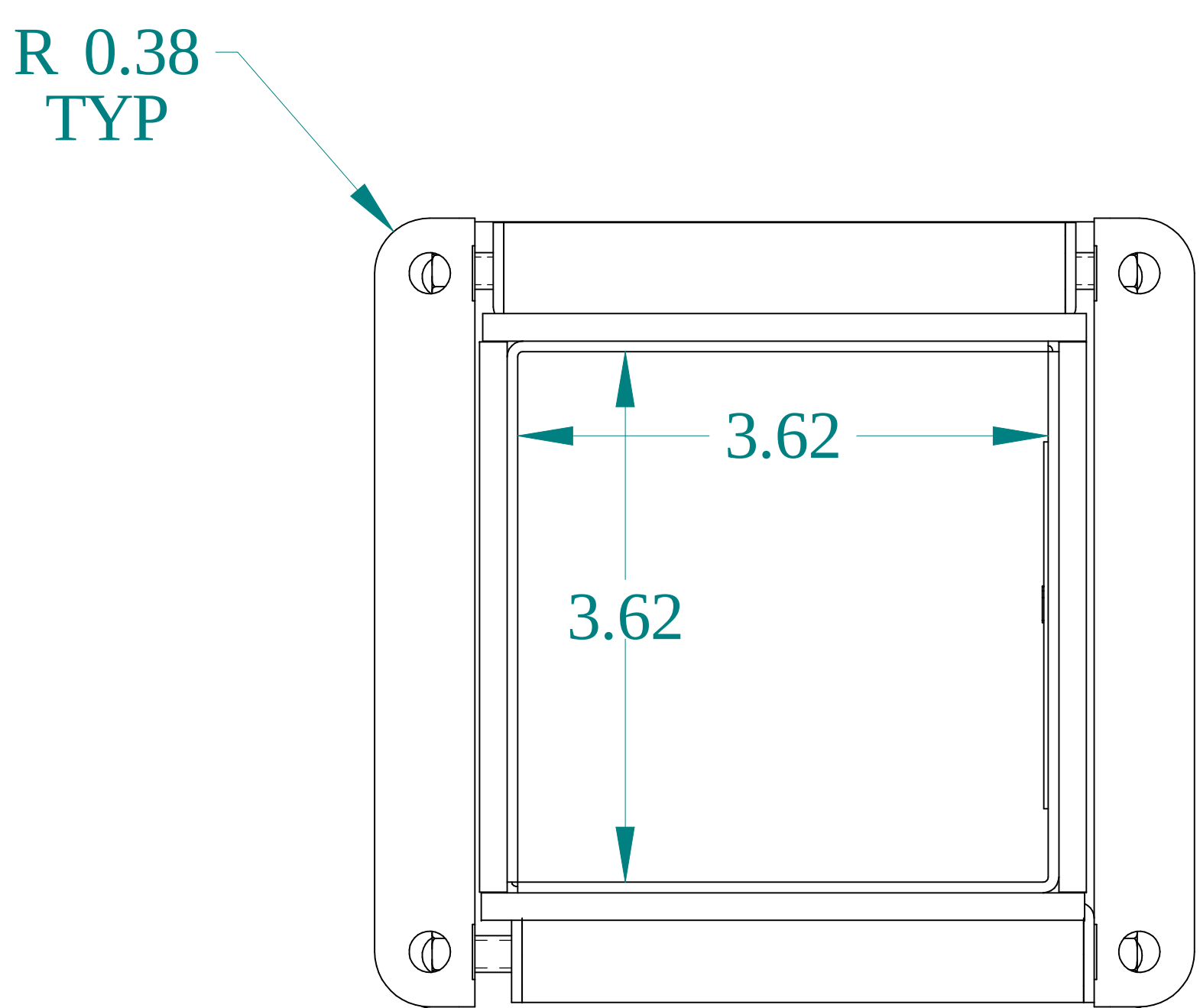
SIDE VIEW
