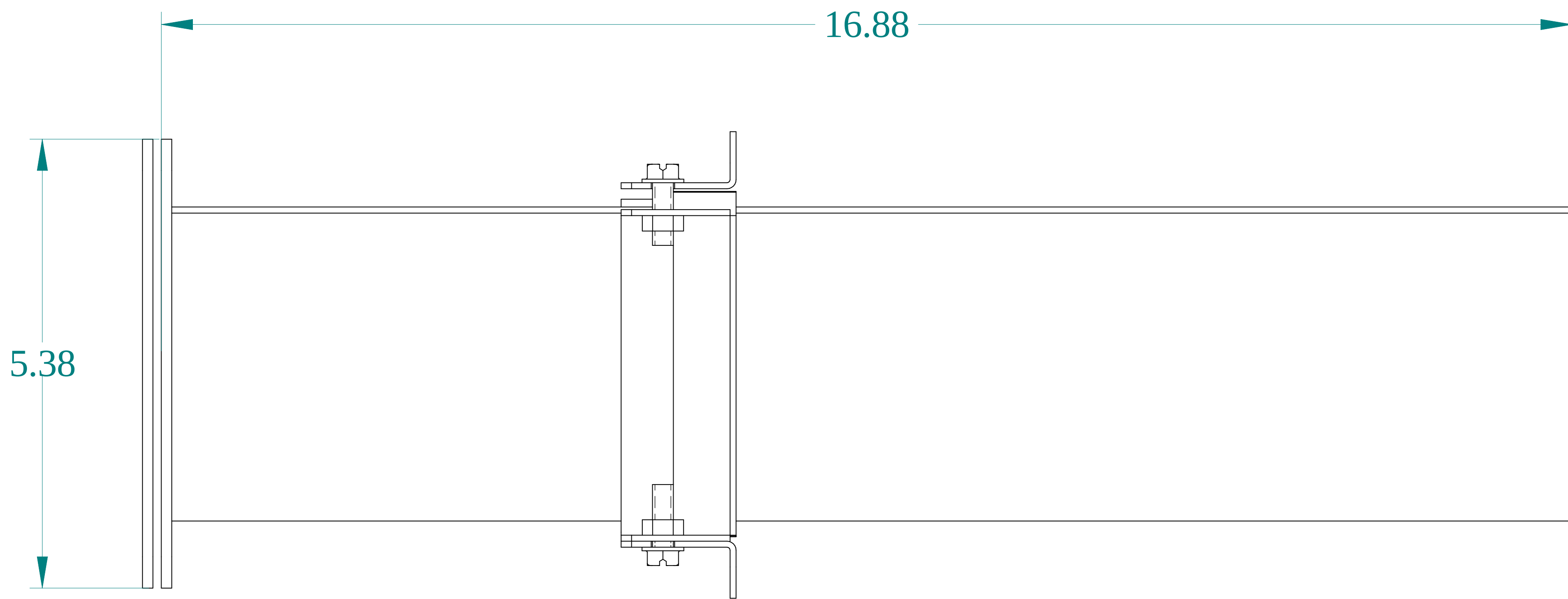
BOTTOM VIEW
