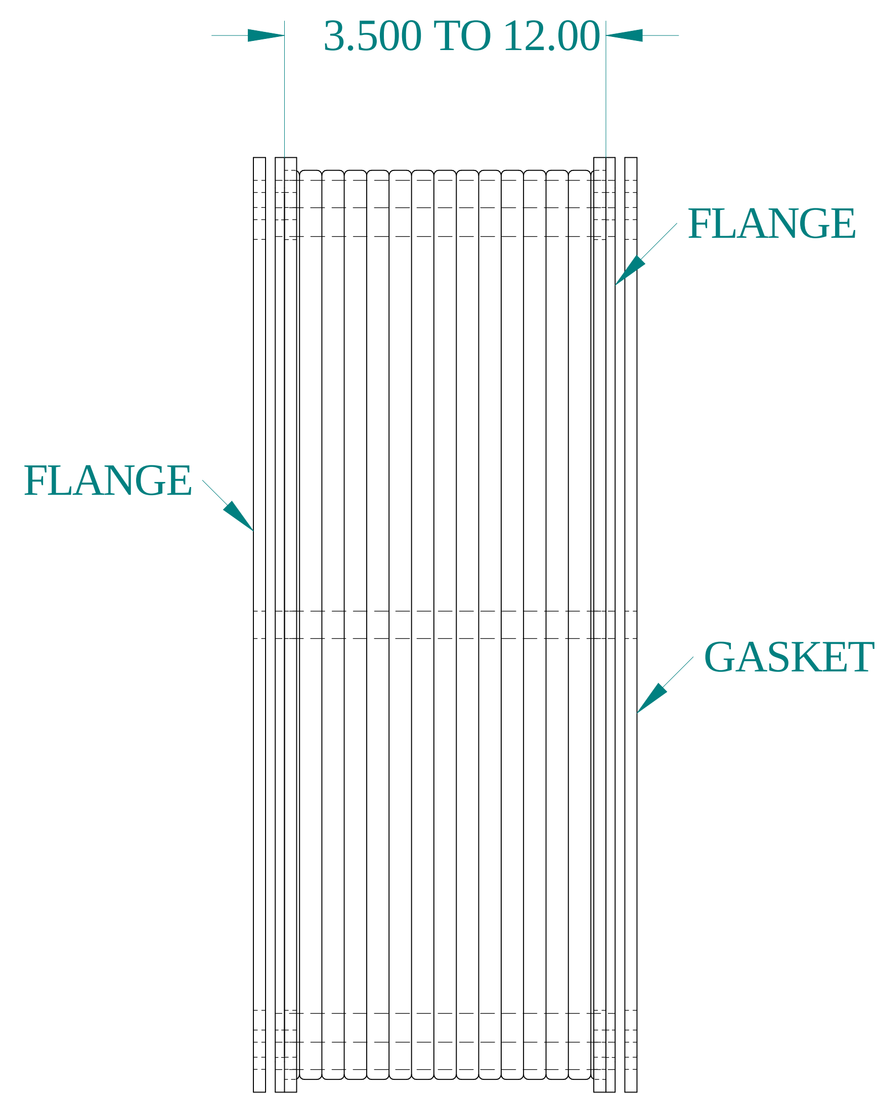
FRONT VIEW
