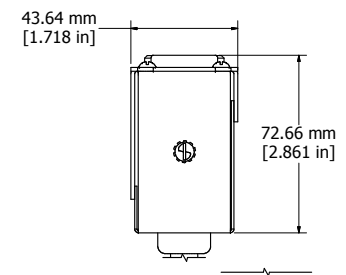
ASSEMBLY - VIEW FROM SIDE
