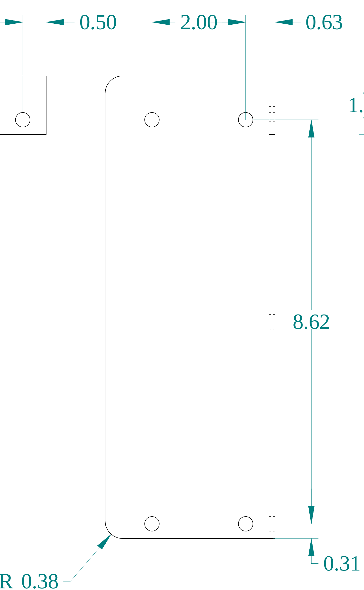
SIDE VIEW
