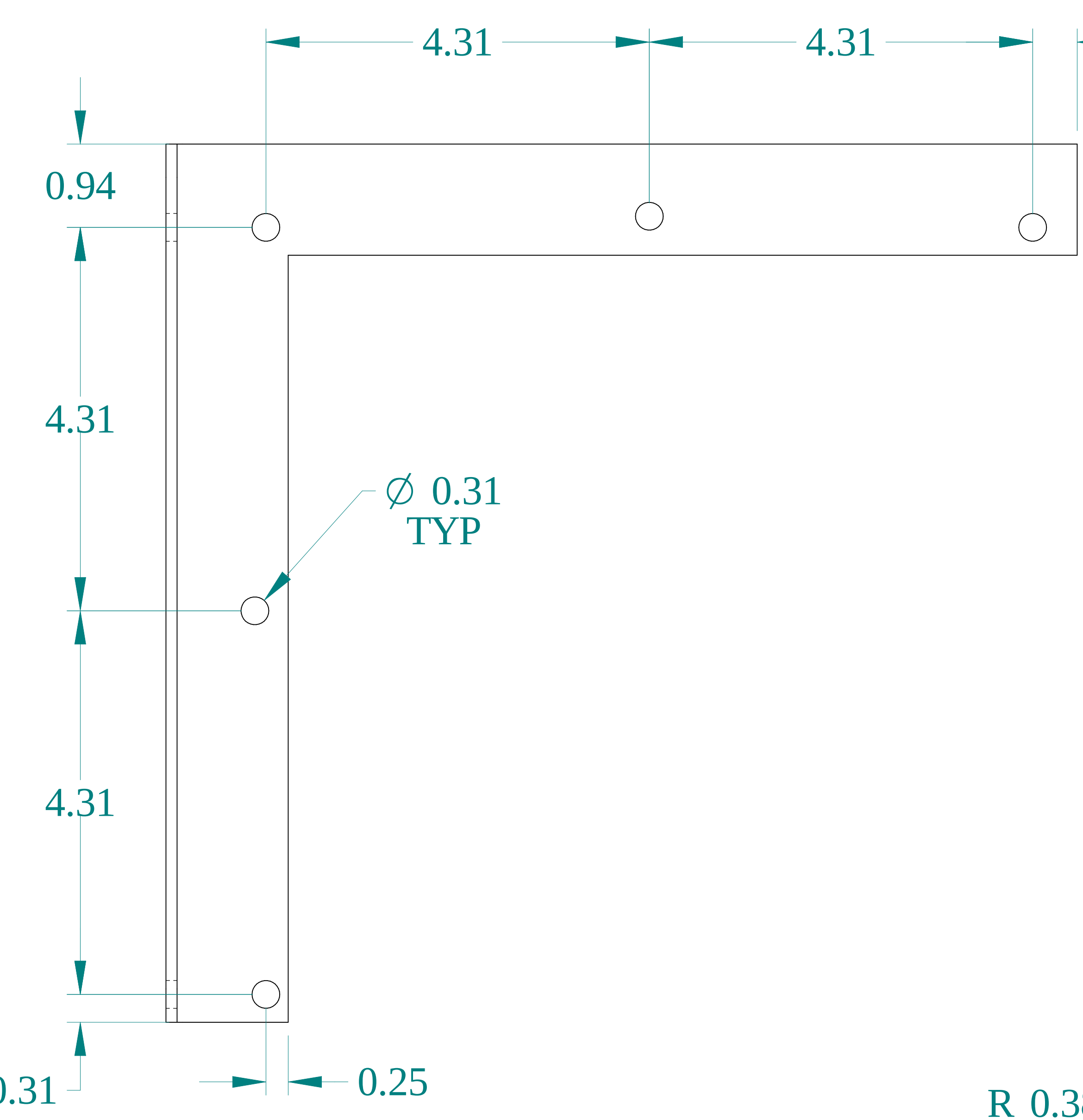
FRONT VIEW
