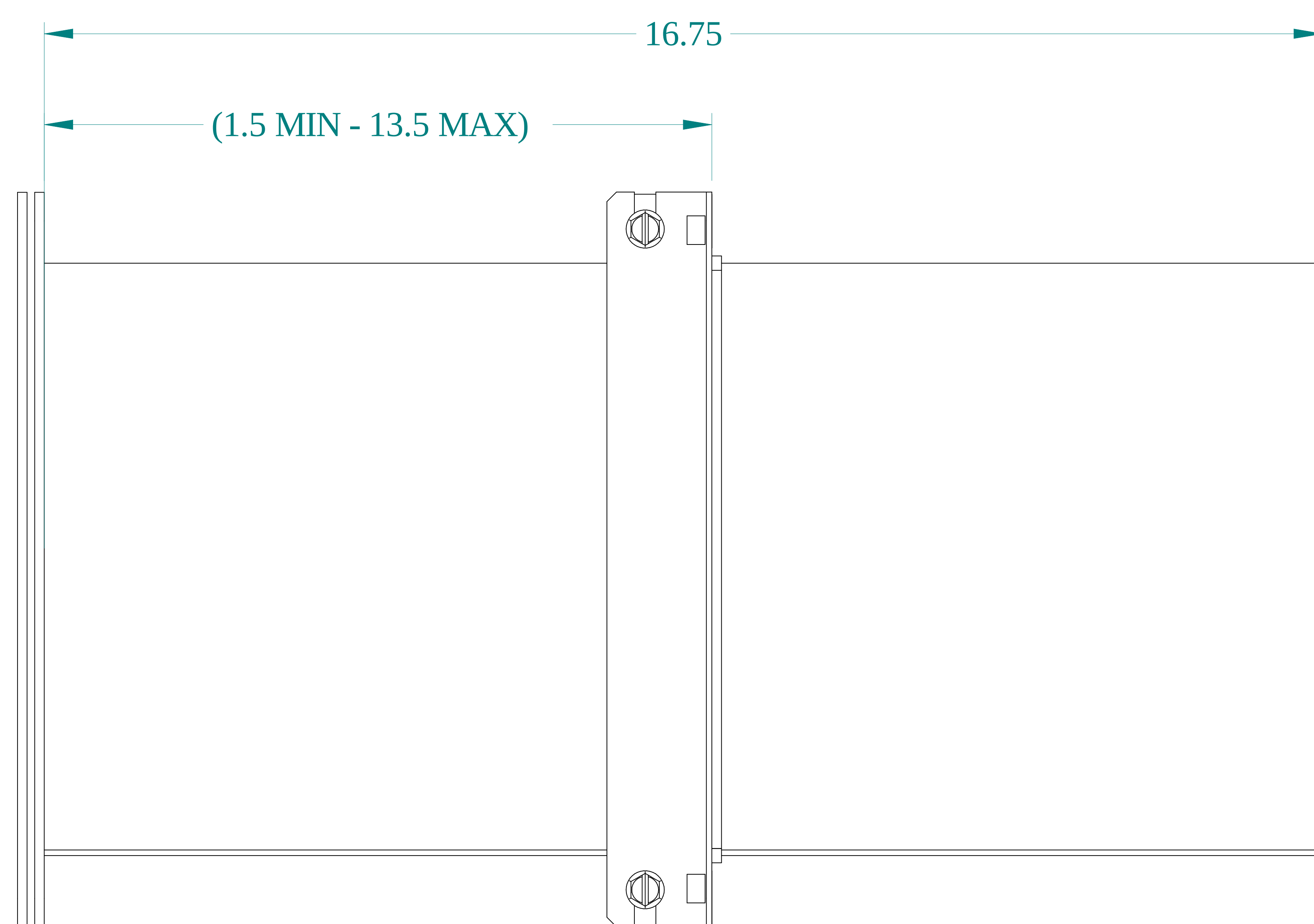
FRONT VIEW
