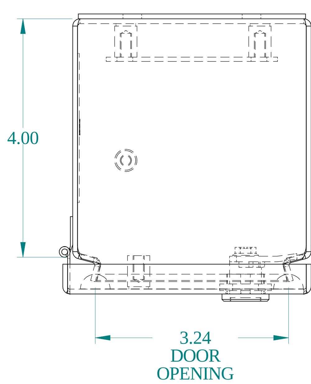
TOP VIEW
