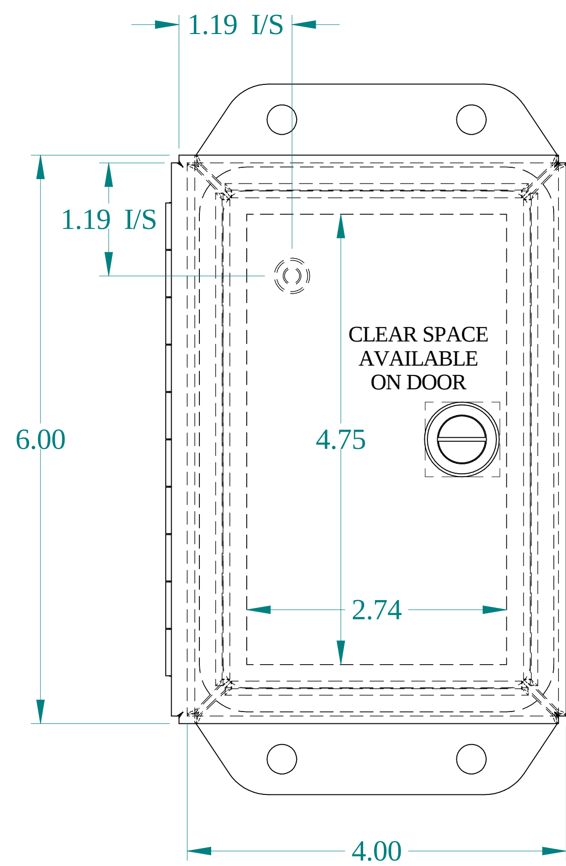
FRONT VIEW
