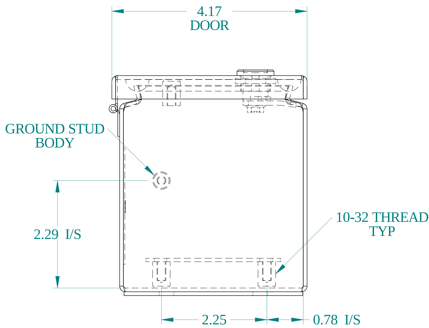
BOTTOM VIEW
