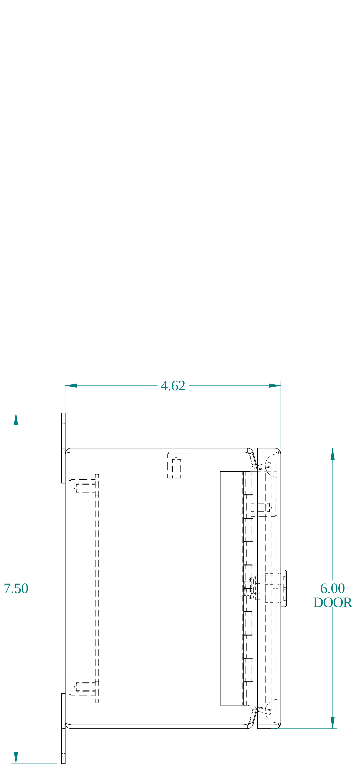
SIDE VIEW
