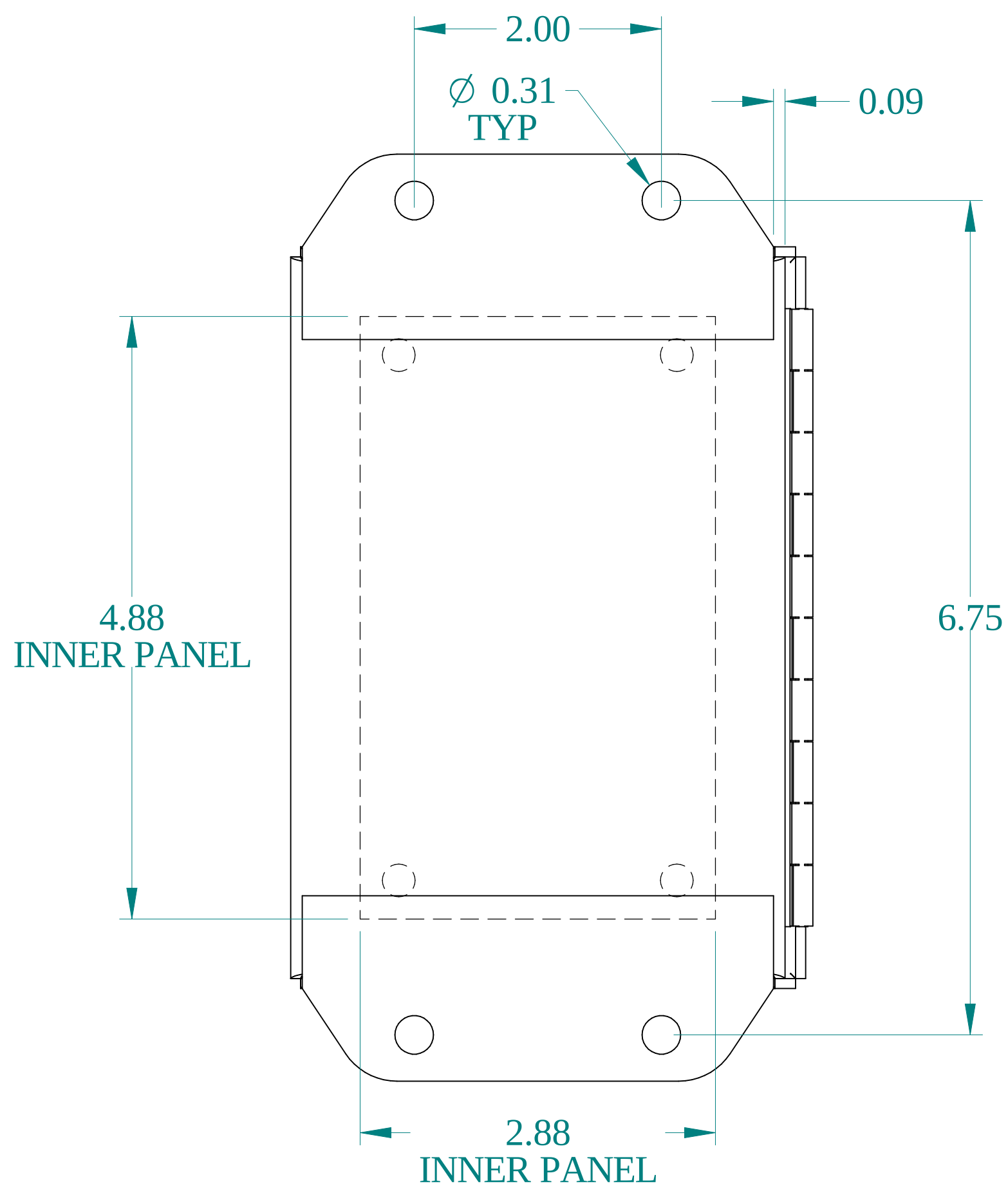
BACK VIEW
