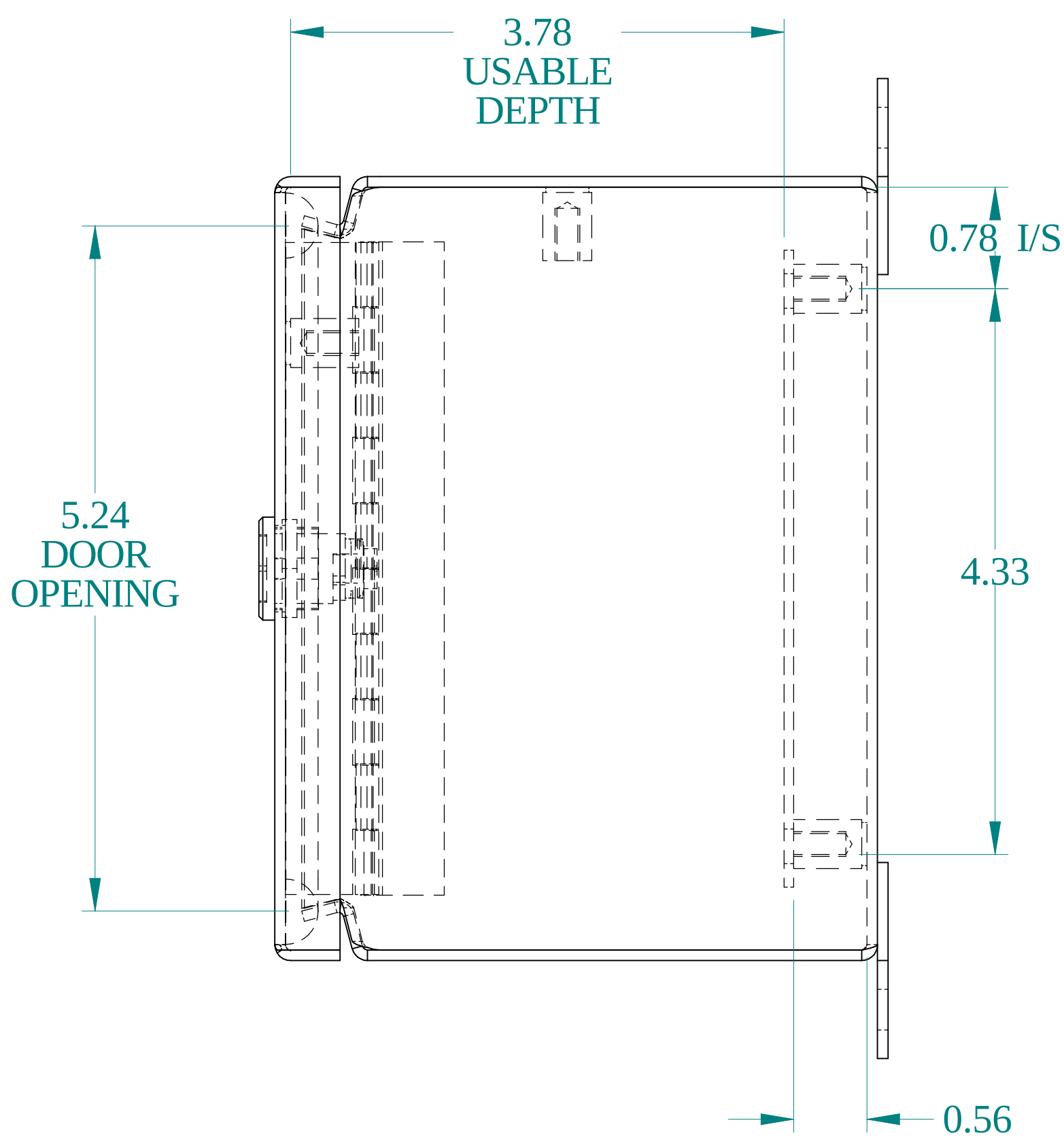
SIDE VIEW
