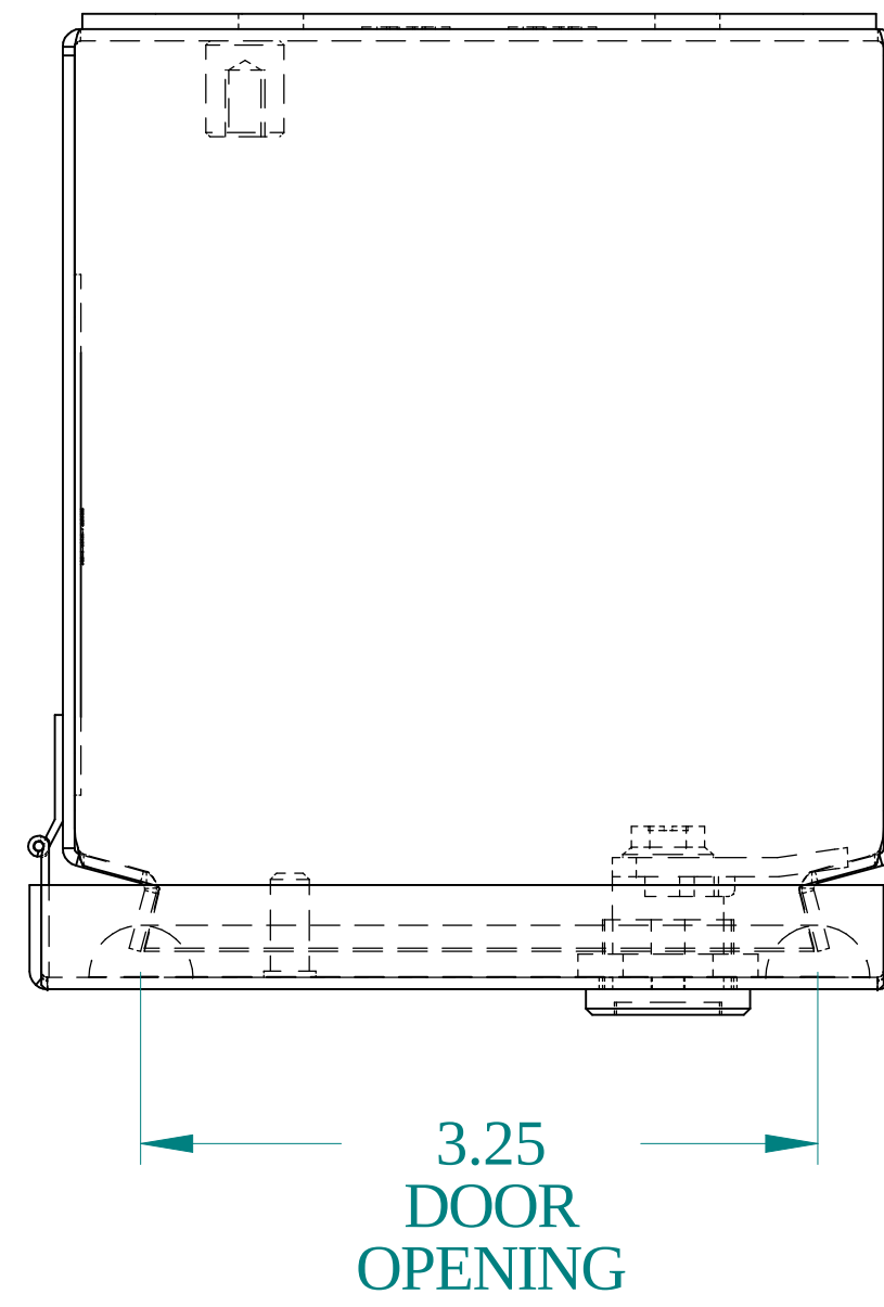
TOP VIEW
