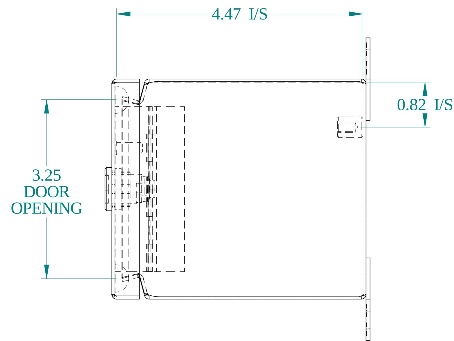
SIDE VIEW
