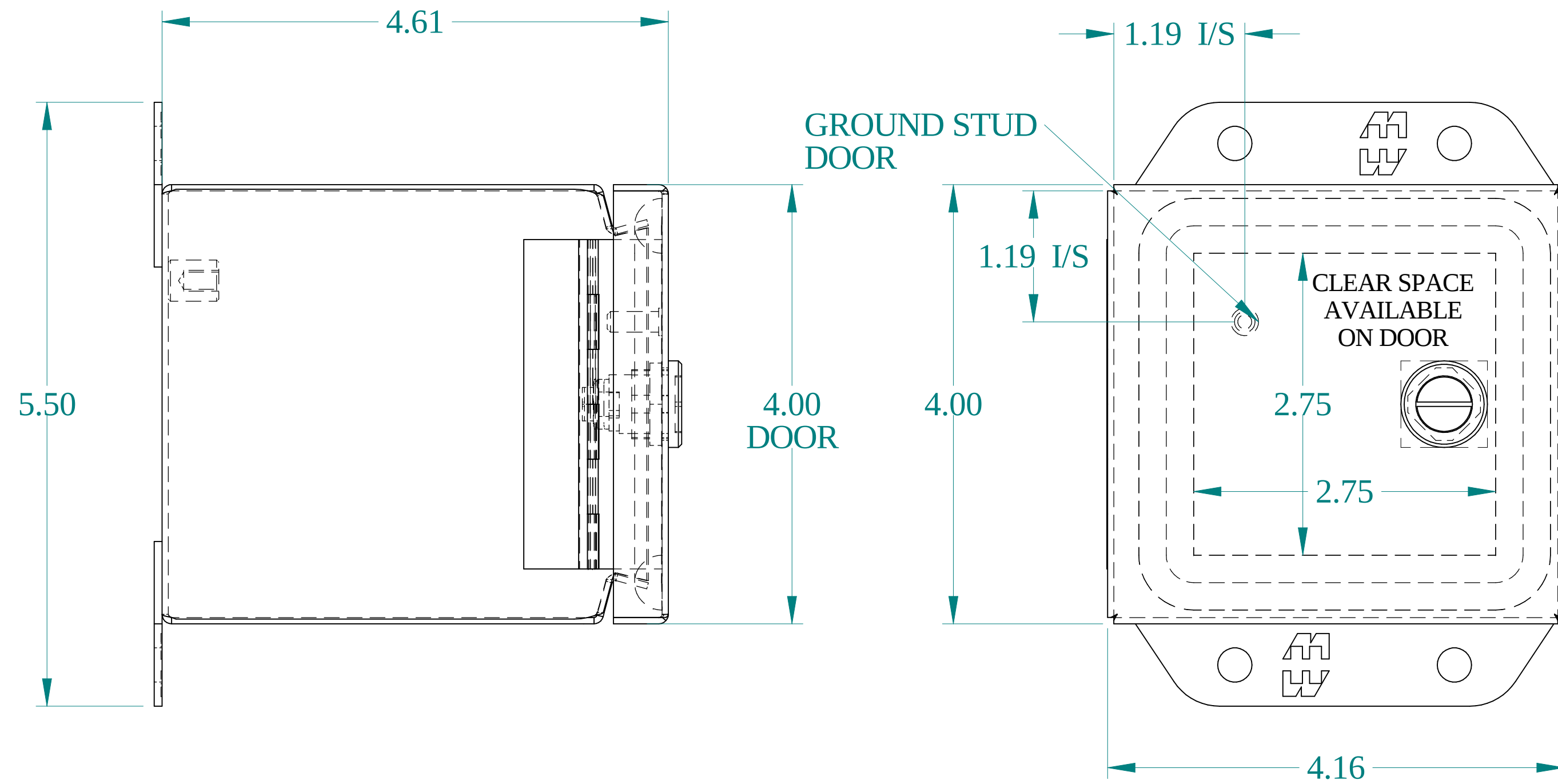
SIDE VIEW
