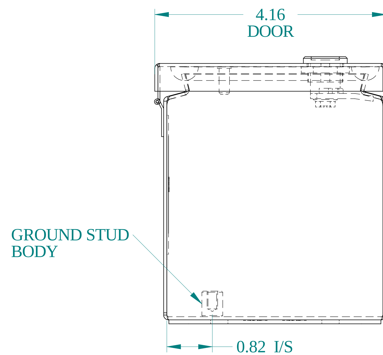
BOTTOM VIEW
