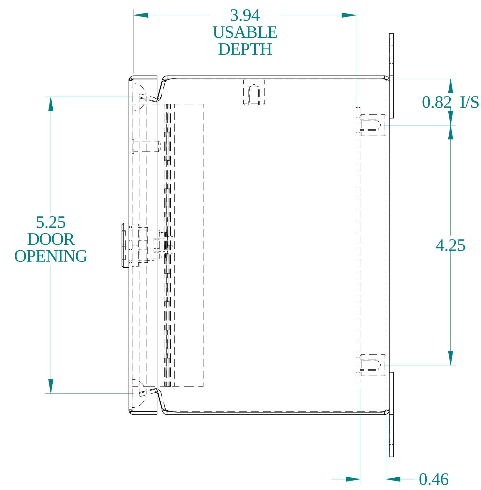
SIDE VIEW
