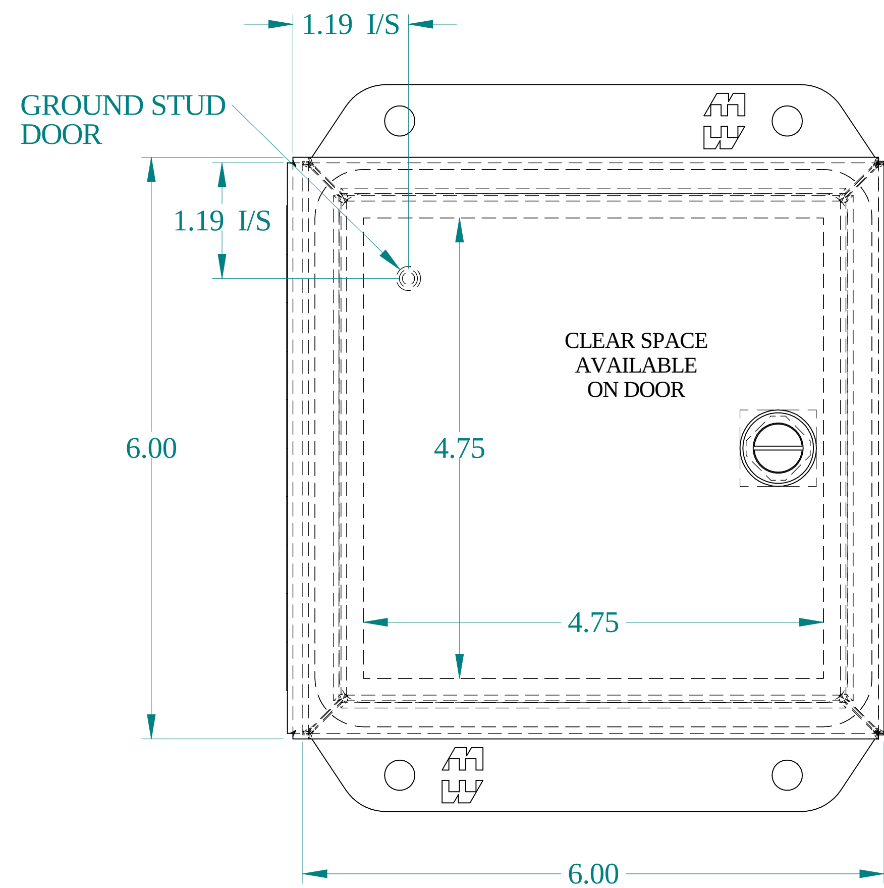
FRONT VIEW
