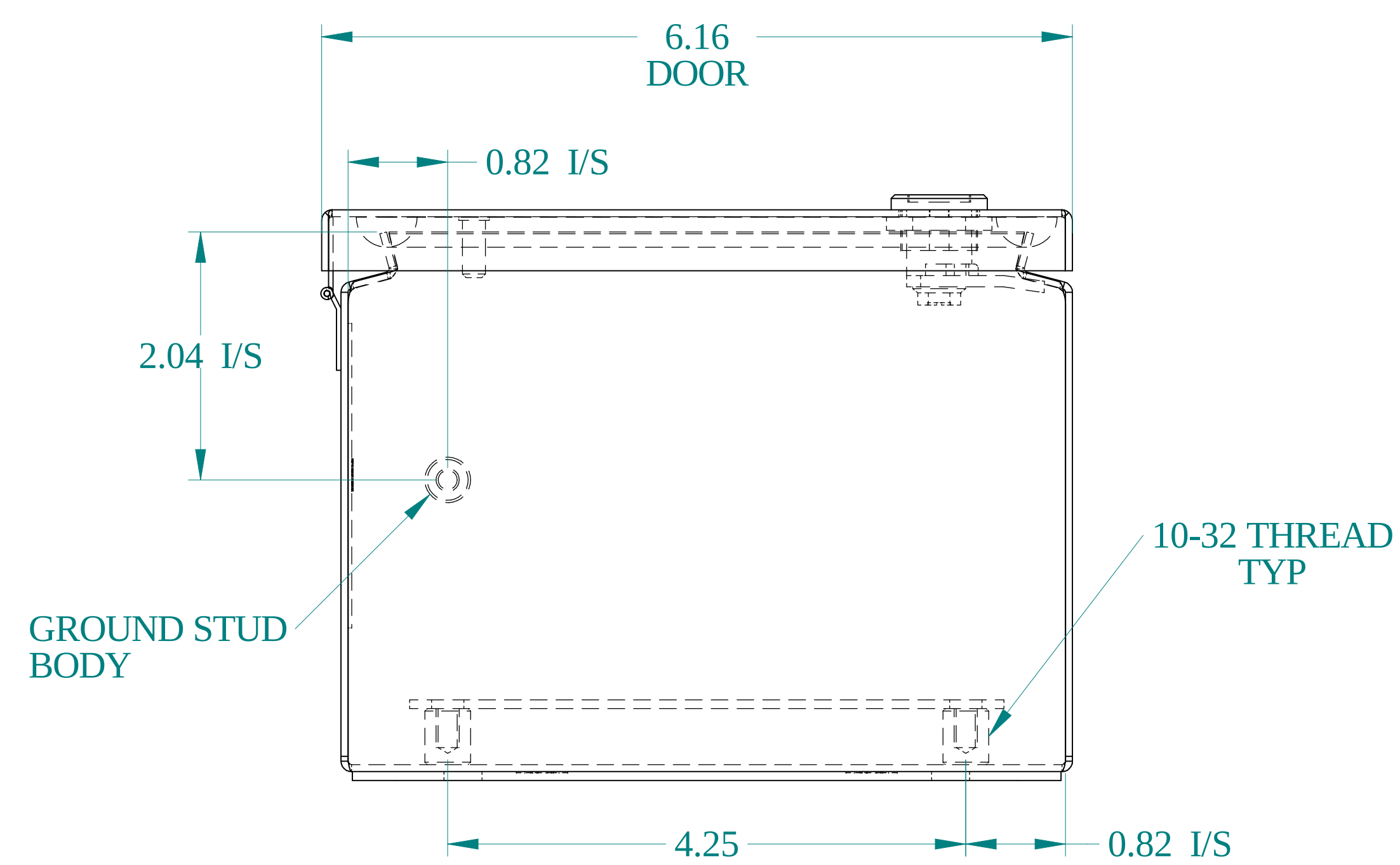
BOTTOM VIEW
