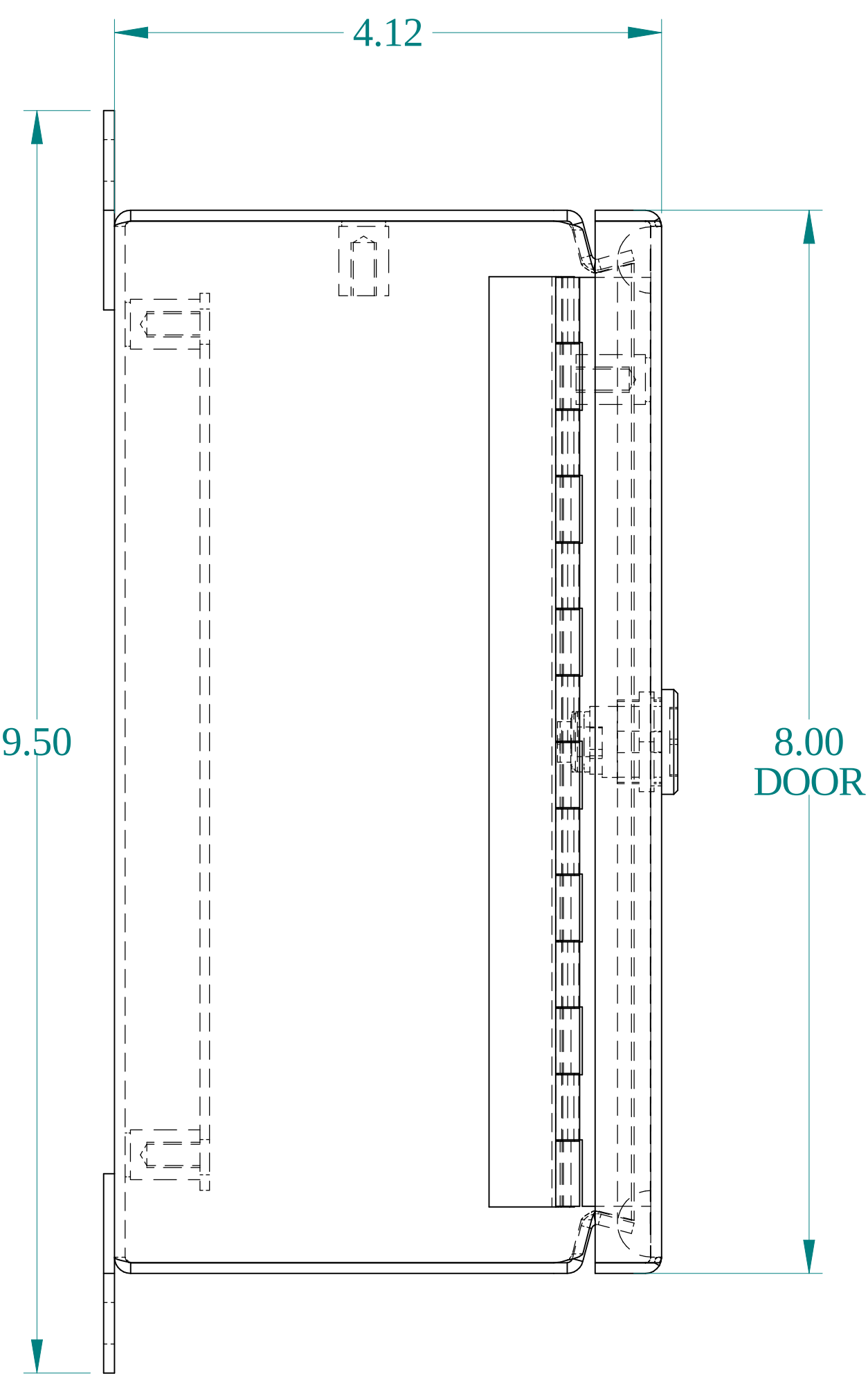
SIDE VIEW
