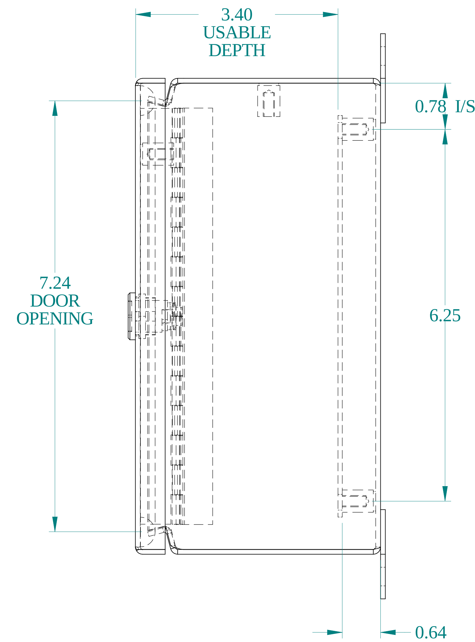
SIDE VIEW
