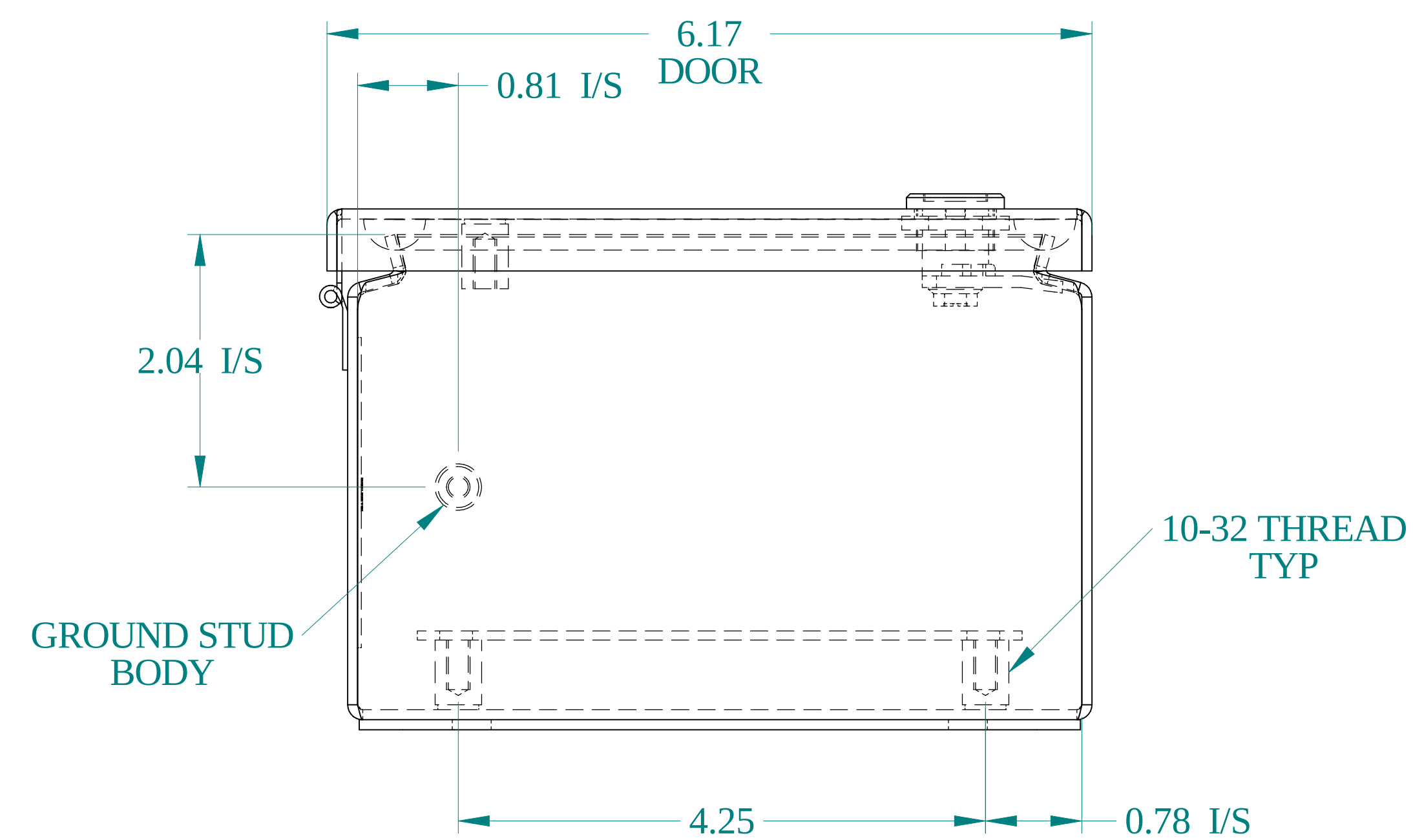
BOTTOM VIEW
