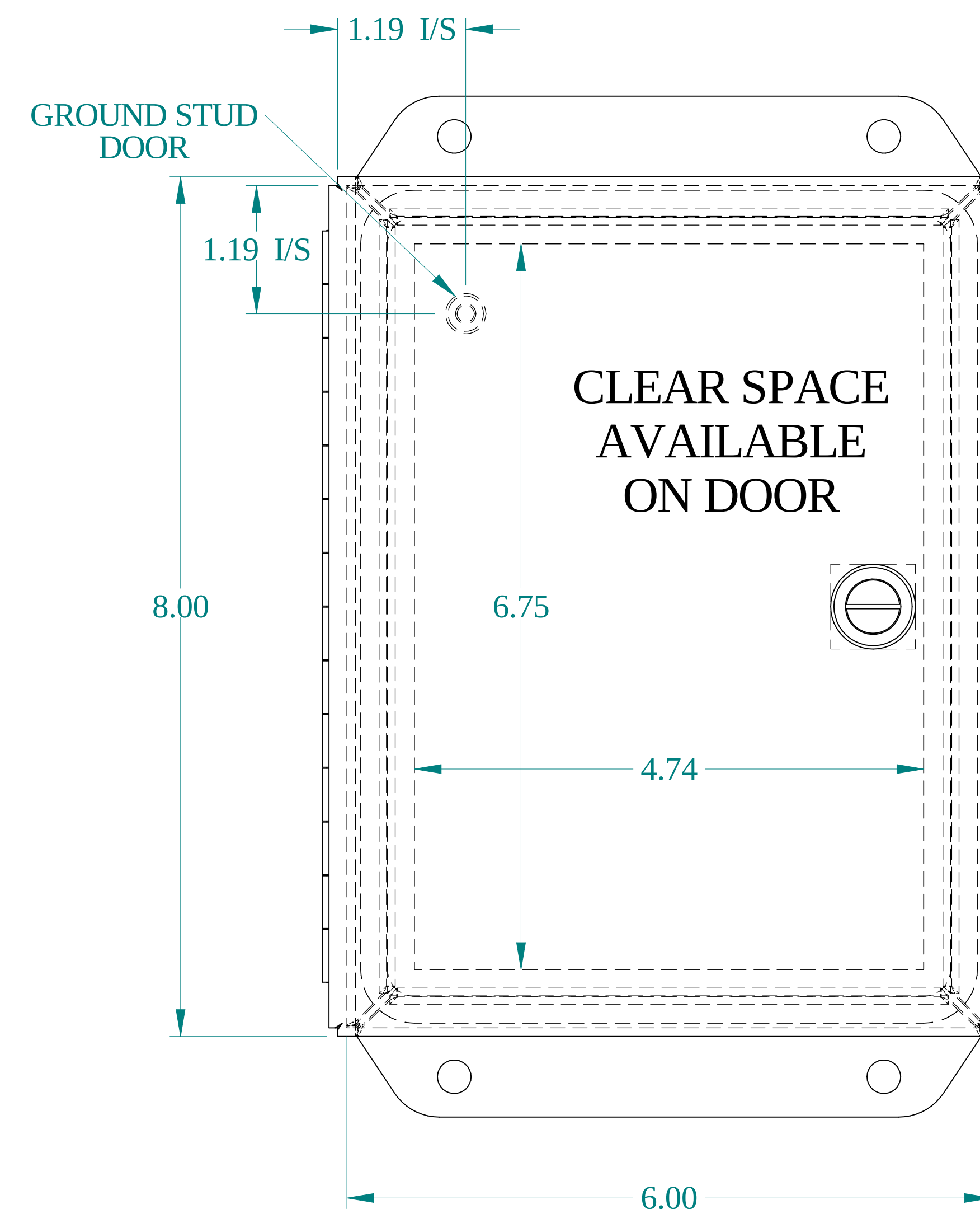
FRONT VIEW
