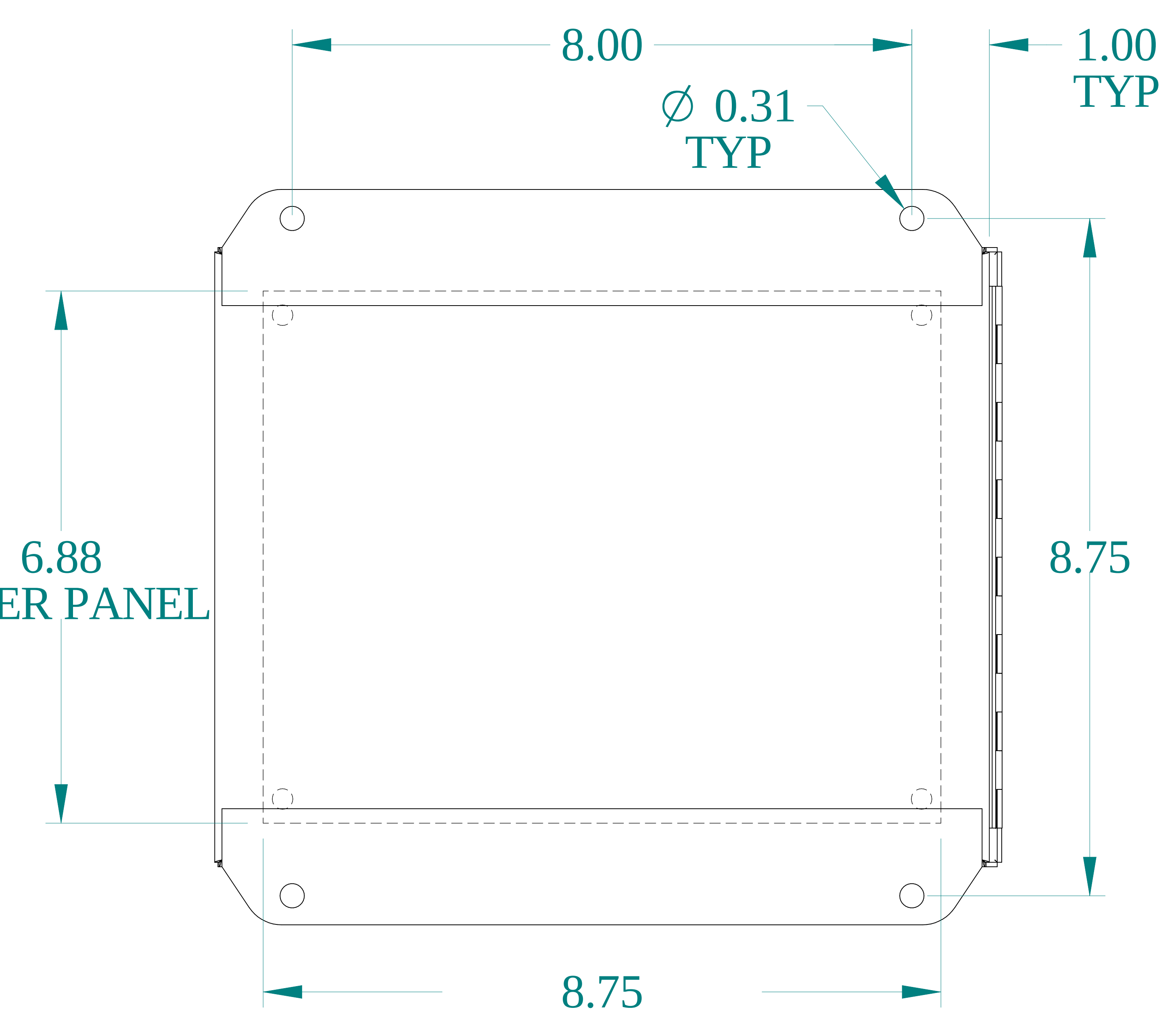
BACK VIEW
