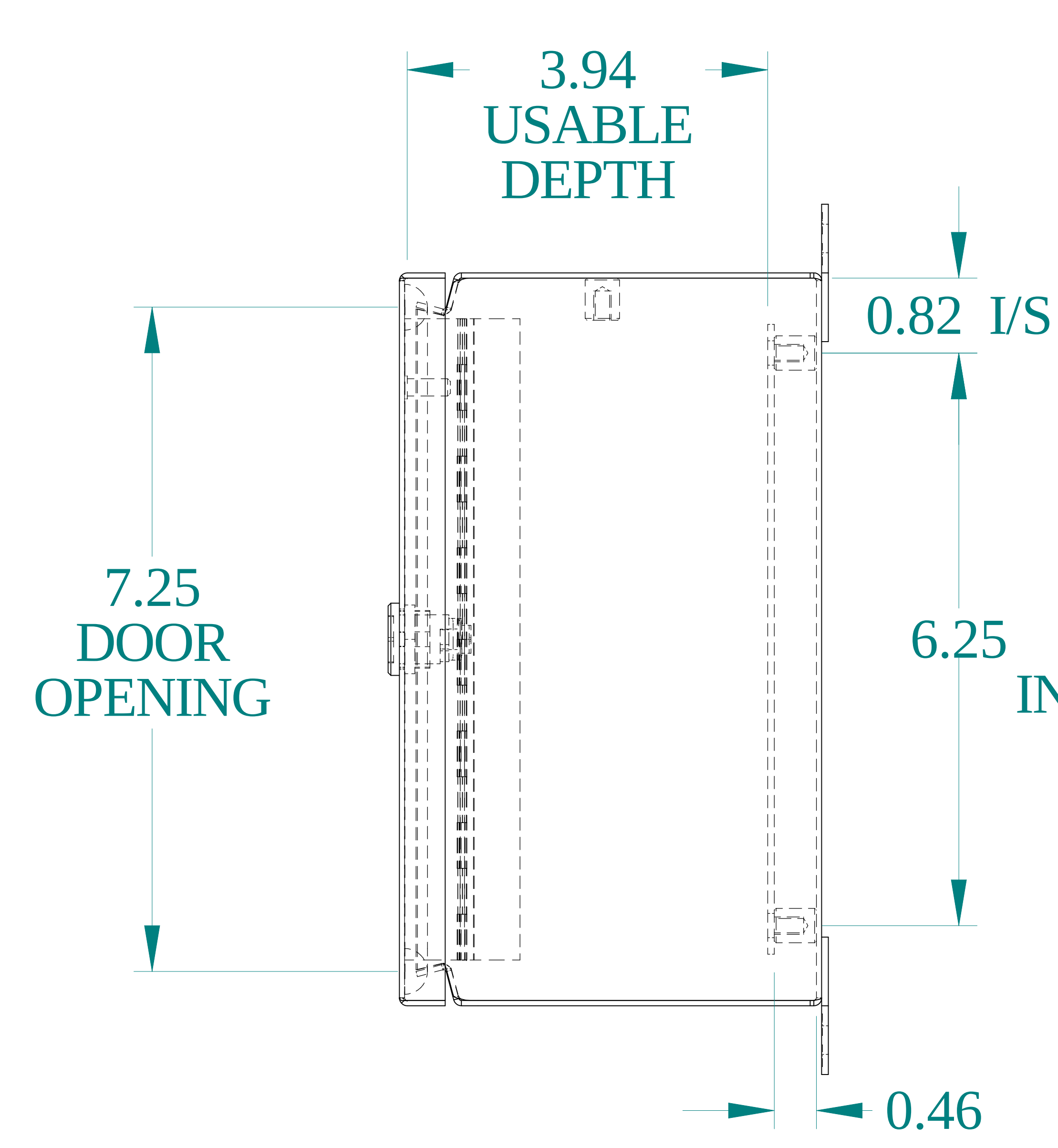
SIDE VIEW
