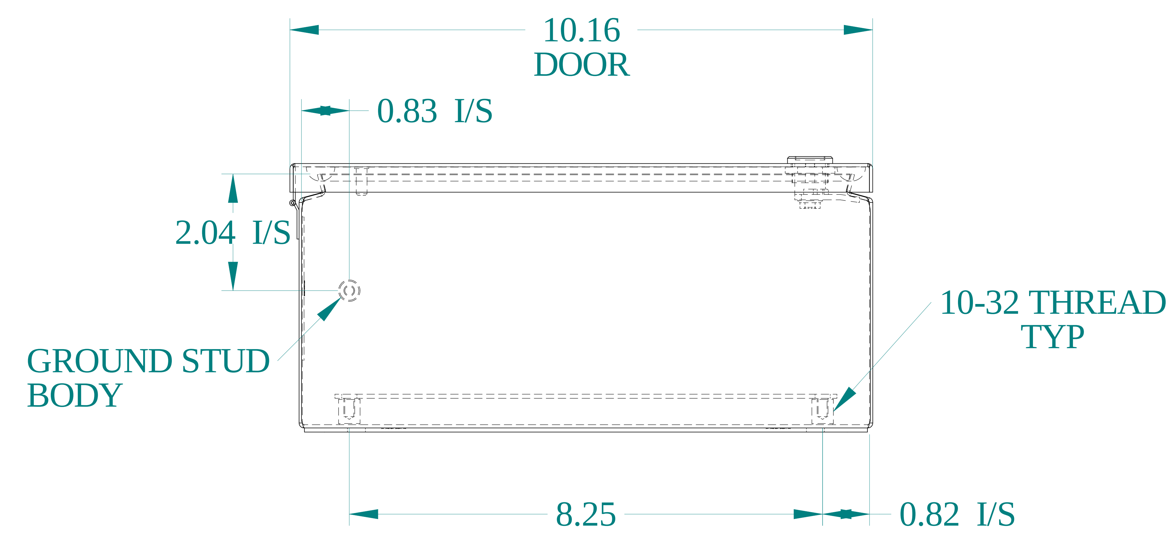
BOTTOM VIEW
