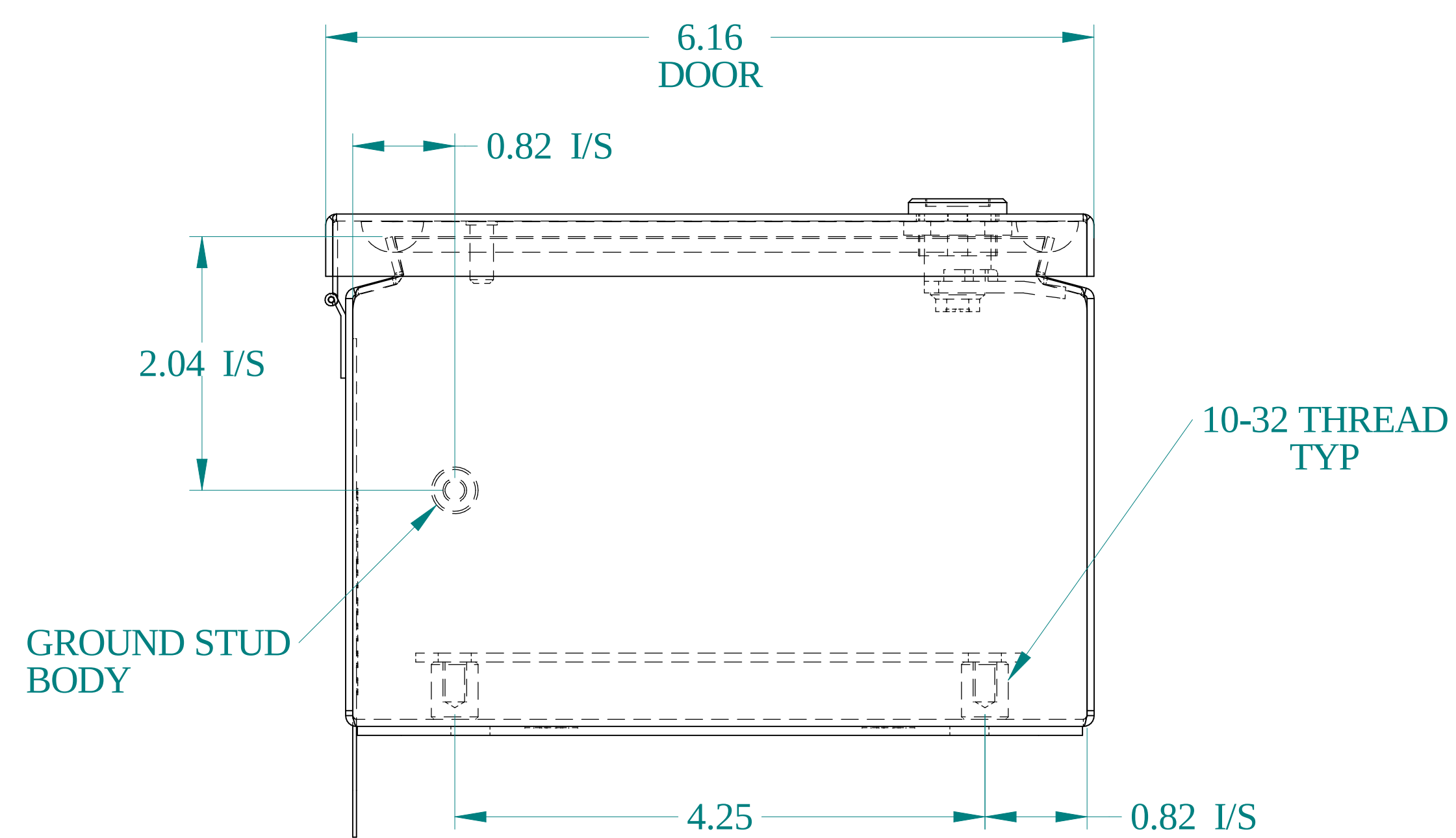
BOTTOM VIEW
