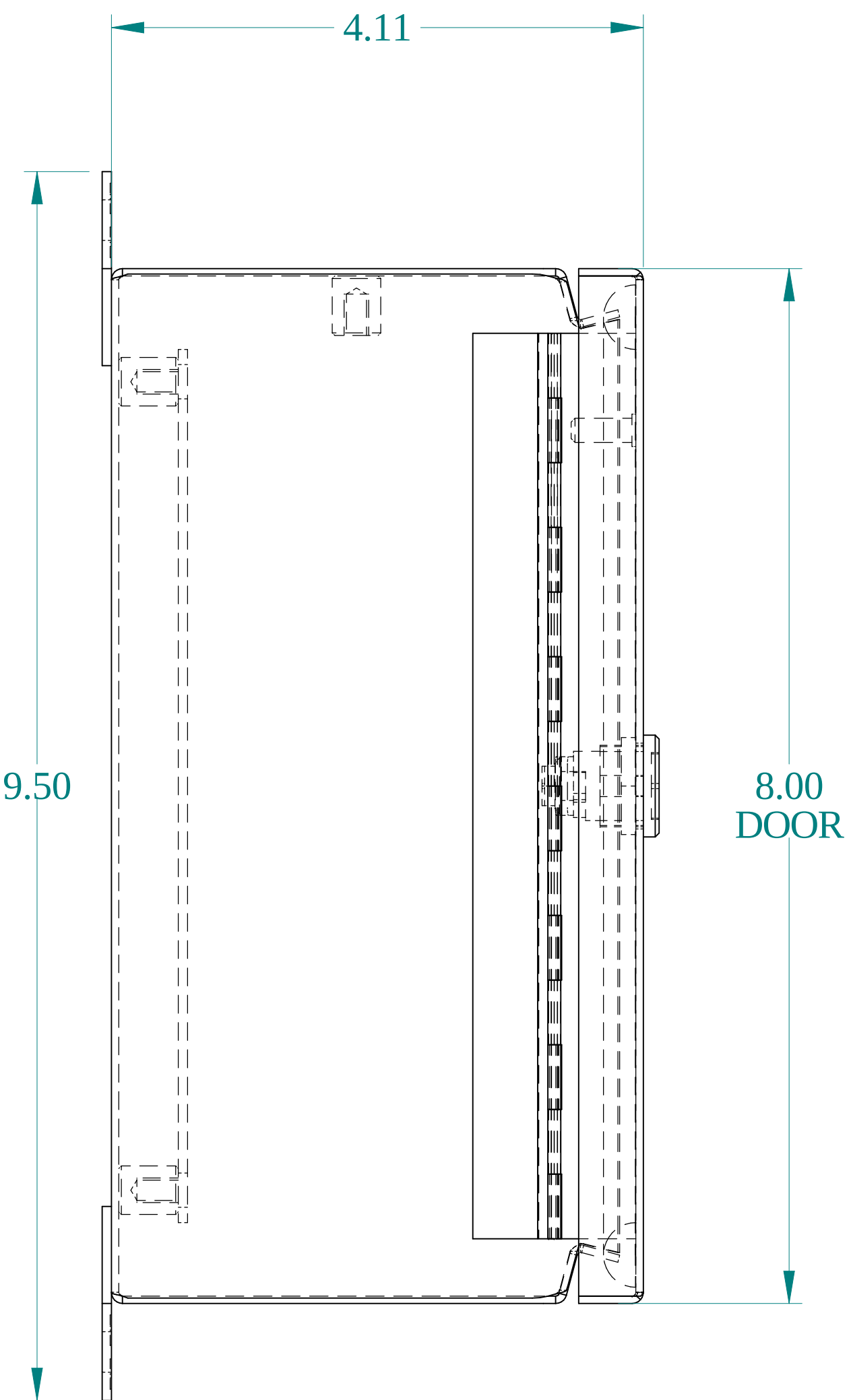
SIDE VIEW
