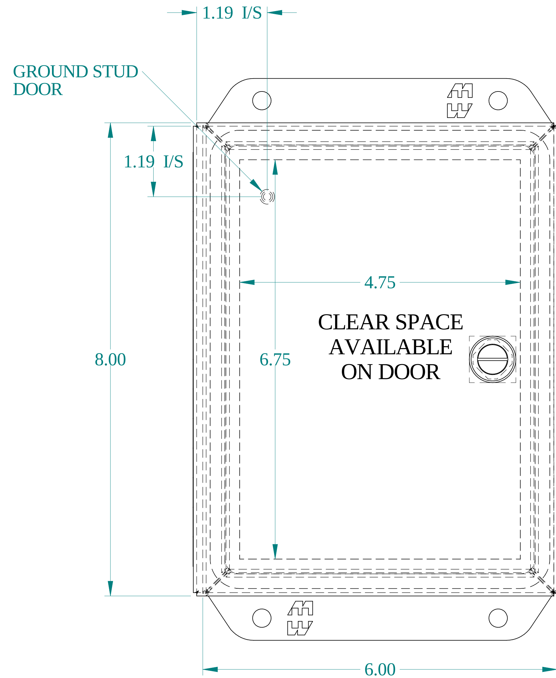
FRONT VIEW
