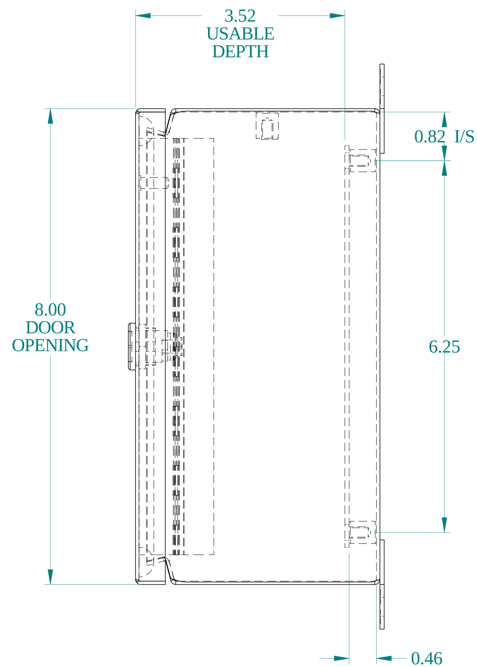
SIDE VIEW
