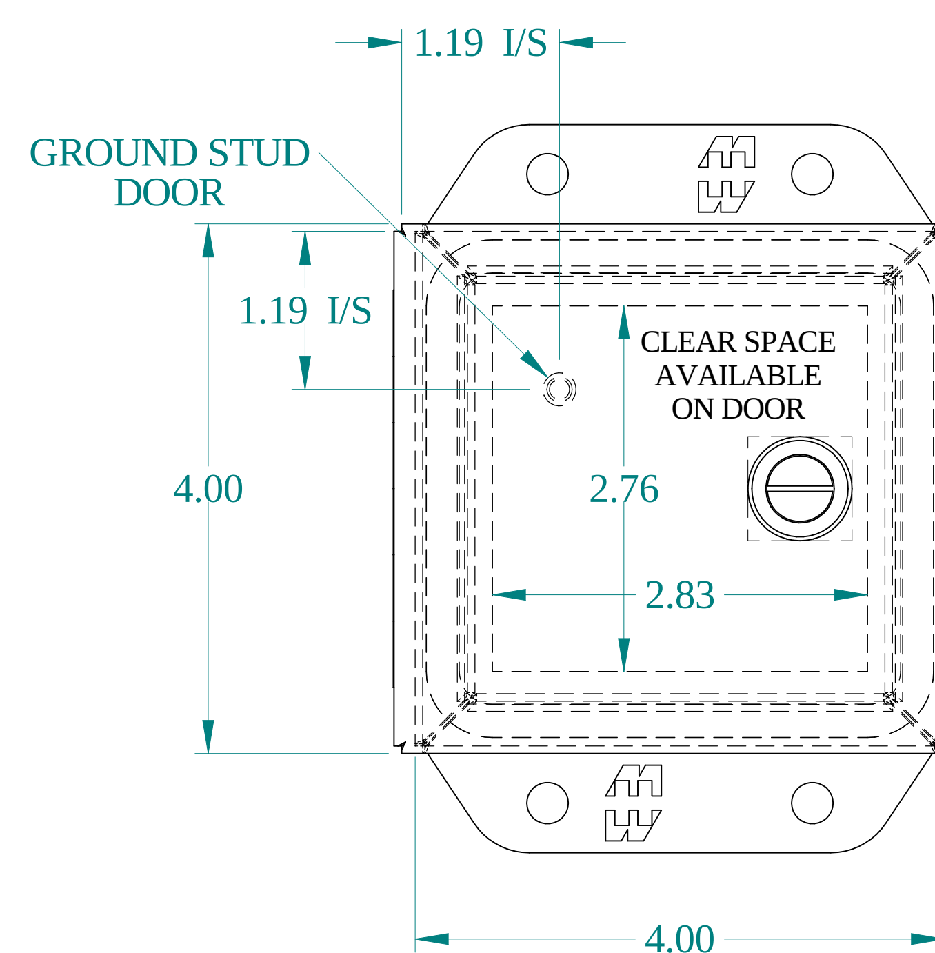
FRONT VIEW
