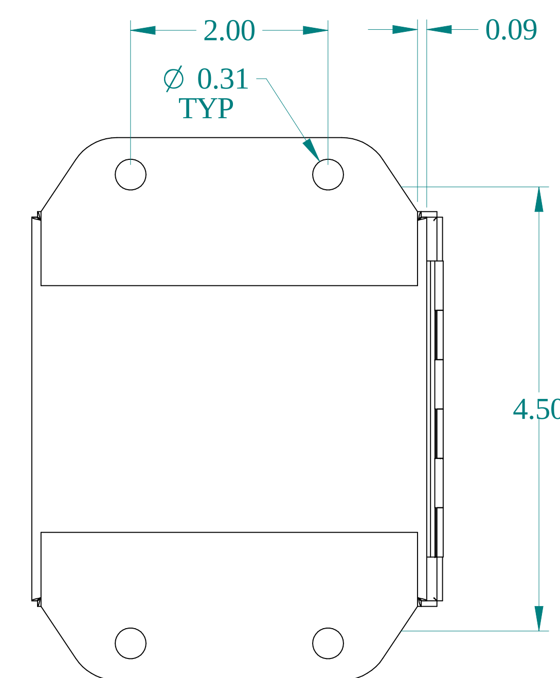
BACK VIEW
